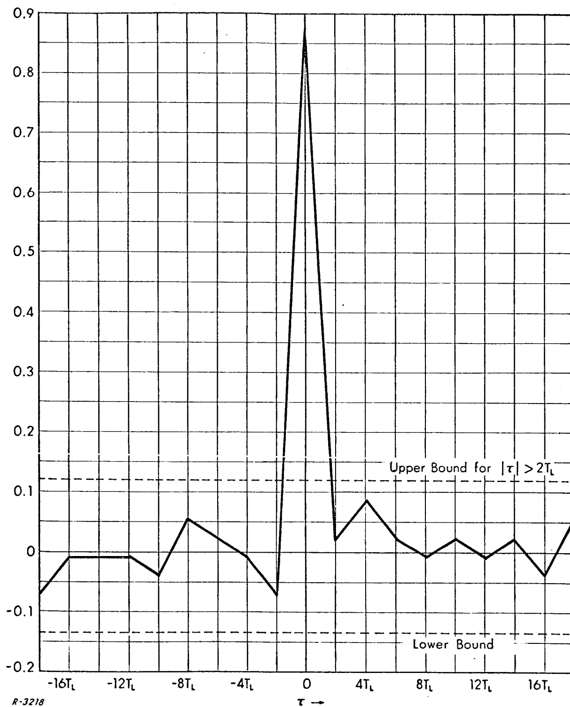
Fig. 4.2 A Cross-Correlation Function of L-Code and L⊕Data.
