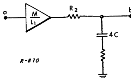
Fig. 3.9 Equivalent Circuit to Fig. 3.8.
