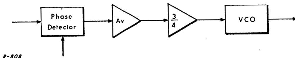
Fig. 3.7 DC Equivalent Circuit of Fig. 3.4.
