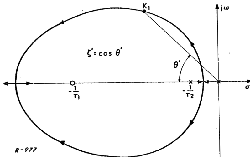
Fig. 3.13 Root Locus Plot of a Standard Second-Order Loop Containing the Filter F(s) = (1 + \tau_1 s) / (1 + \tau_2 s) .
