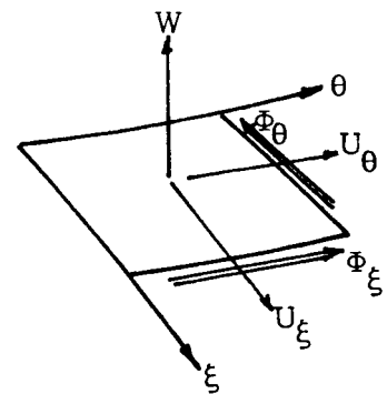
Figure 1.3 Displacements and Rotations
