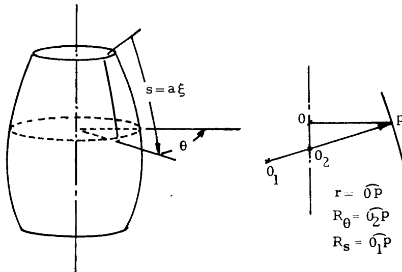
Figure 1.1 Surface Geometry and Coordinates
