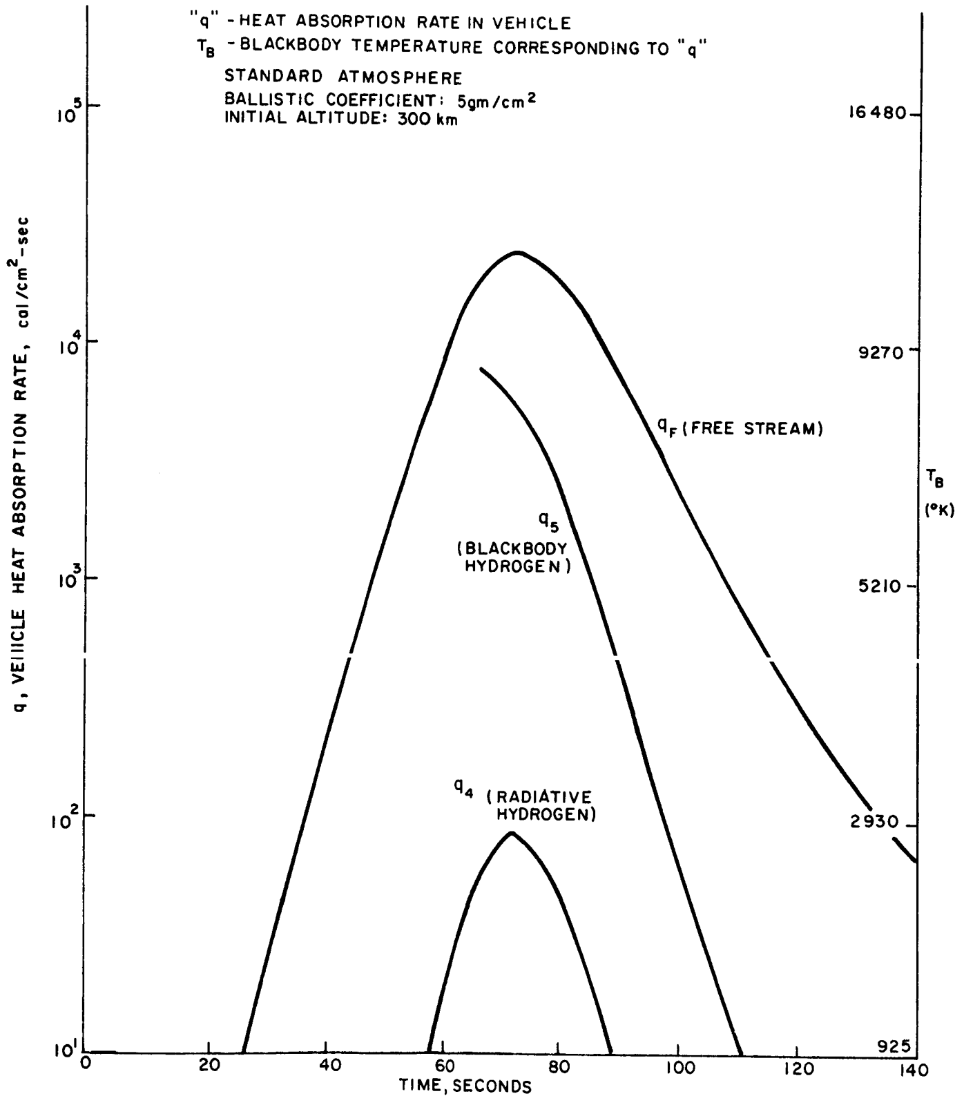
FIGURE 7. ESTIMATED RADIATIVE HEAT ABSORPTION RATES - JUPITER GRAZING ENTRY
