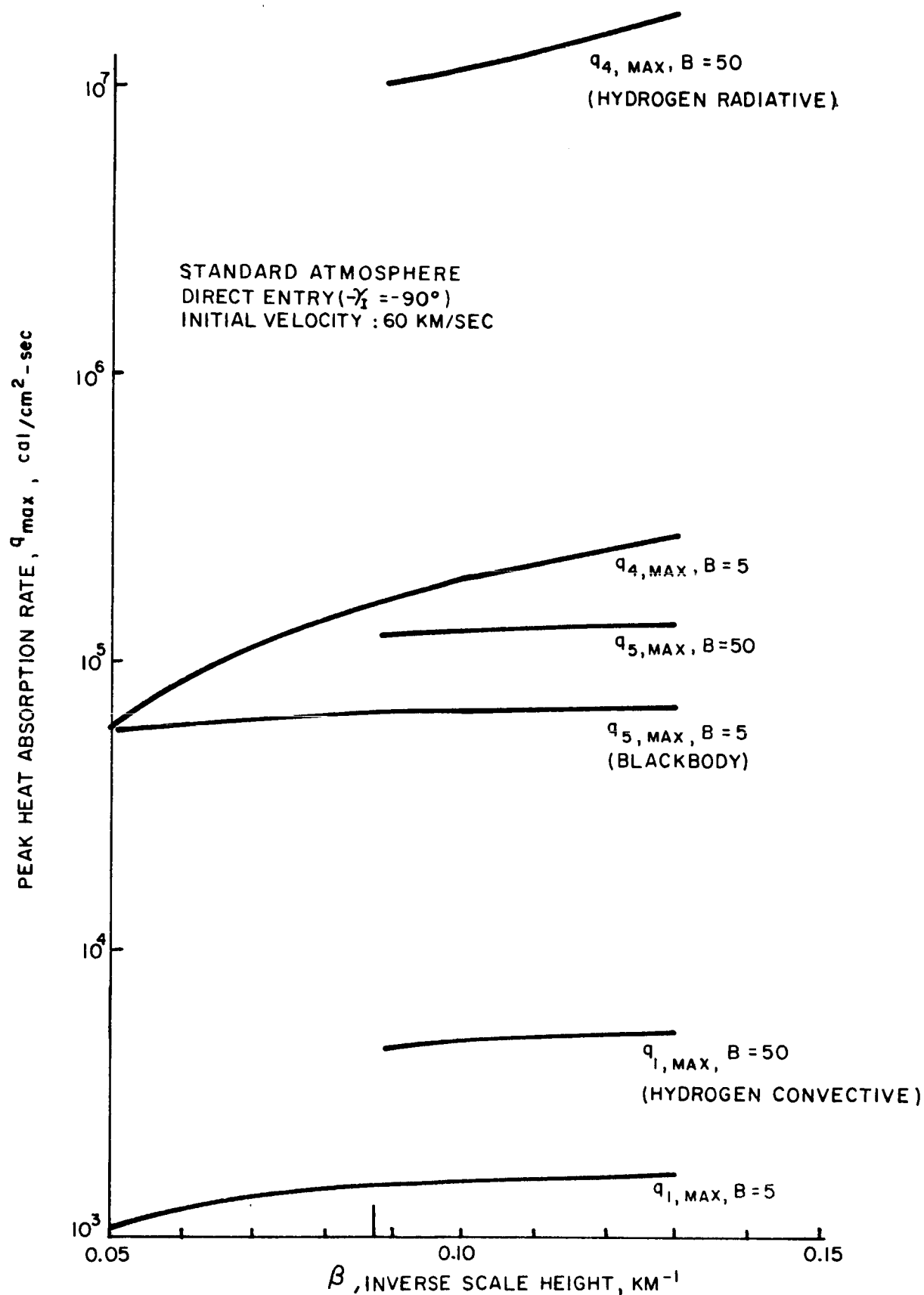
FIGURE 11. ENTRY HEAT ABSORPTION RATE MAXIMA VS. INVERSE SCALE HEIGHT
