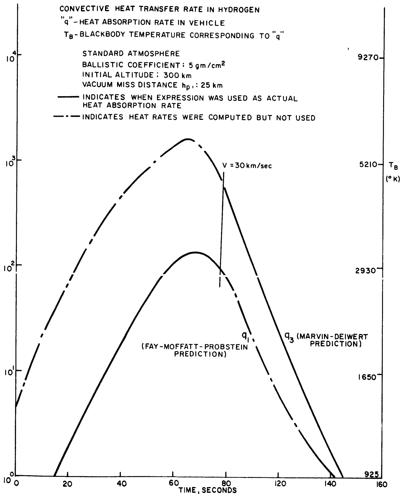
FIGURE 5. ESTIMATED CONVECTIVE HEAT ABSORPTION RATE - JUPITER GRAZING ENTRY
