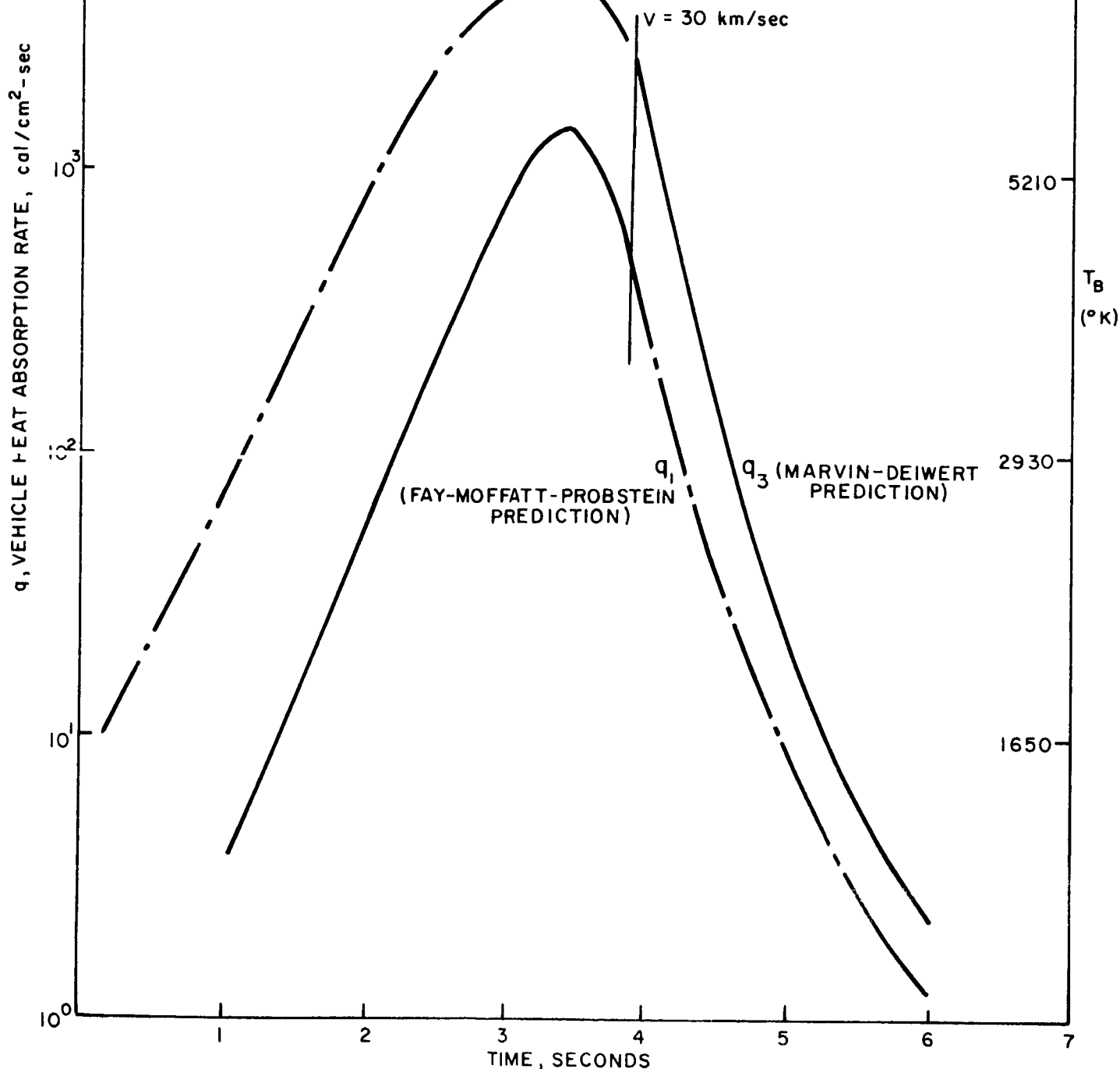
FIGURE 4. ESTIMATED CONVECTIVE HEAT ABSORPTION RATE - JUPITER DIRECT ENTRY
