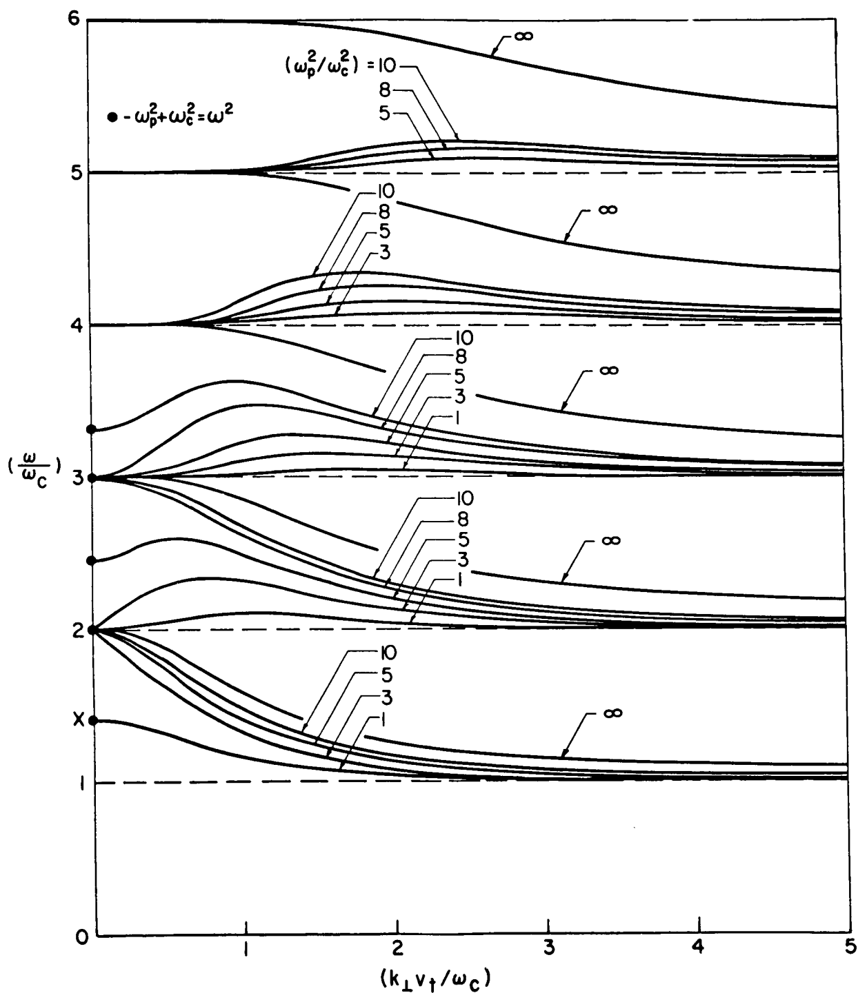
Fig. 10. DISPERSION CHARACTERISTICS OF PERPENDICULAR PROPAGATING CYCLOTRON HARMONIC WAVES FOR MAXWELLIAN DISTRIBUTION.
