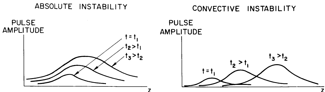
Fig. 13. SKETCHES ILLUSTRATING ABSOLUTE AND CONVECTIVE INSTABILITIES.
