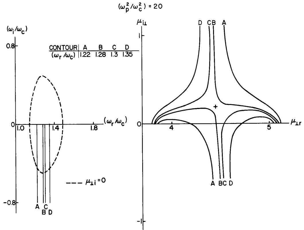
Fig. 17. CONFORMAL MAPPING OF CONTOURS A, B, C, AND D INTO COMPLEX \mu_{\perp} PLANE PROVING THAT INSTABILITIES OF RING DISTRIBUTION ARE ABSOLUTE.
