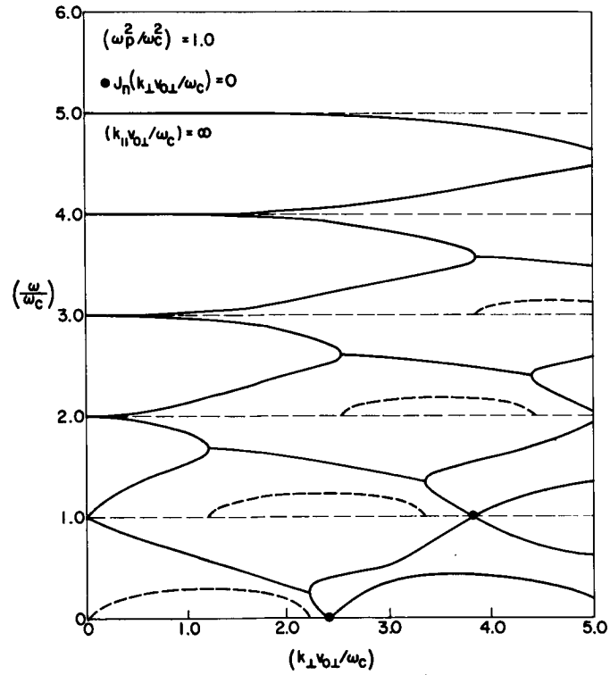
Fig. 24. RESONANT FREQUENCIES FOR OBLIQUELY PROPAGATING CYCLOTRON HARMONIC WAVES WITH k_{\parallel} CONSTANT; RING DISTRIBUTION FOR (a) (\omega_p^2/\omega_c^2) = 0.25 , AND (b) (\omega_p^2/\omega_c^2) = 1 .
