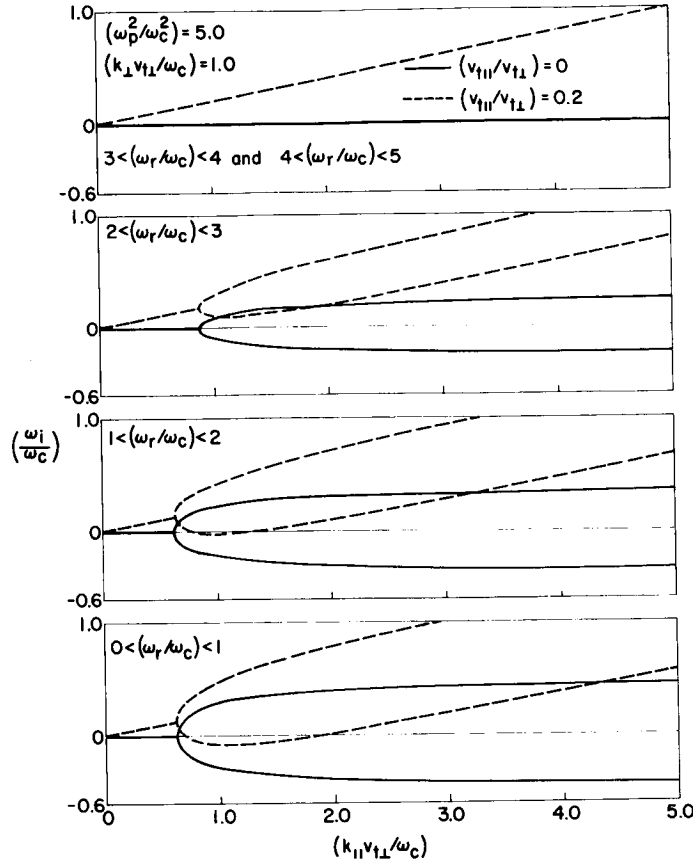
Fig. 31. IMAGINARY PART OF \omega FOR OBLIQUE PROPAGATION OF CYCLOTRON HARMONIC WAVES. Here the parallel component of the electron velocity v_{\parallel} is distributed according to a resonance function with effective thermal speed v_{t\parallel} , and the transverse components have a Maxwellian distribution with thermal speed v_{t\perp} .
