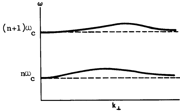
Fig. 5. TYPICAL DISPERSION CHARACTERISTICS OF CYCLOTRON HARMONIC WAVES PROPAGATING PERPENDICULAR TO THE MAGNETIC FIELD.
