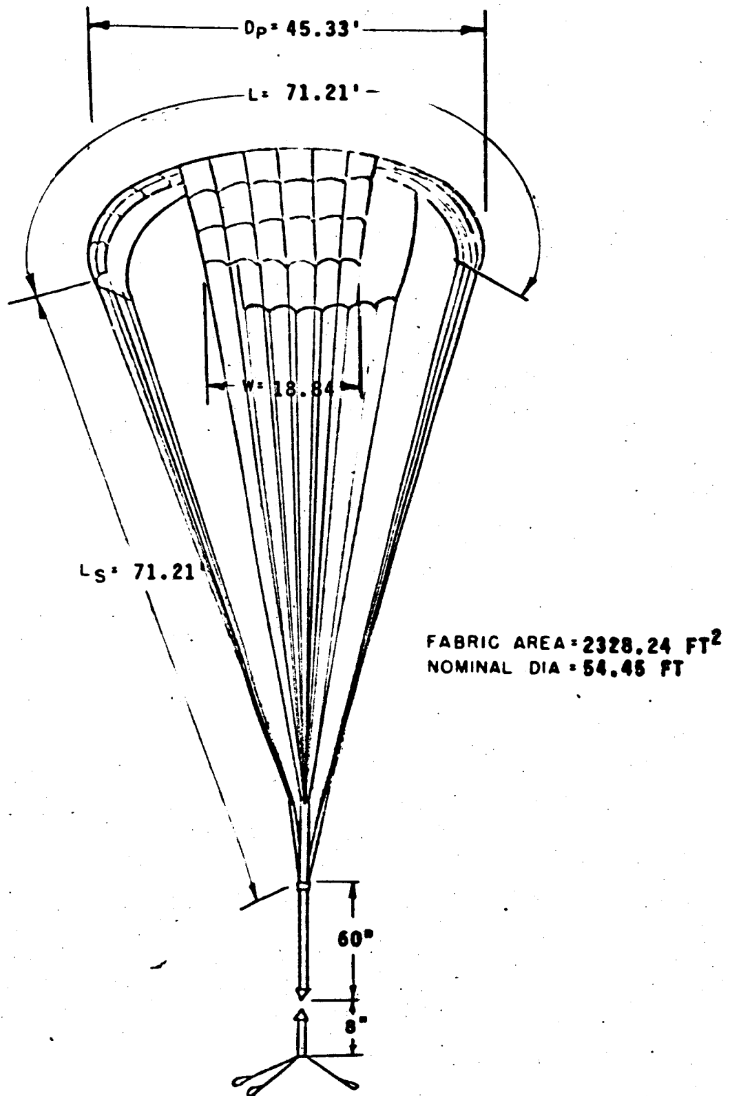
FIGURE 2 GENERAL DIMENSIONS
