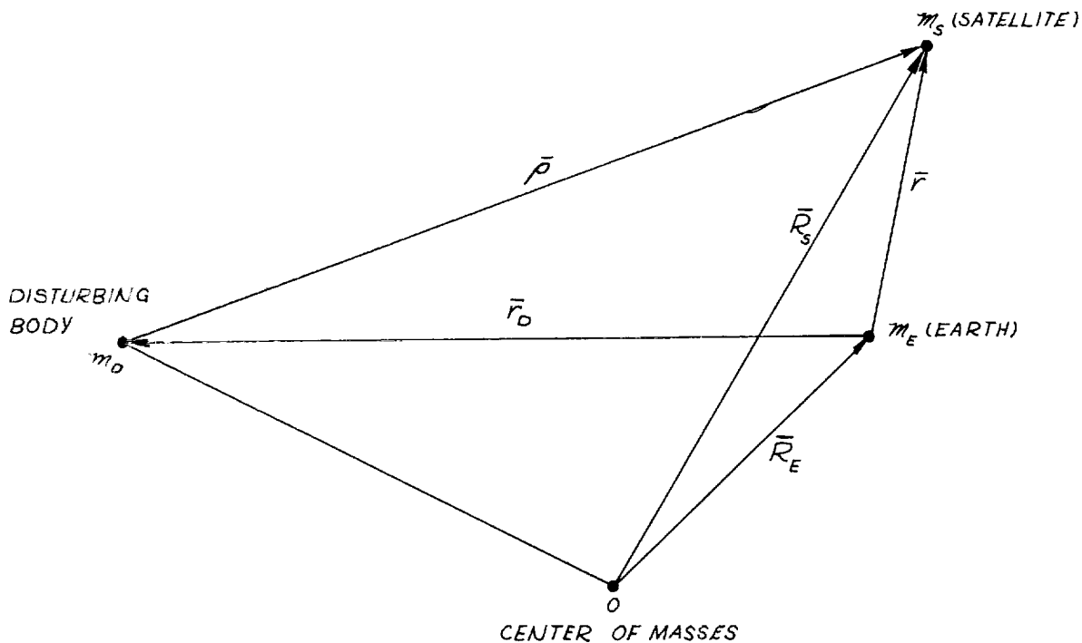
Figure 2. Geometry of the Three-Body Problem
