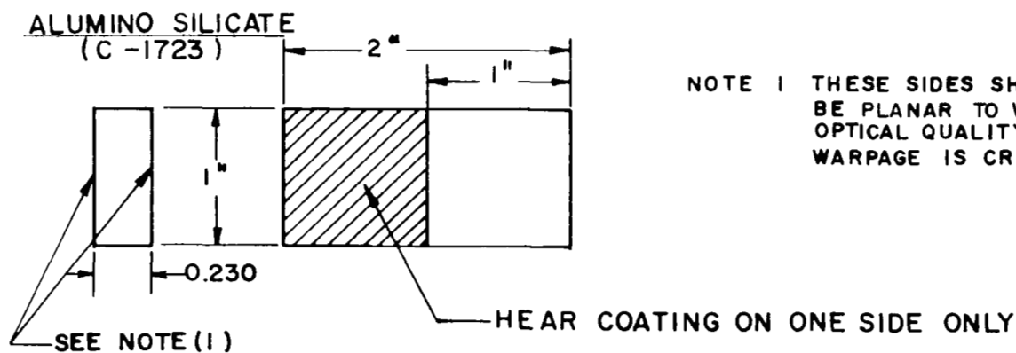
FIG. 2 : COATING ARRANGEMENT-WINDOW SAMPLES
