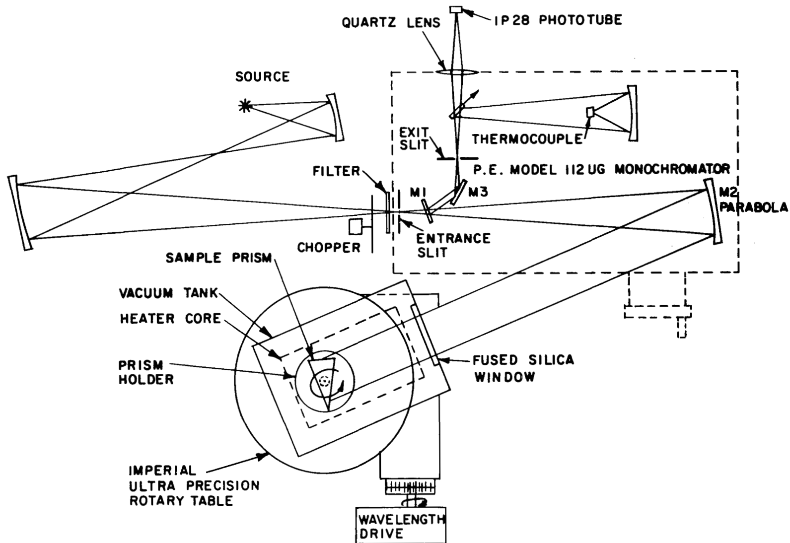
FIG. 15 : MODIFIED PERKIN ELMER 112 UG MONOCHROMATOR AND ROTARY TABLE FOR REFRACTIVE INDEX MEASUREMENTS
