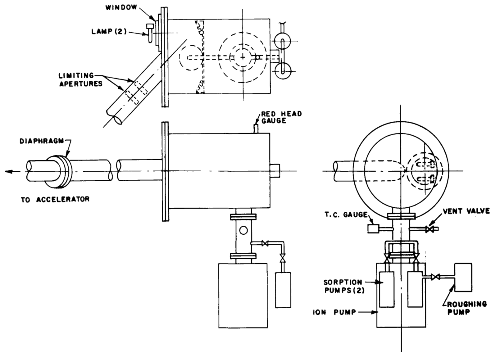
FIG. 13: PUMPING ARRANGEMENT
