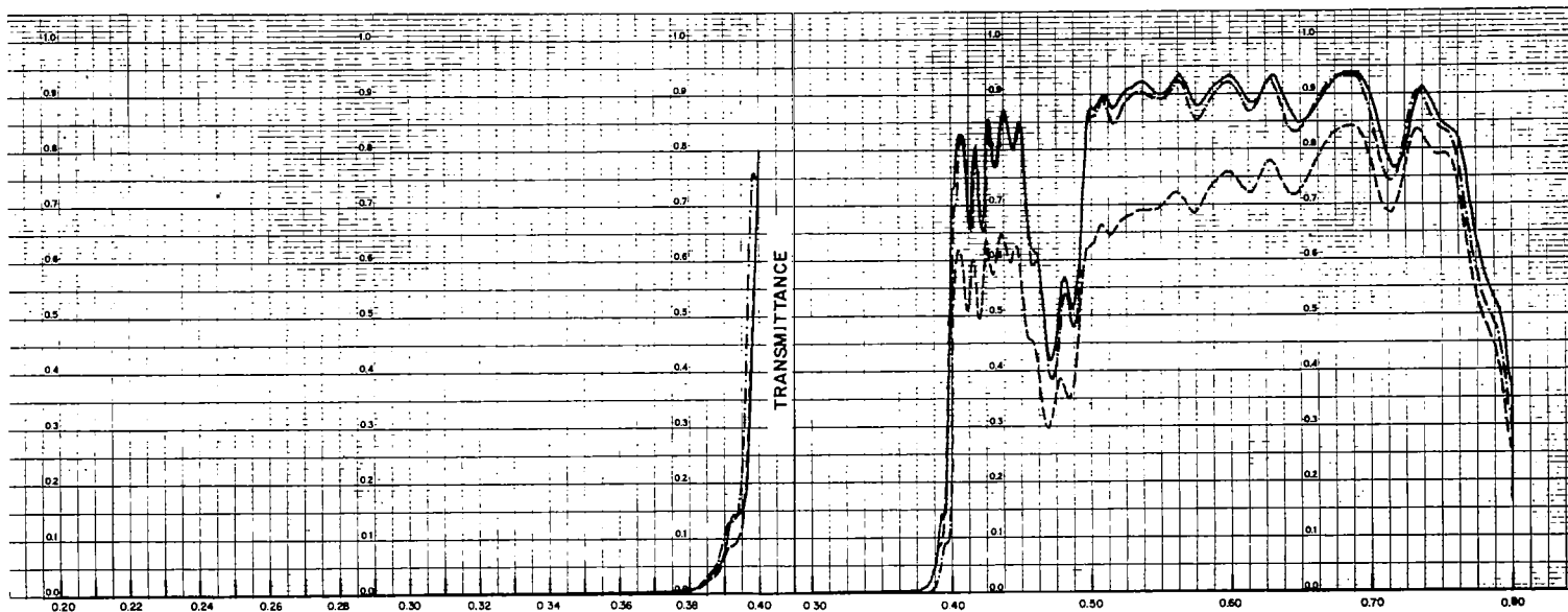
VYCOR-CORNING CODE 7913—EFFECT OF IRRADIATION ON TRANSMITTANCE AT 26°C, WBHM COATING, SAMPLE THICKNESS 0.378 CM
