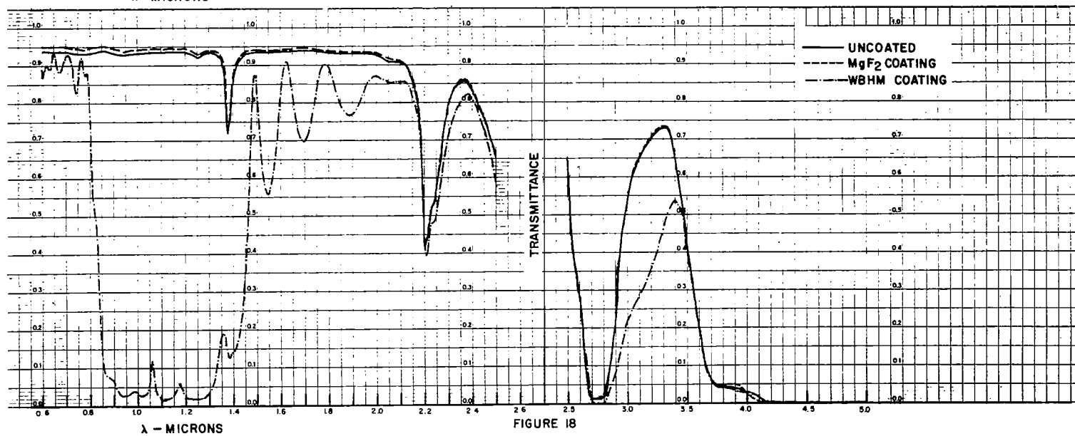
FUSED SILICA-CORNING CODE 7940, U.V. GRADE - TRANSMITTANCE AT 26°C, SAMPLE THICKNESS 1.784 CM
