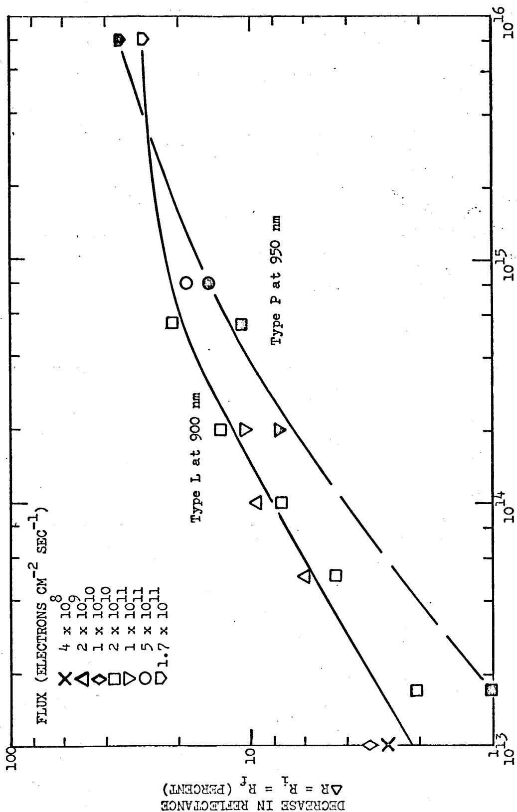
Figure 4. Electron Rate Study in \text{TiO}_2 -Methyl Silicone Coatings
