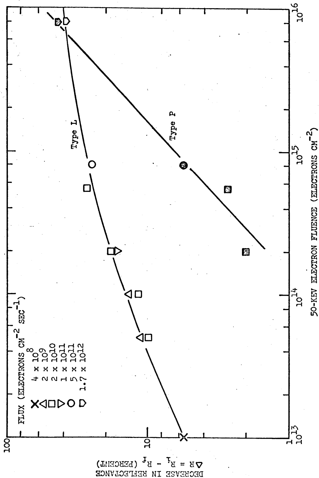
Figure 2. Electron Rate Study in TiO 2 -Methyl Silicone Coatings at 2100 nm.
