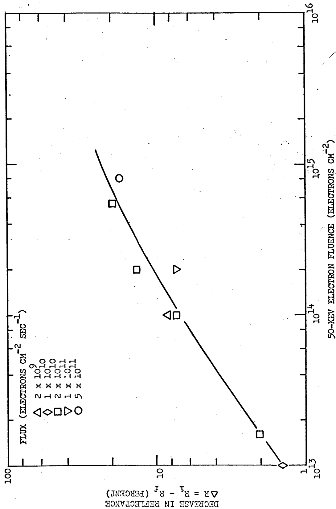
Figure 6. Electron Rate Study in Type L \text{TiO}_2 -Methyl Silicone at 590 nm.
