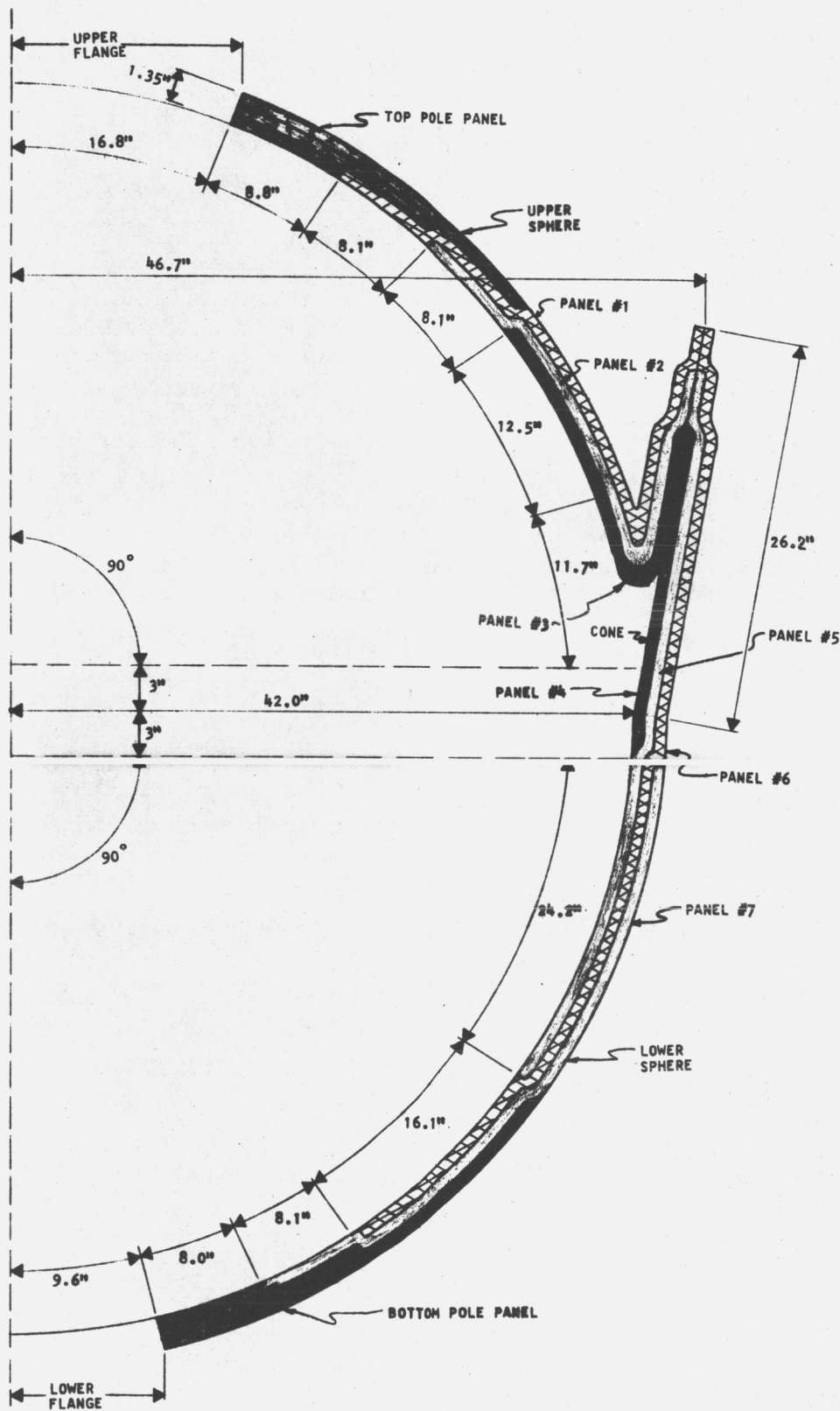
TITLE FIGURE *A-1 ARRANGEMENT OF INSULATION LAYERS FOR ENTIRE SYSTEM IN r-\theta PLANE
