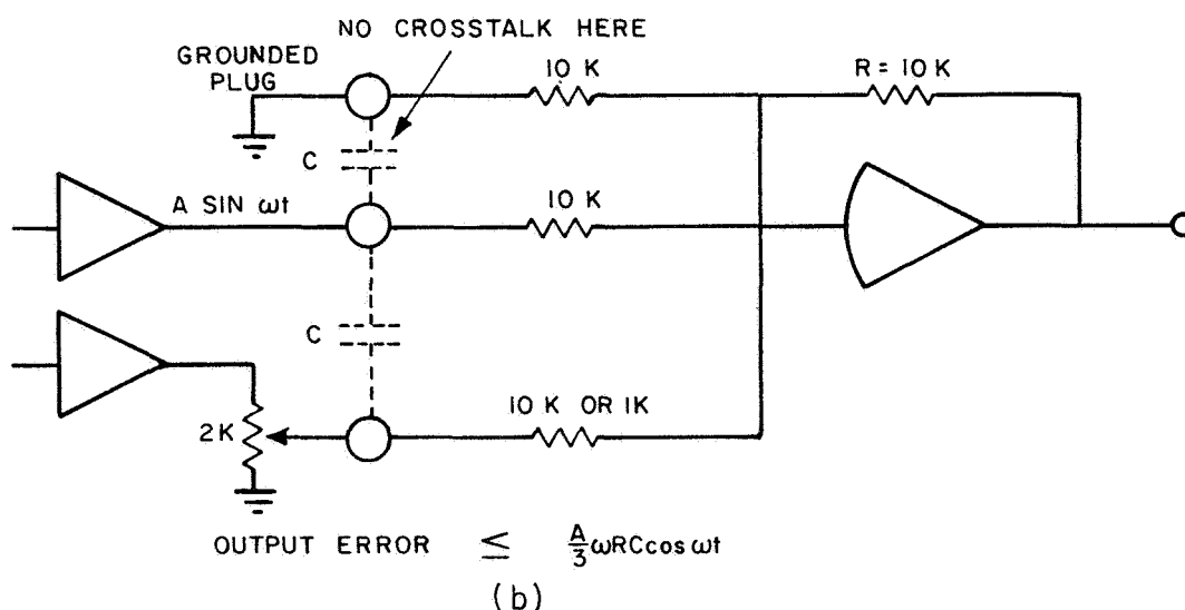
Fig. 3.3 Patchbay capacitances between inputs cause gain errors.
