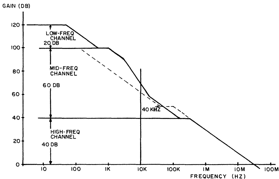
Fig. 4.1 (a) Block diagram showing signal flow through the three channels. (b) Open-loop Bode plot of the three channels and their combination.
