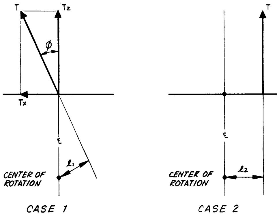
Fig. 10. Two types of thrust misalignment.
