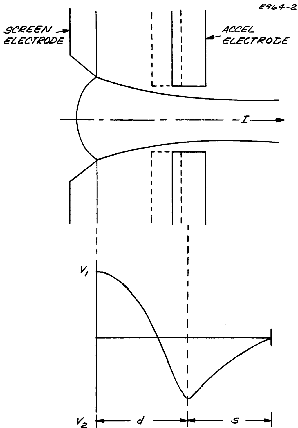
Fig. 4. Ion gun showing accel perturbation and idealized potential profile of planar gun.
