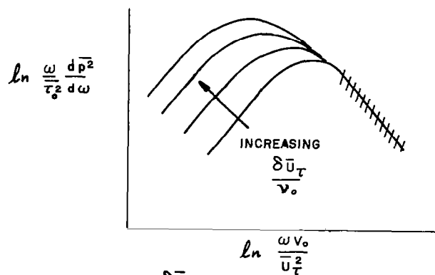
FIGURE 35 a. EFFECT OF \frac{\delta \bar{u}_\tau}{v_\infty} ON LOW FREQUENCY PLOT
