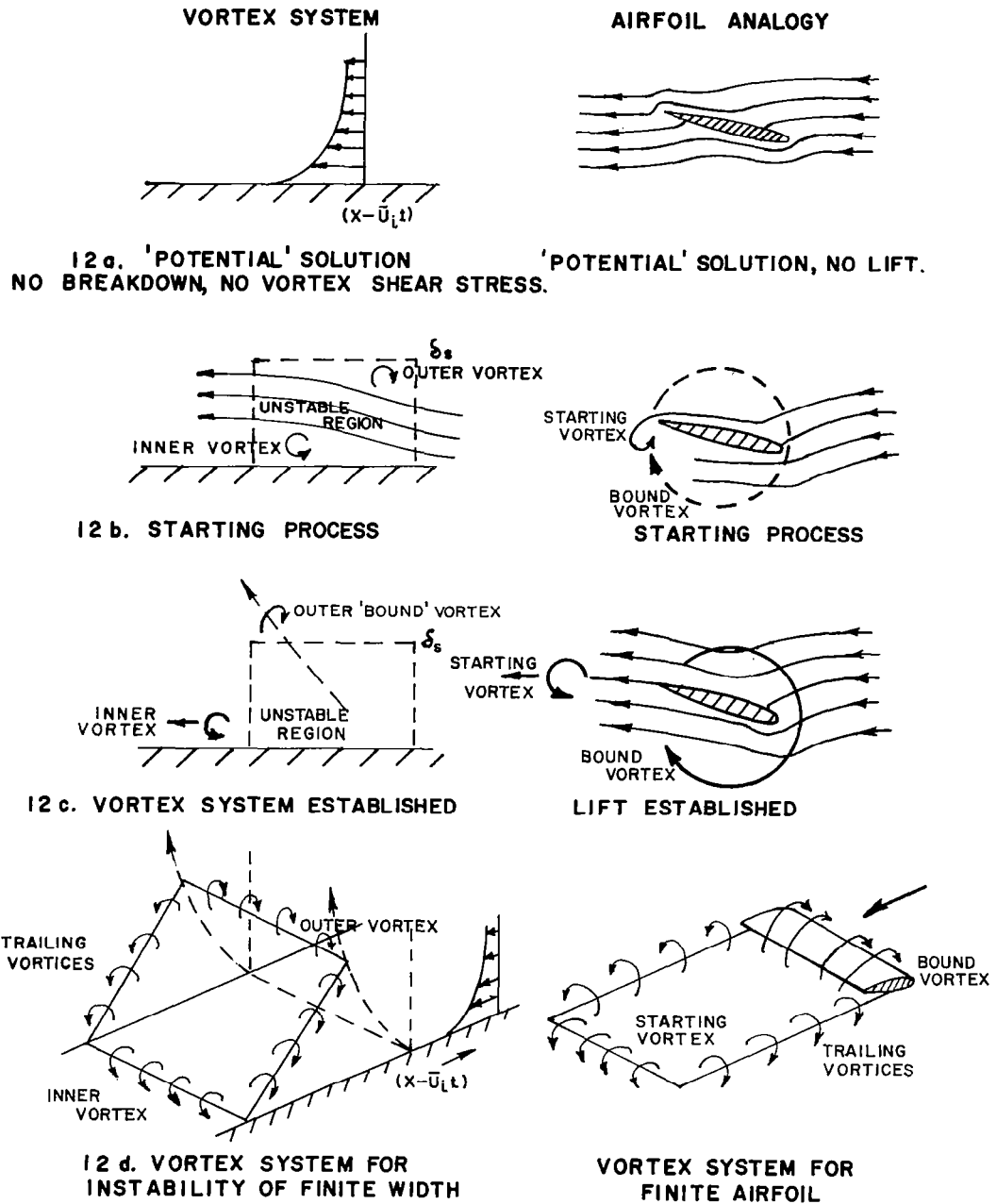
FIGURE 12 LIFT AIRFOIL ANALOGY
