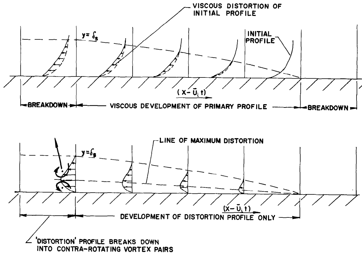
FIGURE 5. VORTEX-PAIR GENERATION EXPLAINED BY BREAKDOWN OF VISCOUS 'DISTORTION' PROFILE
