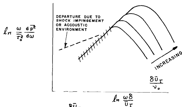
FIGURE 35 b. EFFECT OF \frac{\delta \bar{u}_\tau}{v_\infty} ON HIGH FREQUENCY PLOT
