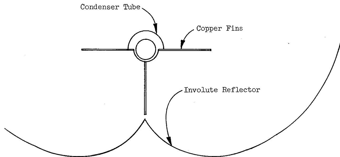
Fig. 9. Section through a finned tube fitted with an involute reflector for installation in a cylindrical drum-shaped radiator.
