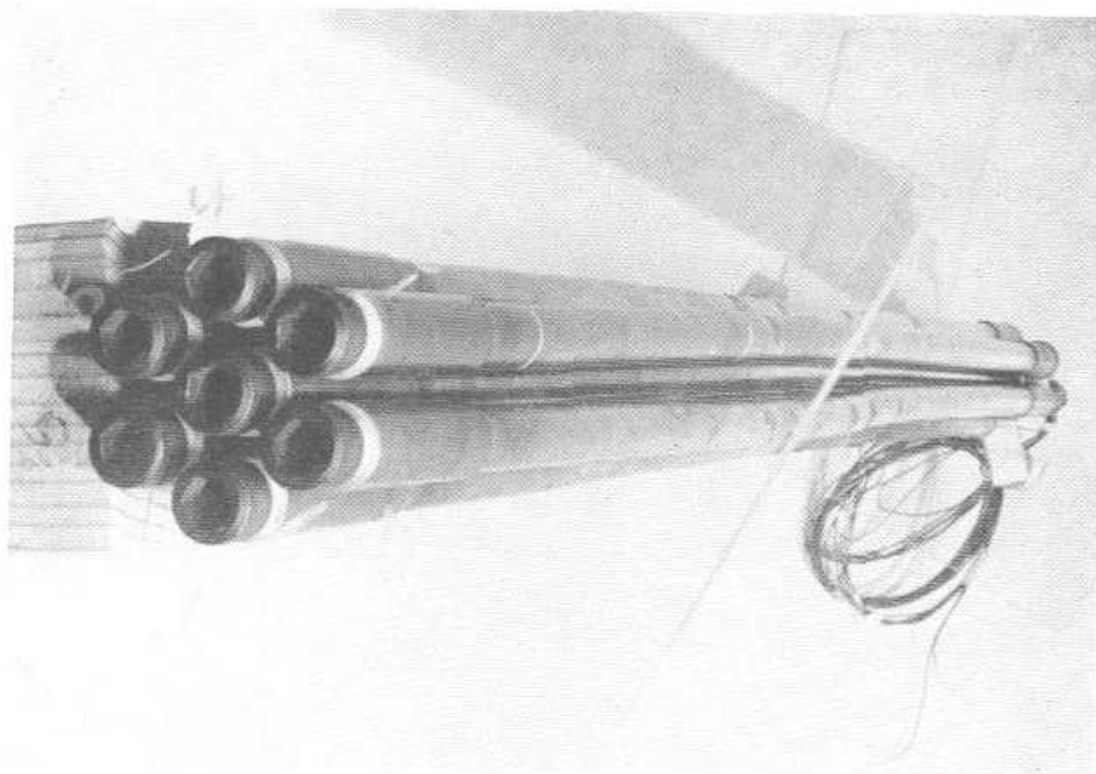
Fig. 4. An electrically heated mock-up of a prototype fuel-element for the EGR. Note that the rods have been warped by hot spots.
