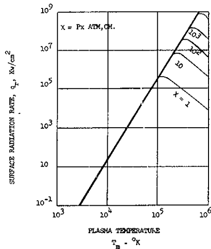
Fig. 4. Thermal radiation from uranium plasma Ref. (7).
