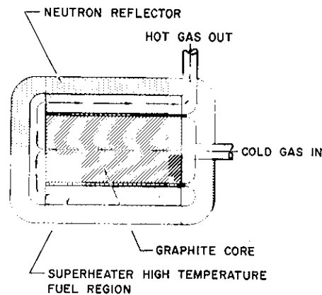
Fig. 6. Superheater reactor schematic outline.
