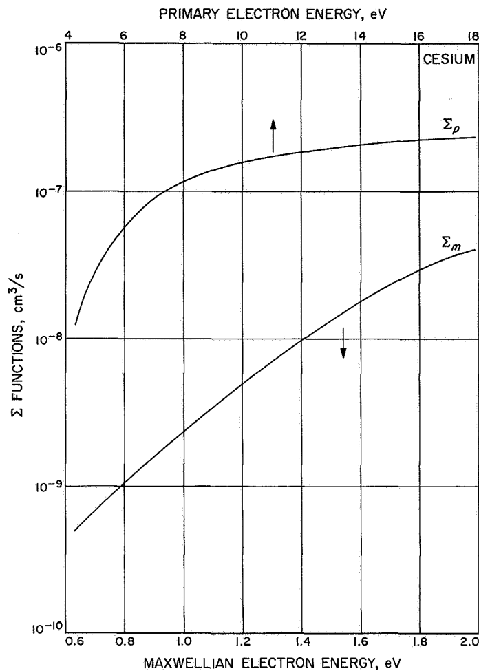
Fig. 13. Ion production coefficients for primary and Maxwellian electrons in cesium
