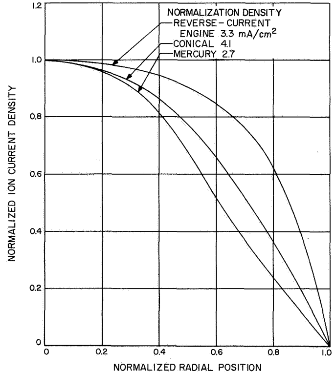
Fig. 32. Typical normalized beam current density distributions for three engines
