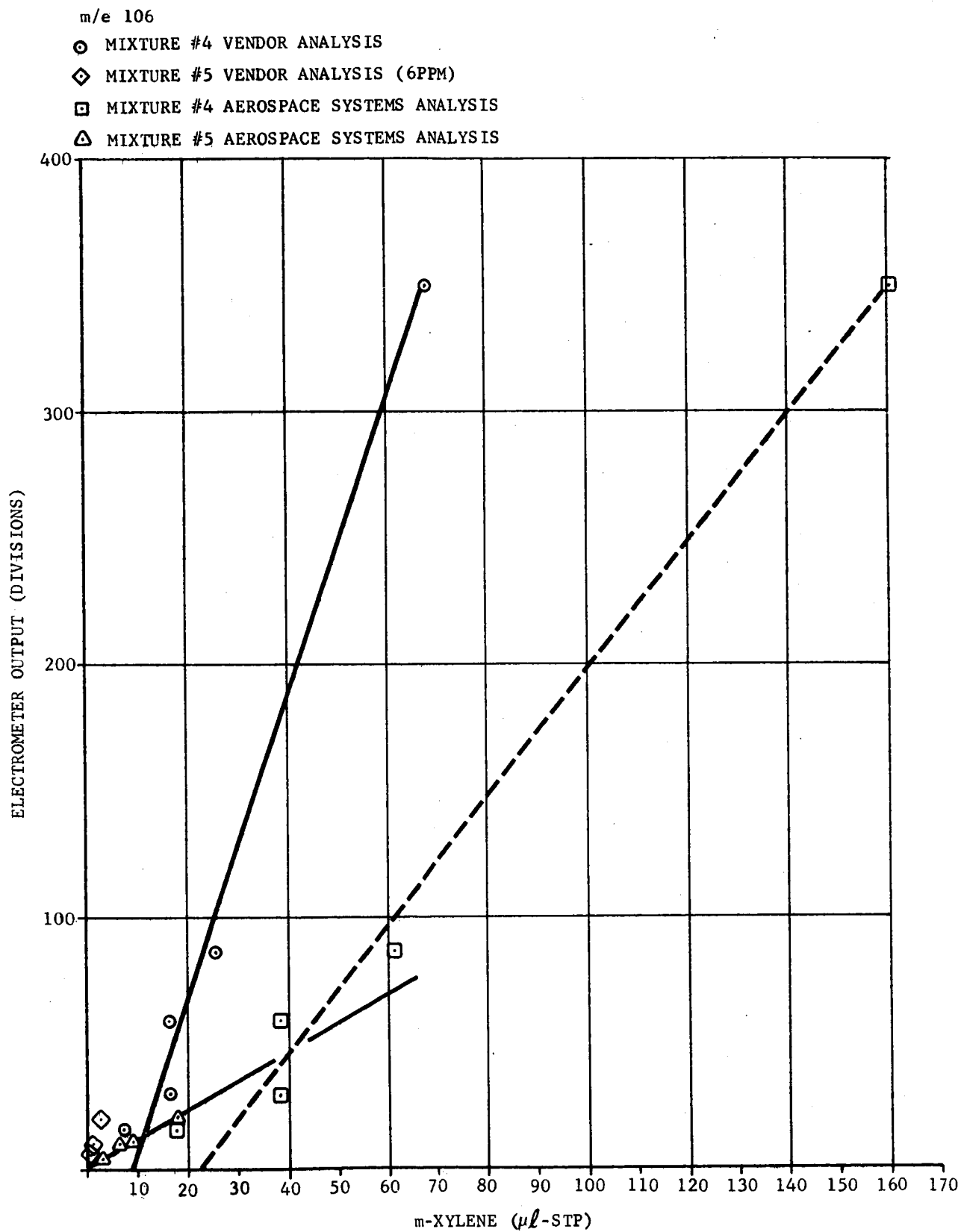
FIGURE 4-24 OUTPUT VS. AMOUNT SORBED M-XYLENE ON PORAPAK Q
