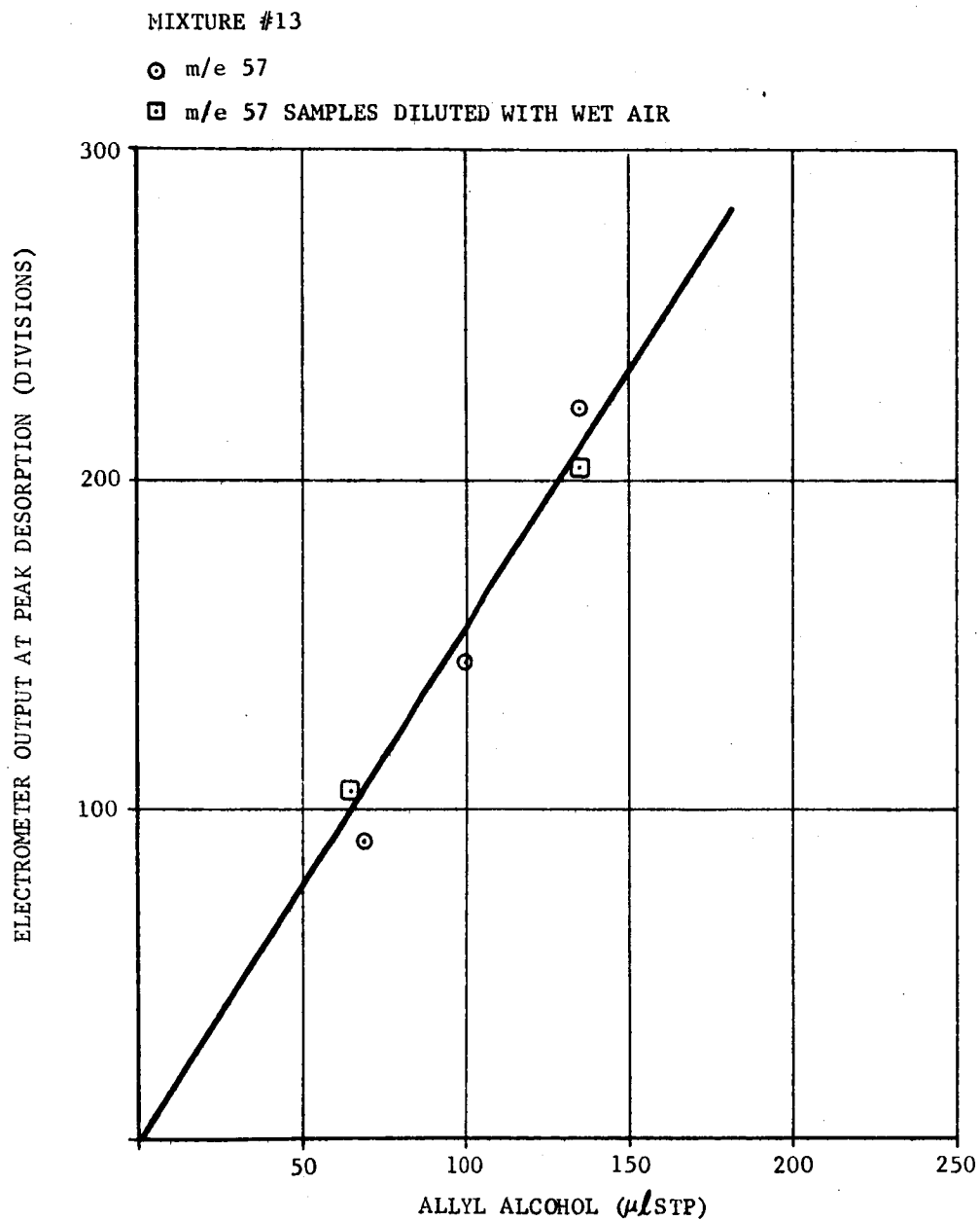
FIGURE 4-8 OUTPUT VS. AMOUNT SORBED ALLYL ALCOHOL ON PORAPAK Q
