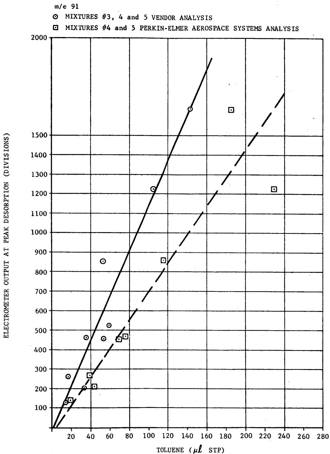
FIGURE 4-22 OUTPUT VS. AMOUNT SORBED TOLUENE ON PORAPAK Q
