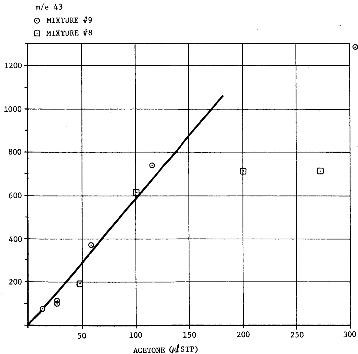
FIGURE 4-6 OUTPUT VS. AMOUNT SORBED ACETONE ON PORAPAK Q
