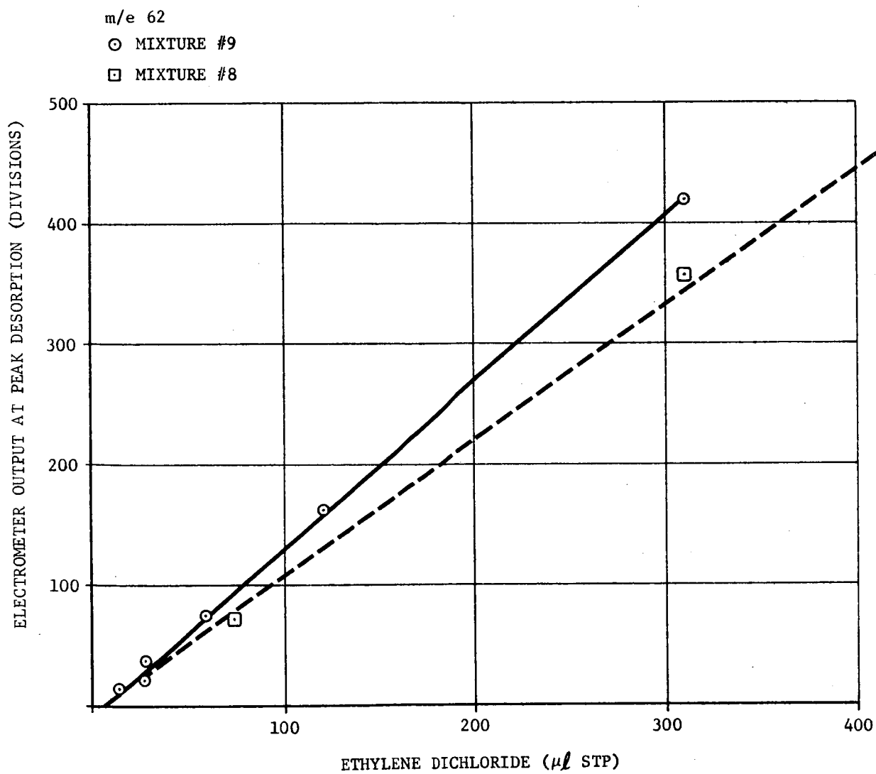
FIGURE 4-15 OUTPUT VS. AMOUNT SORBED ETHYLENE DICHLORIDE ON PORAPAK Q
