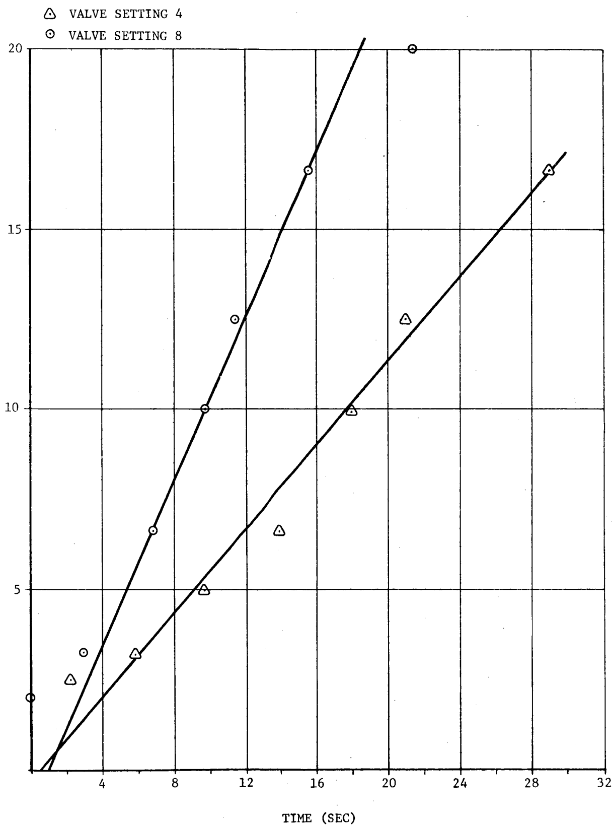
FIGURE 2-5A PUMPOUT RATE THROUGH MICROMETER NEEDLE VALVE
