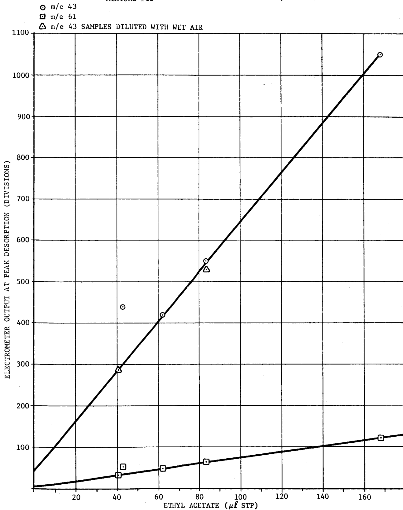
FIGURE 4-14 OUTPUT VS. AMOUNT SORBED ETHYL ACETATE ON PORAPAK Q
