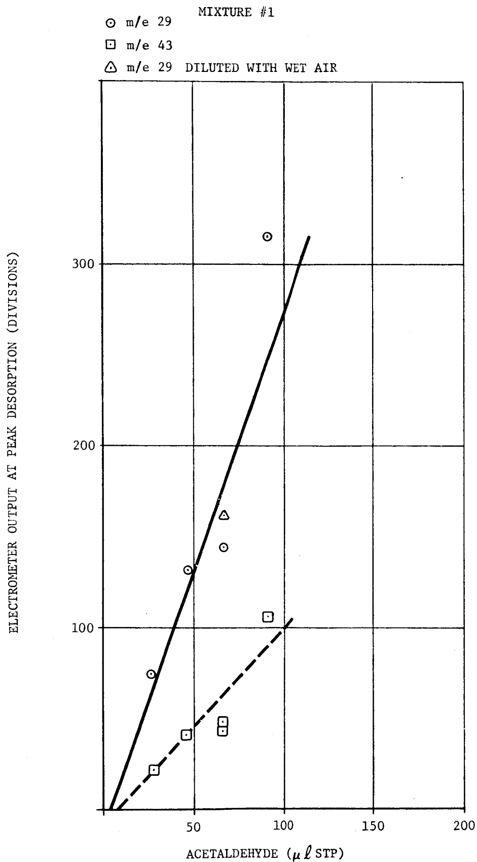
FIGURE 4-7 OUTPUT VS. AMOUNT SORBED ACETALDEHYDE ON CHARCOAL
