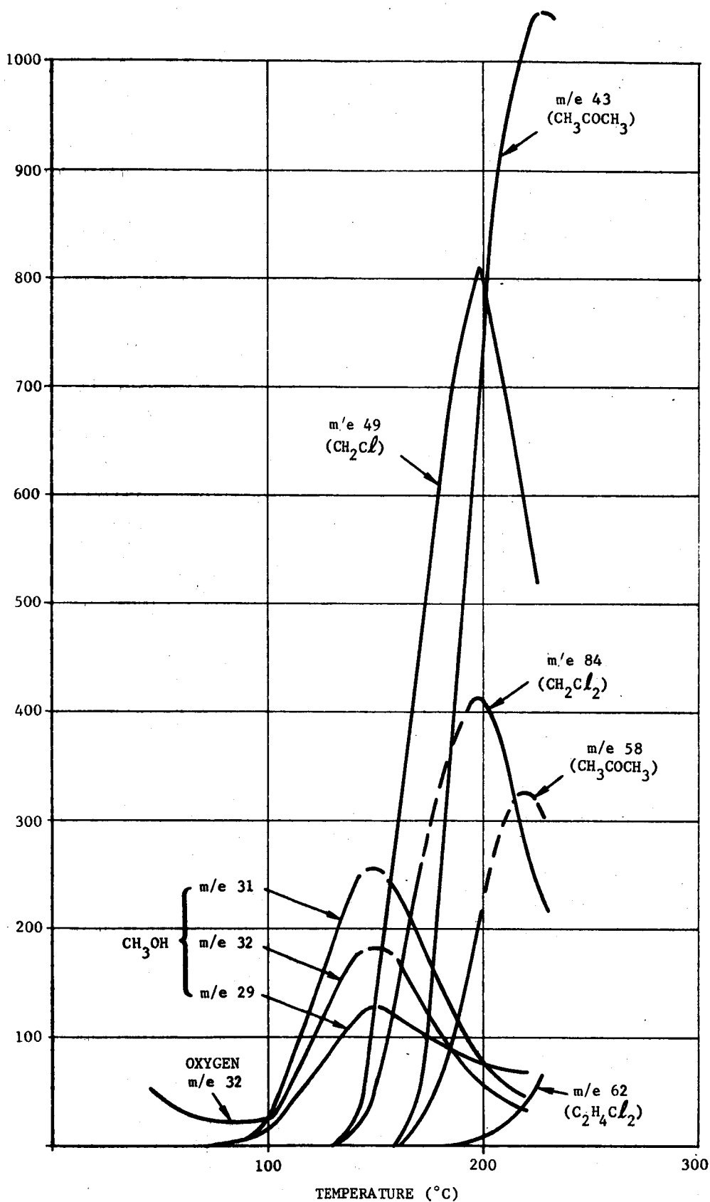
FIGURE 4-26 DESORPTION CURVE ACETONE ( CH_3COCH_3 ), METHANOL ( CH_3OH ), METHYLENE CHLORIDE ( CH_2Cl_2 ) AND ETHYLENE DICHLORIDE ( C_2H_4Cl_2 ) CHARCOAL
