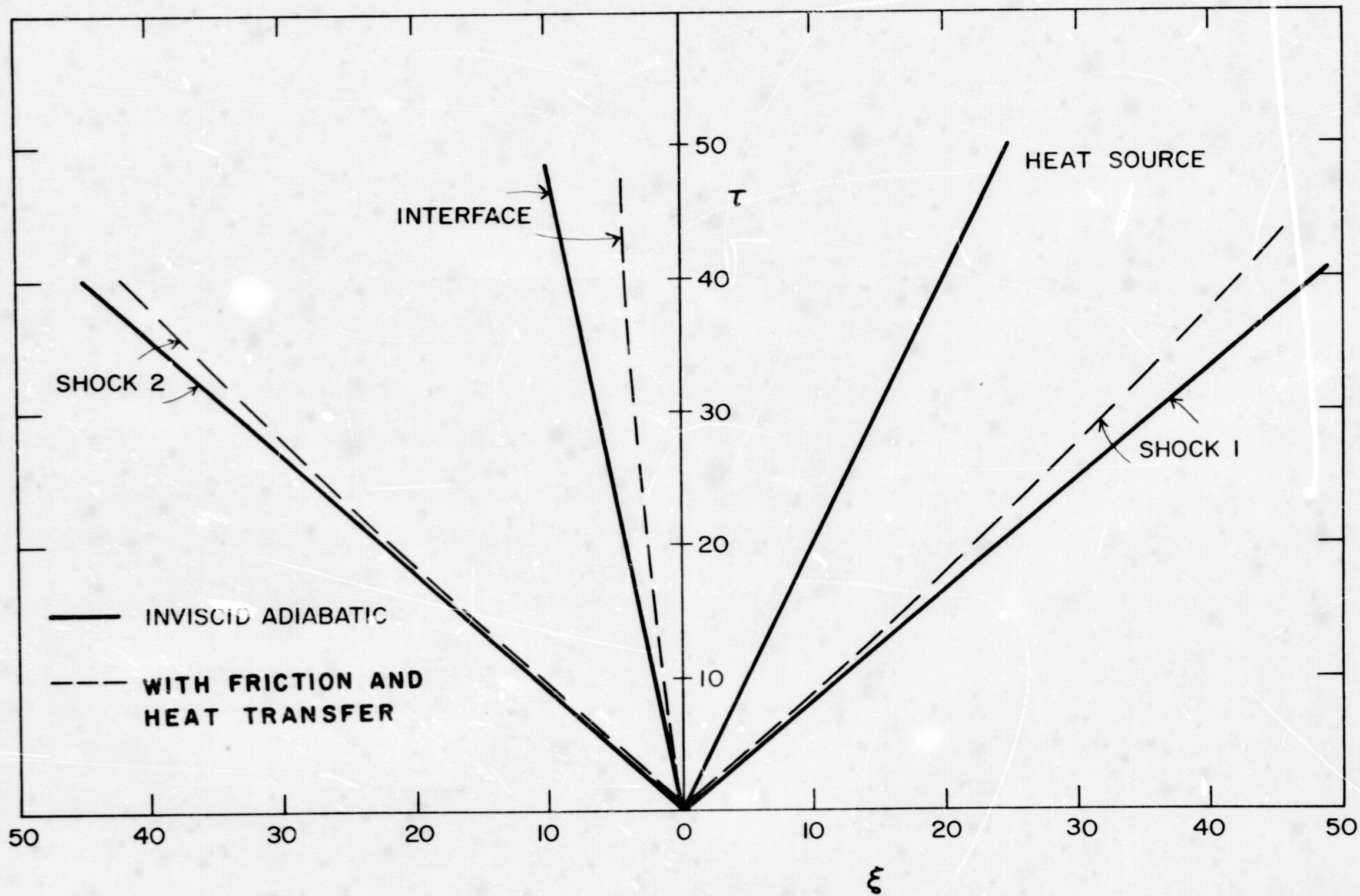
FIGURE 3. Wave diagram for inviscid adiabatic flow and for flow with friction and heat transfer
