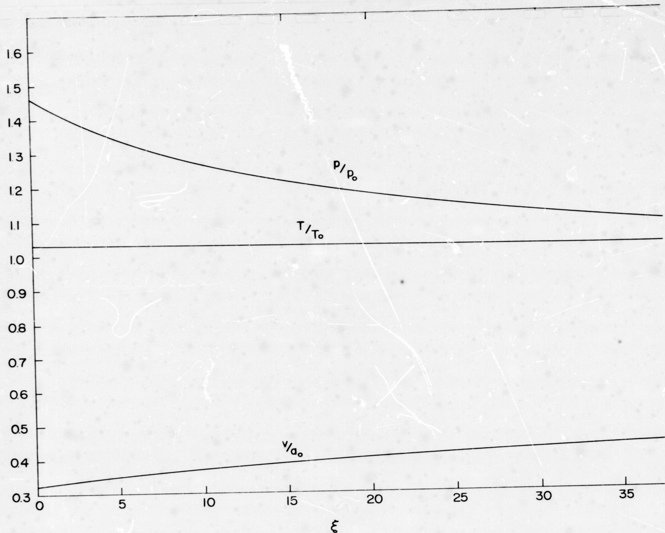
FIGURE 8. Pressure, temperature and velocity distributions ahead of the heat source at \tau = 80 in a co-ordinate system fixed to the heat source
