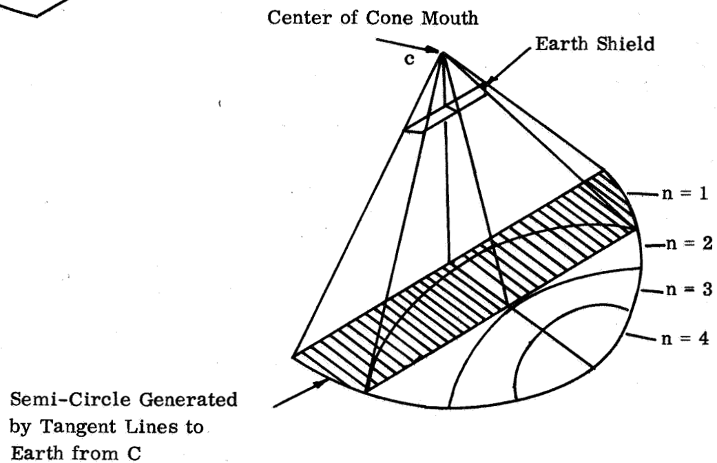
Figure 12 Earth Shield For First-Stage Cone
