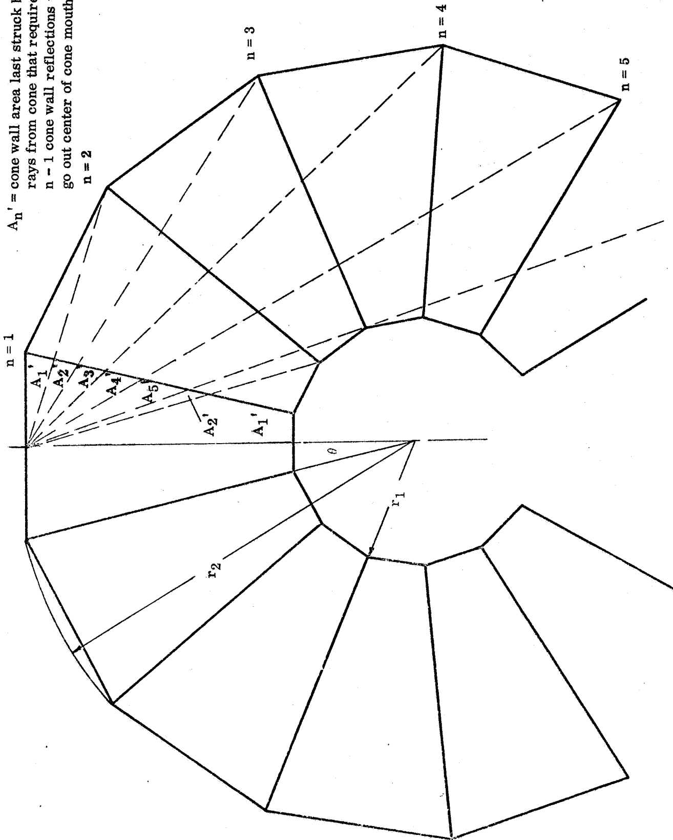
Figure 6 Vertical Plane of First Stage Reflected in Cone Walls
