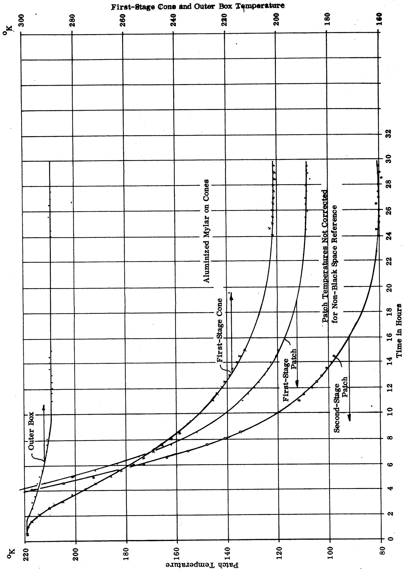
Figure 35 Radiant Cooler Test No. 7 (Aug. 28 & 29, 1967)
