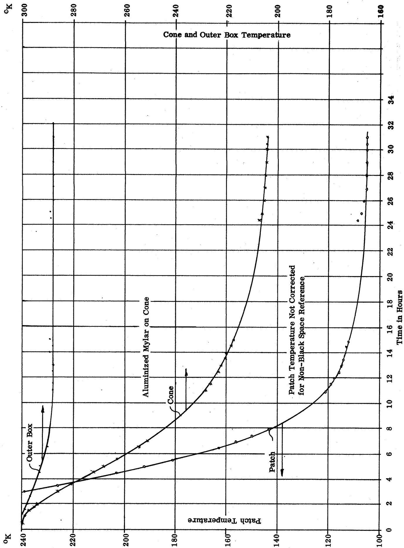
Figure 34 Radiant Cooler Test No. 6 (Aug. 21 & 22, 1967)
