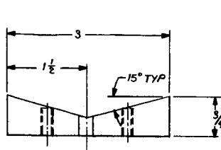
DETAIL #38 1 REQ'D ALUM BLK ANODIZE
