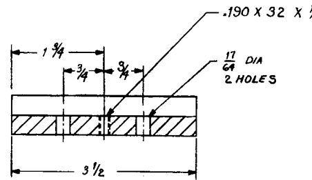
DETAIL #38 1 REQ'D ALUM BLK ANODIZE
