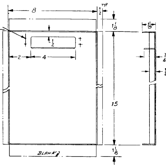
# DETAIL 61 (2) REQ'D '132 SHEET METAL PAINT BLK. HALF SCALE
