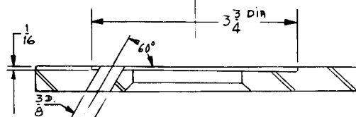
DETAIL # 44 1 REQ'D ALUM BLACK OXIDE
