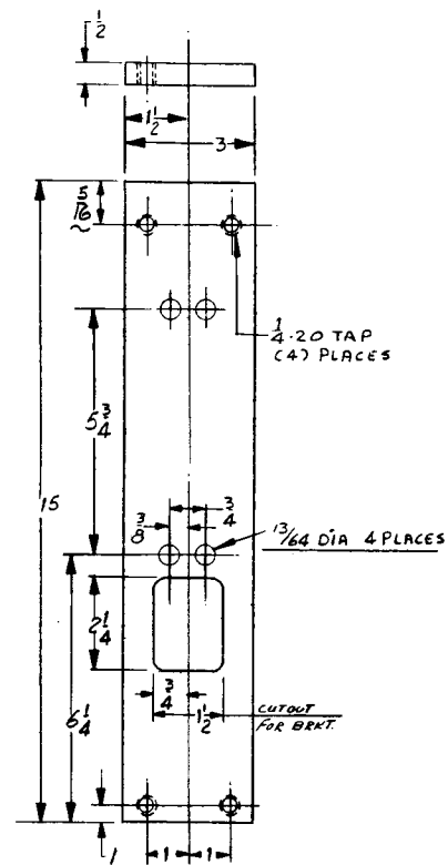
DETAIL # 21 1 REQ'D ALUM BLACK ANODIZE HALF SCALE
