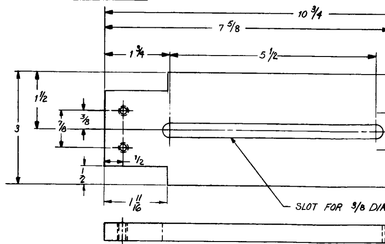
DETAIL #40 1 REQ'D ALUM BLK ANODIZE
