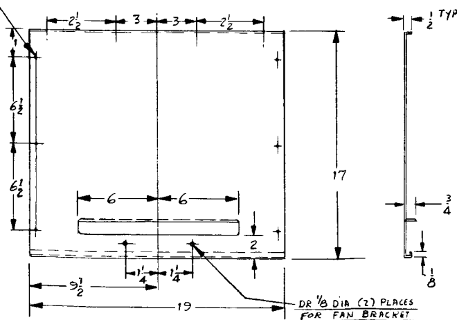
# DETAIL 61 (2) REQ'D '132 SHEET METAL PAINT BLK. HALF SCALE
