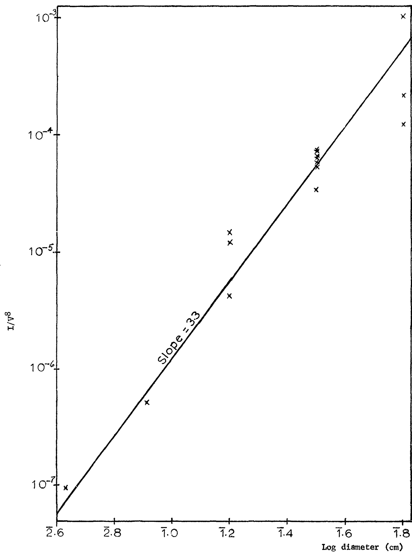
Figure 40. Dependence of Spike Intensity on Projectile Diameter, 3261\text{\AA} .
