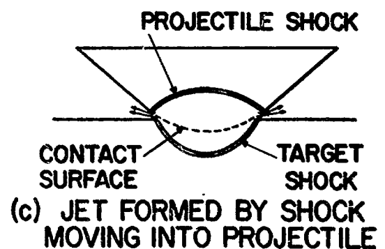
Figure 12 Jetless and Jet Producing Impacts
