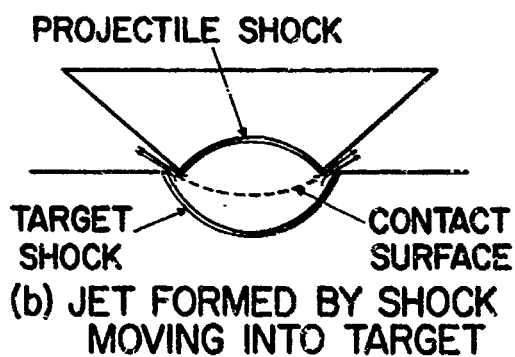
Figure 12 Jetless and Jet Producing Impacts
