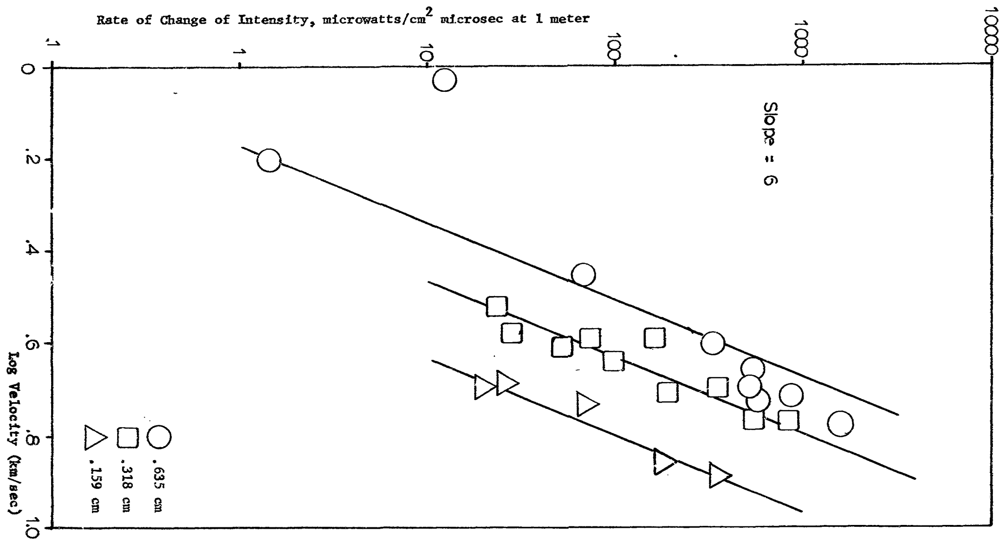
Figure 49. Spike Rate of Change of Intensity for Cu-Cd Impacts, 5085 Å
