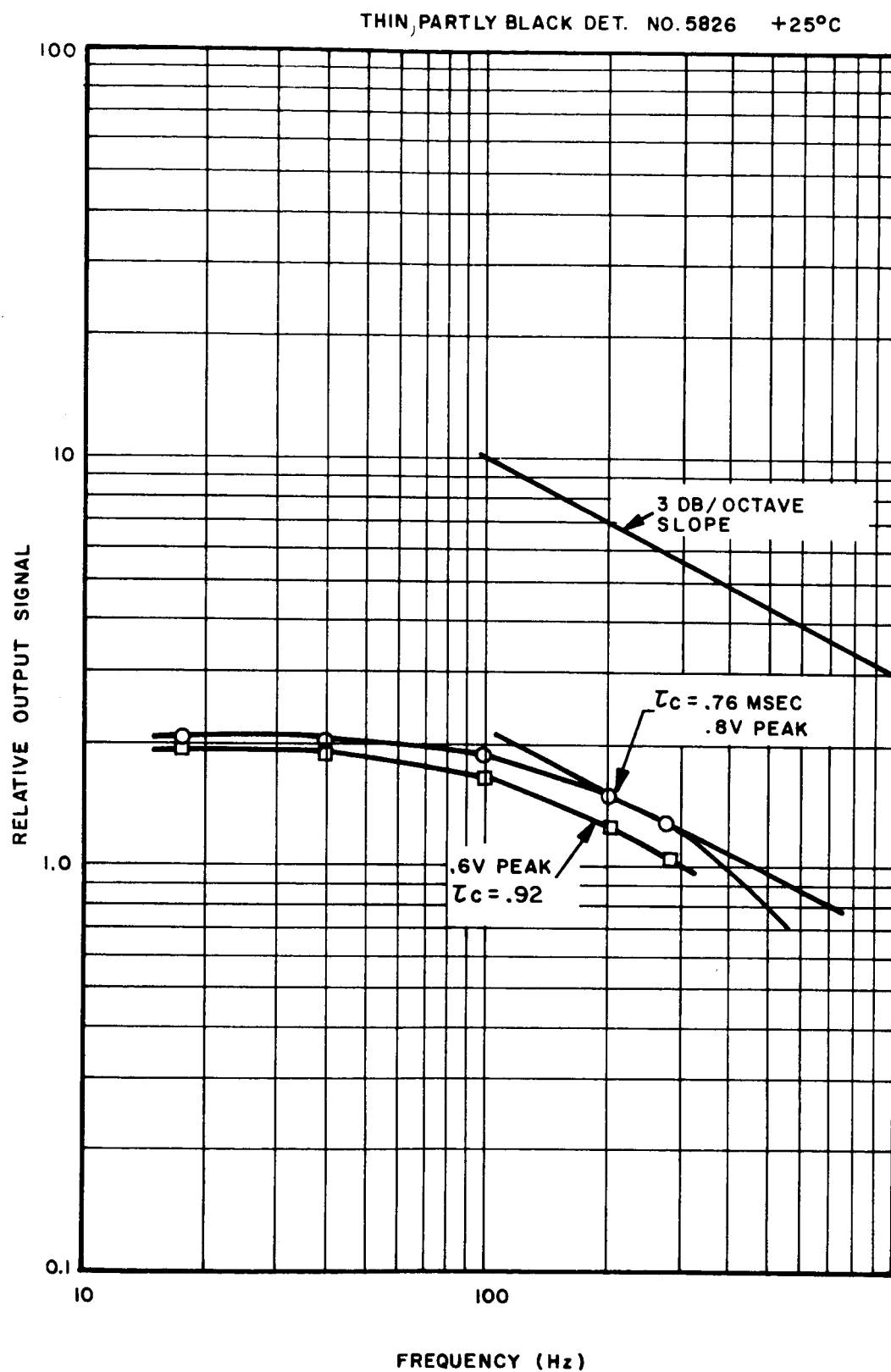
Figure I-3-1 RELATIVE OUTPUT vs. FREQUENCY DETECTOR 5826
