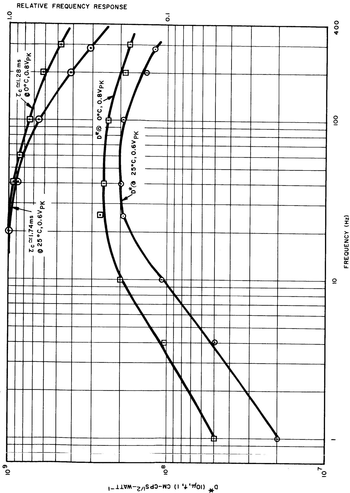
Figure 1-3-13, D^* & Z_c OF DETECTOR #5807 STANDARD THICKNESS, (16\mu) , BLACKENED
