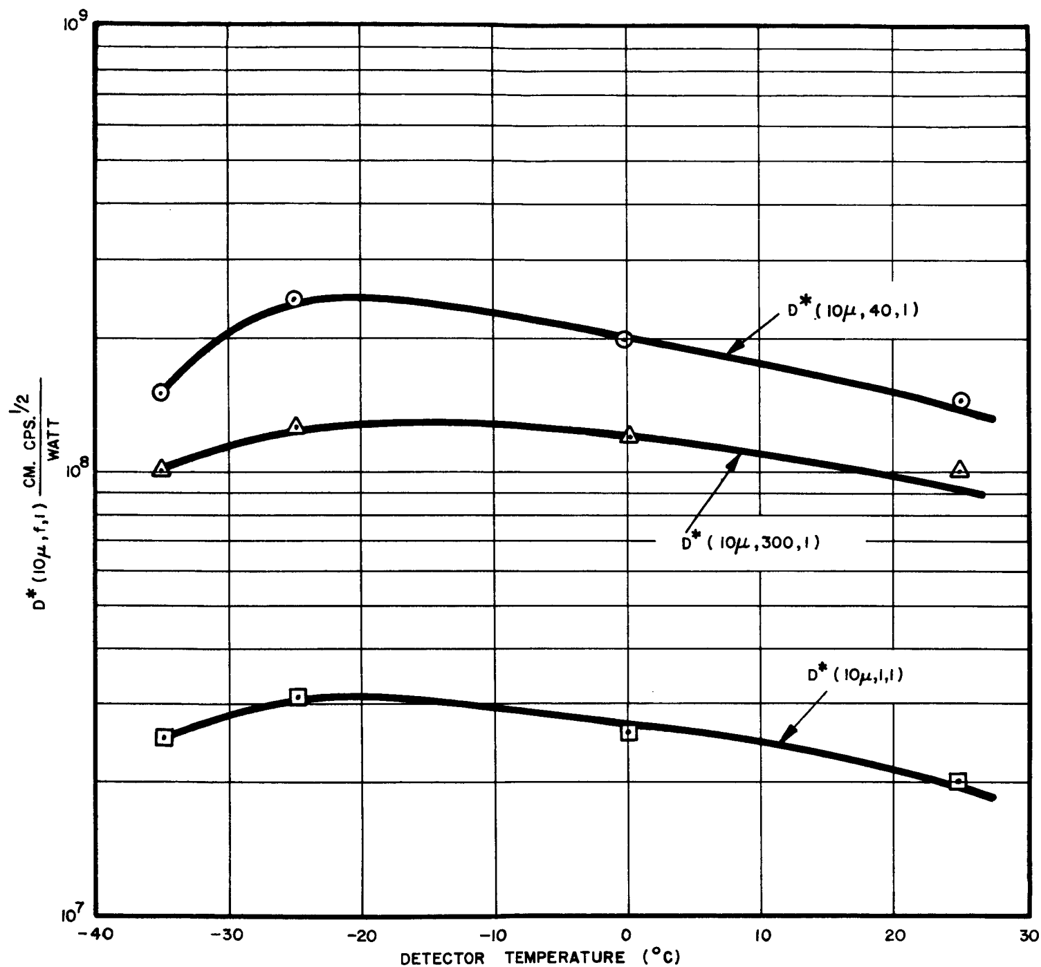
Figure I-3-12 D^* VERSUS DETECTOR TEMPERATURE FOR DETECTOR NO. 5853 THICKNESS = 15\mu (STD.)
