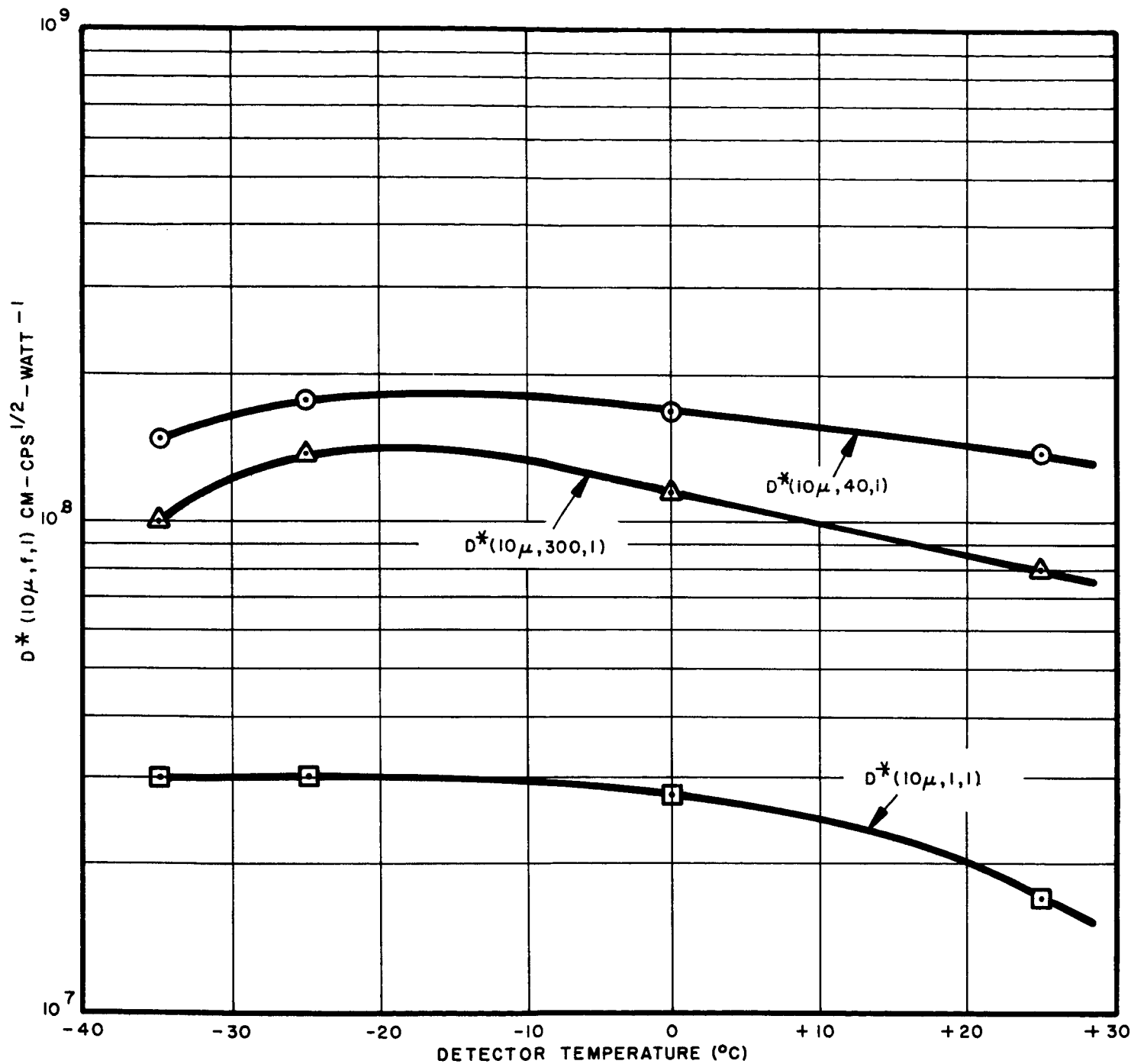
Figure 1-3-8, DETECTIVITY AS A FUNCTION OF DETECTOR TEMPERATURE FOR DETECTOR # 58II, THIN FLAKE ( 8\mu )
