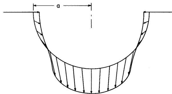
3 e. CONSTANT DISPLACEMENT U_x = 0.01a .
