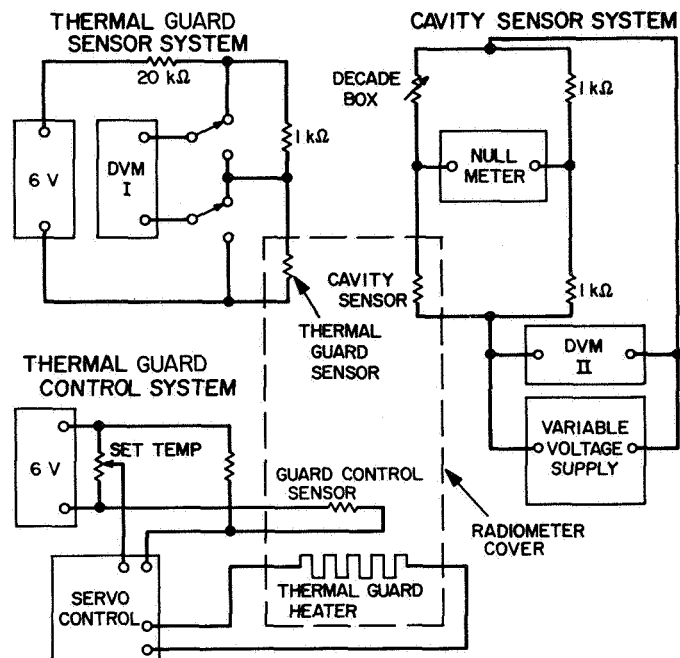
Fig. 2. Electronic circuit
