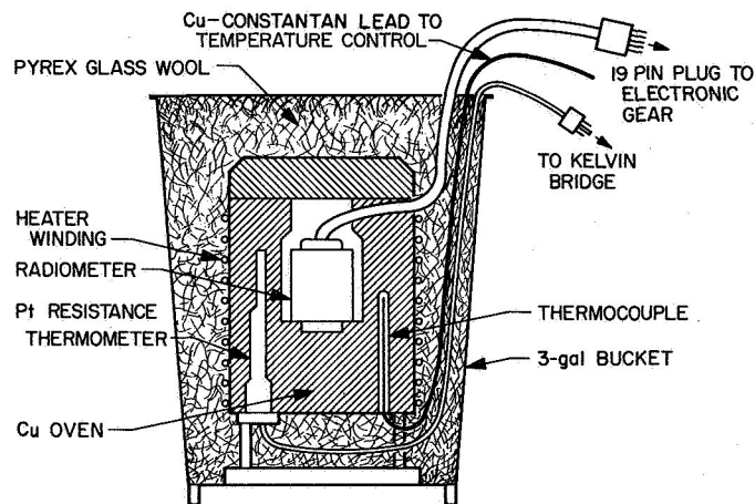
Fig. 3. Thermometer calibrating oven
