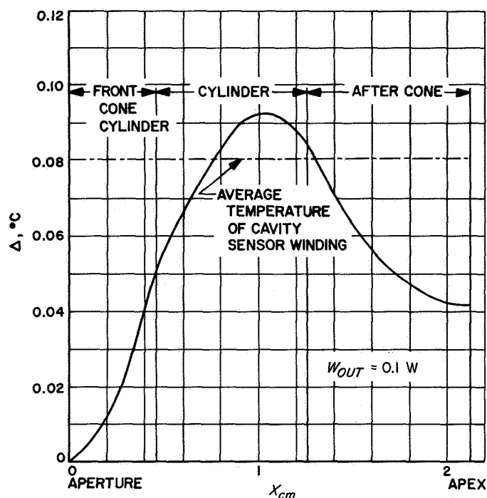
Fig. 5. Cavity temperature distribution
