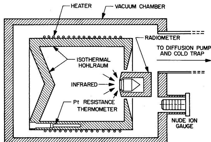
Fig. 6. Setup for verifying accuracy of absolute radiometers
