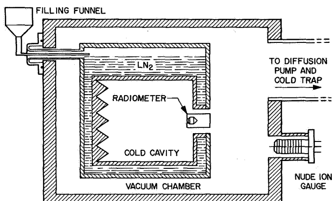
Fig. 4. Radiometer in cold cavity and vacuum chamber
