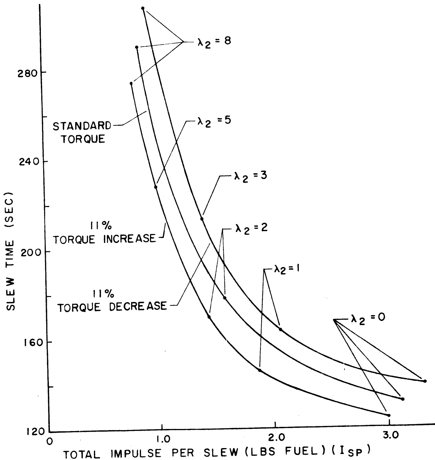
FIGURE 3.8 TIME - FUEL CURVES FOR IDEAL THRUSTER (MOJAVE - QUITO)
