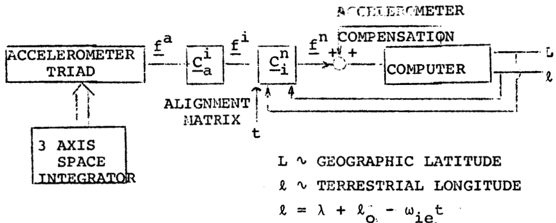
Fig. 2 Computation in geographical coordinates.
