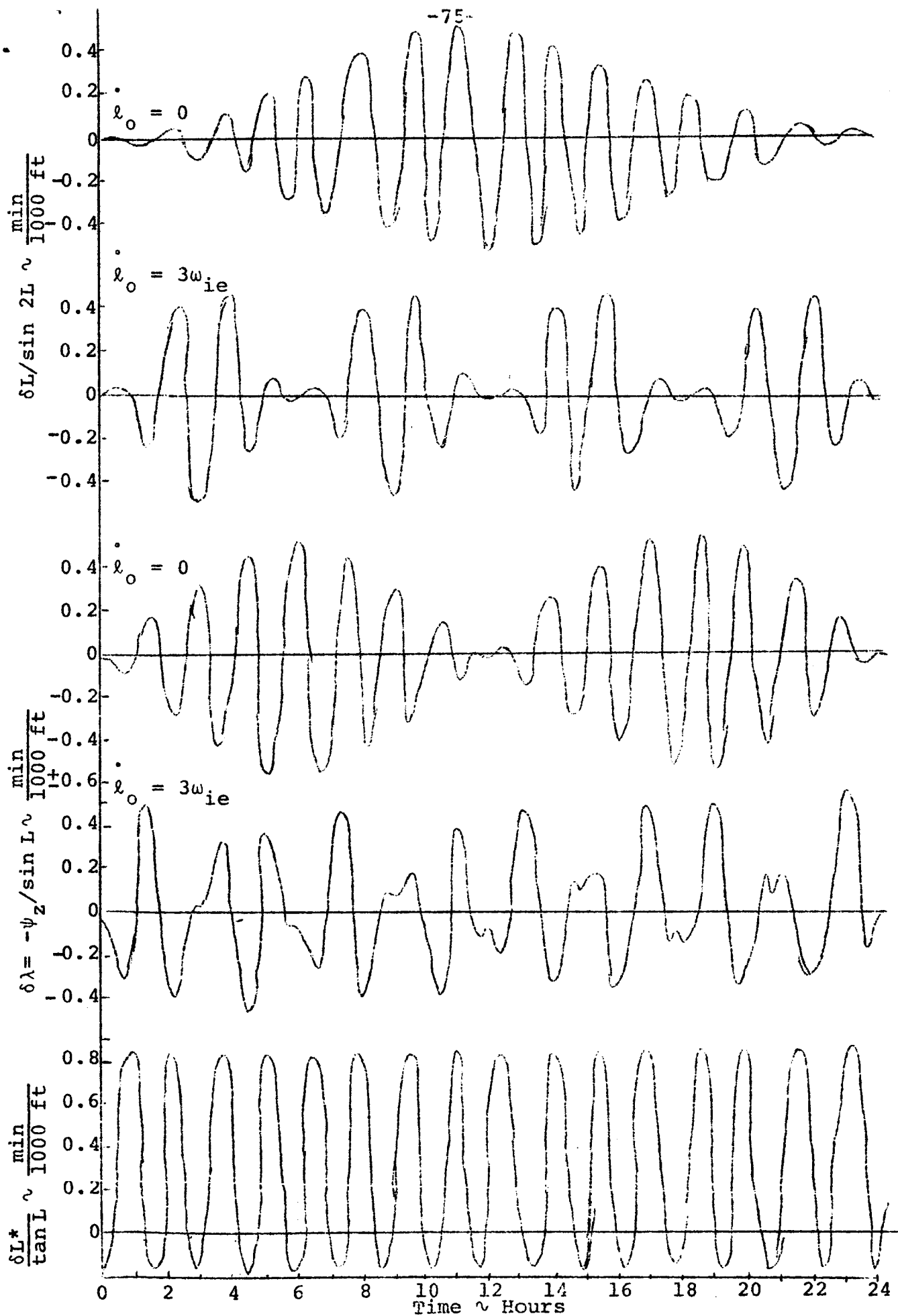
Figure 11 ~ Altimeter-caused error - inertial computation
