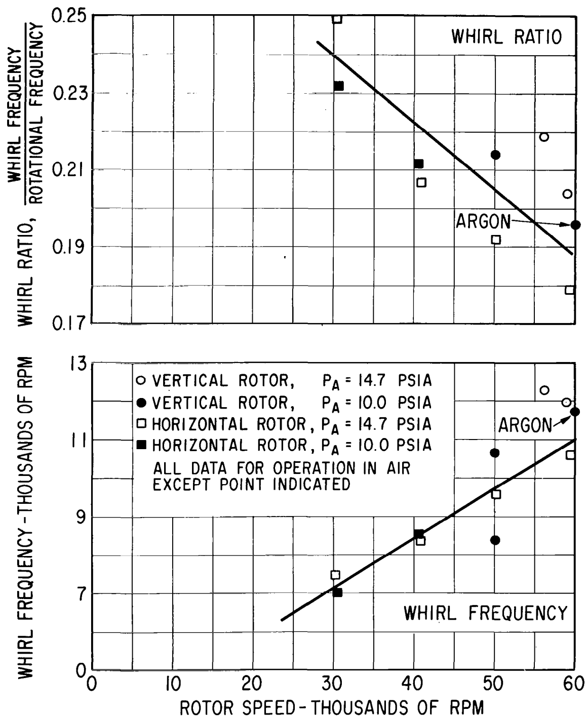
Fig. IV-30 - Whirl Frequency And Whirl-Frequency Ratio Versus Rotor Speed For The Final No. 2 Journal Bearing Design
