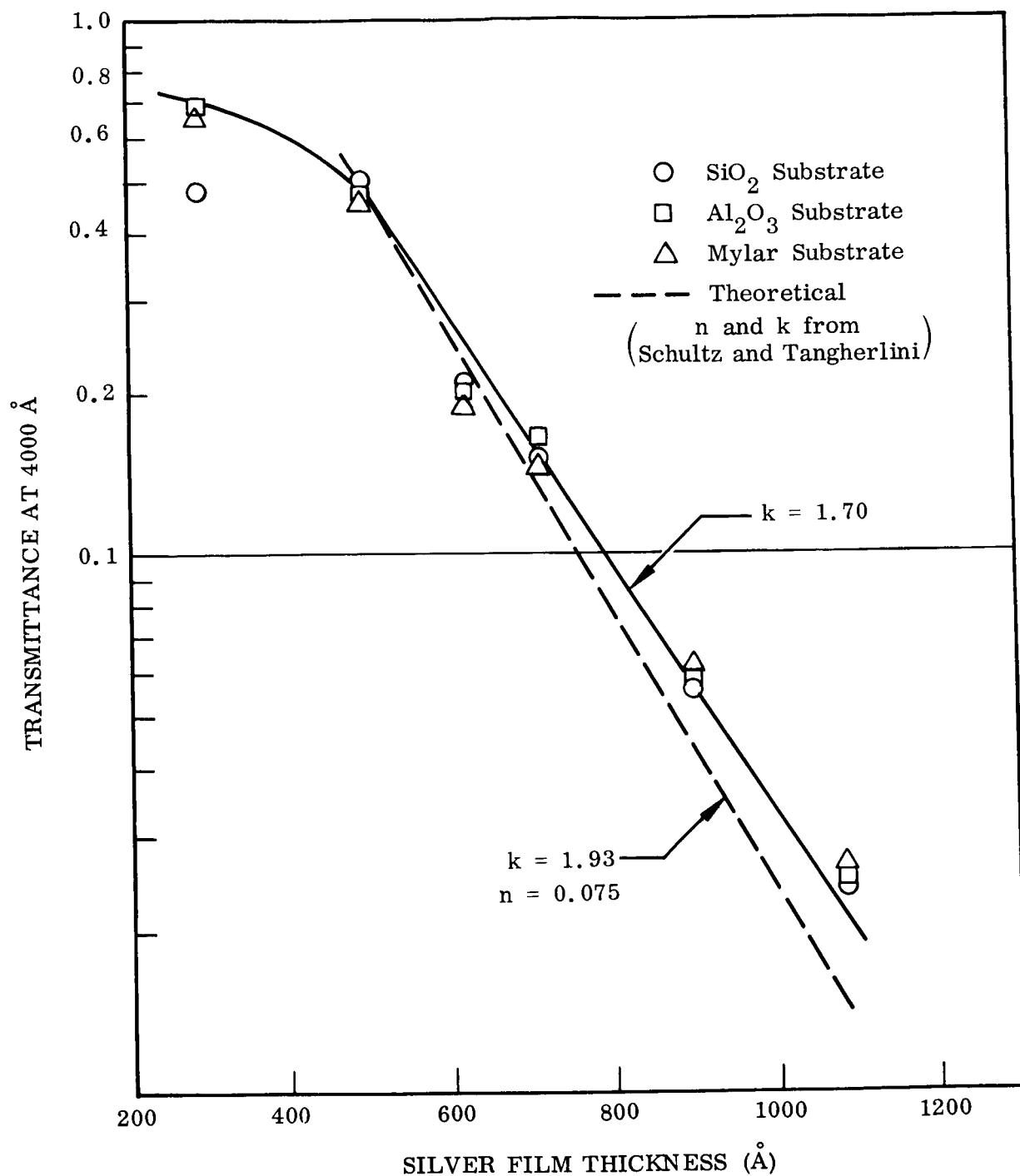
Fig. 6-15 Transmittance of Silver on Various Substrates as a Function of Film Thickness at \lambda = 4000 \text{ Å}
