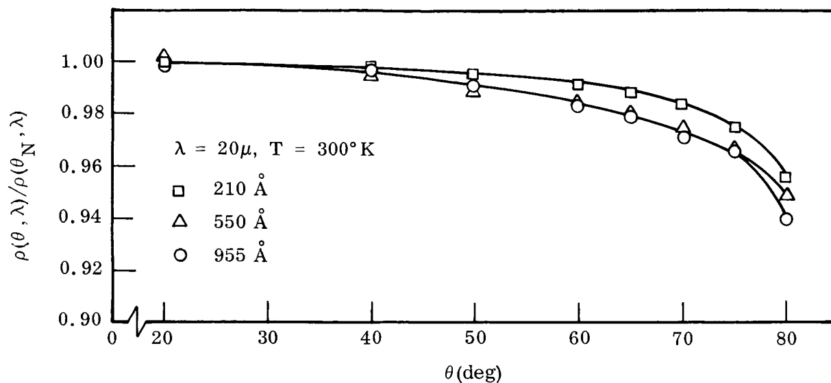
Fig. 6-11 Relative Directional Reflectance of \text{Ag}/\text{Al}_2\text{O}_3 Samples at 20\mu
