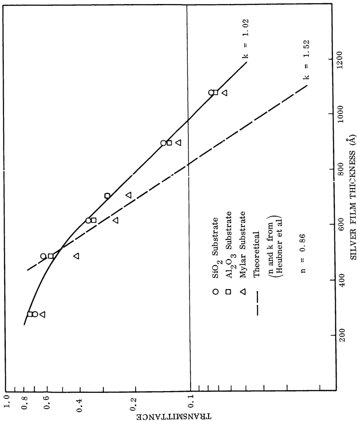
Fig. 6-14 Transmittance of Silver on Various Substrates as a Function of Film Thickness at \lambda = 3600 \text{ Å}
