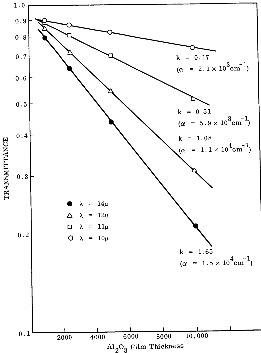
Fig. 6-18 Infrared Absorption Coefficients of \text{Al}_2\text{O}_3 Films
