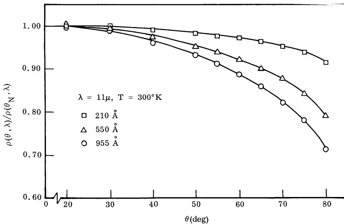
Fig. 6-12 Relative Directional Reflectance of \text{Ag}/\text{Al}_2\text{O}_3 Samples at 11\mu
