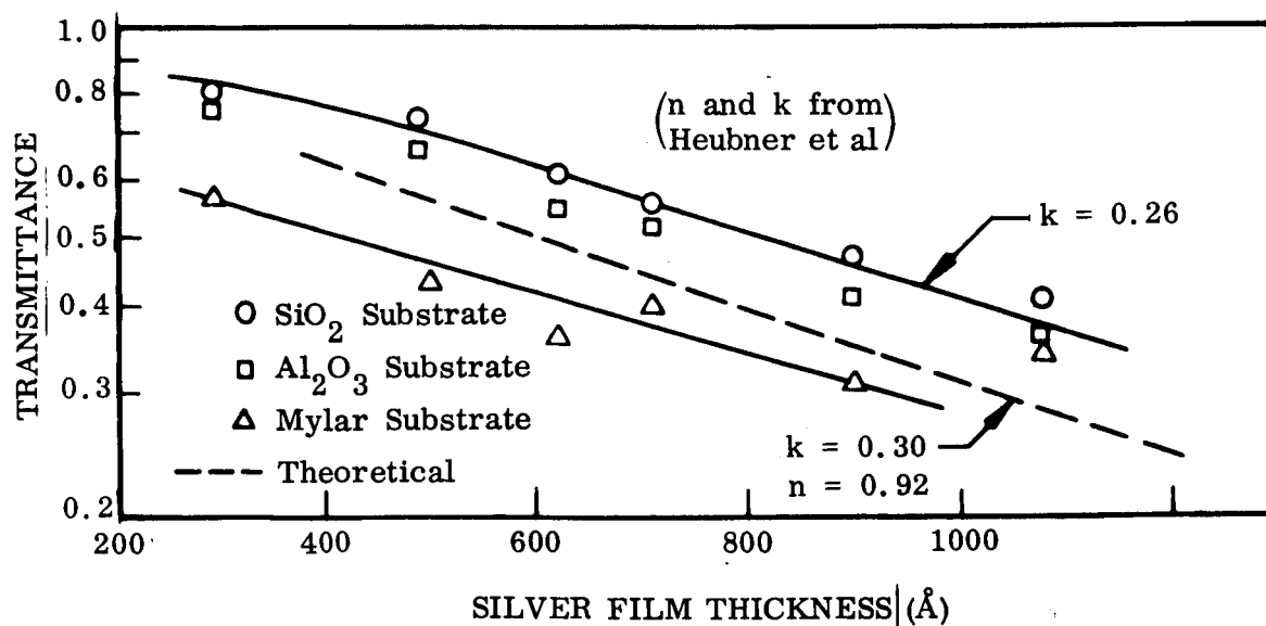
Fig. 6-13 Transmittance of Silver on Various Substrates as a Function of Film Thickness at \lambda = 3220 Å
