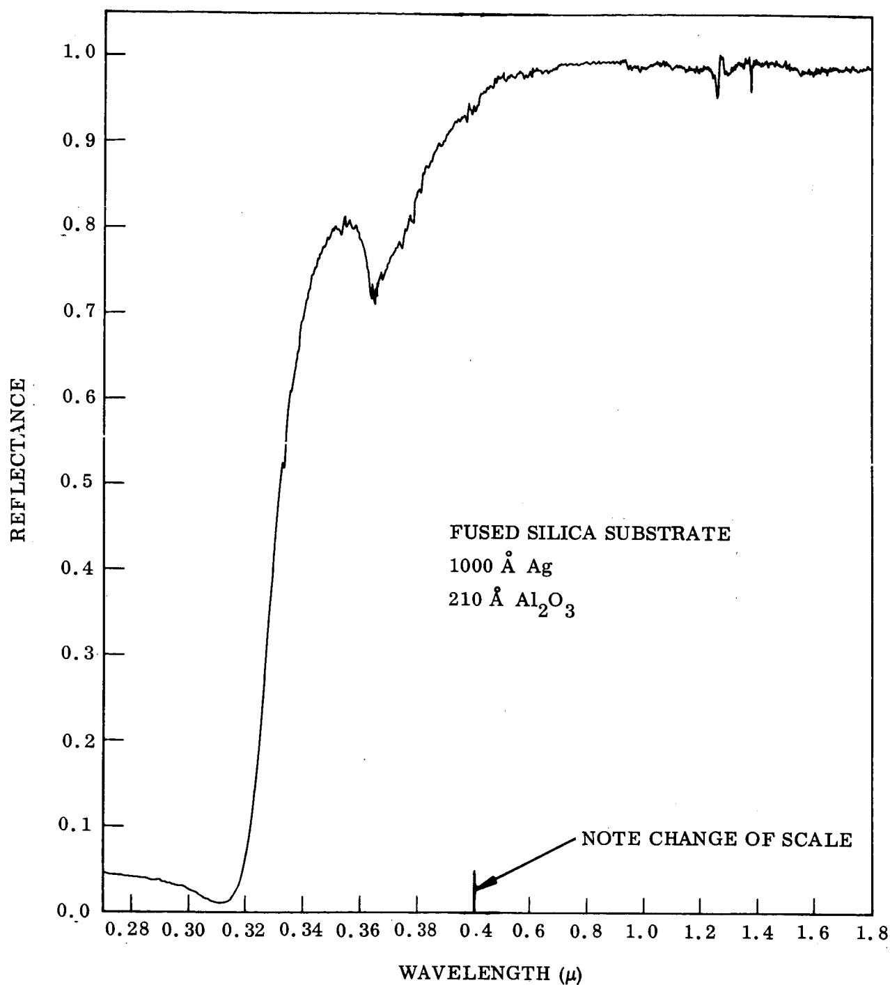
Fig. 6-6 Spectral Reflectance of 210 Å Aluminum Oxide Film on Silver at Less Than 1.8 \mu
