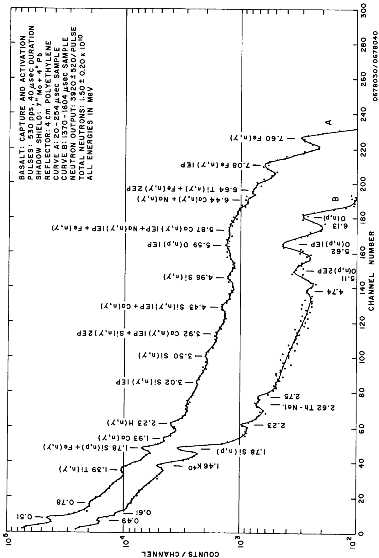
Figure 3 CAPTURE AND CYCLIC ACTIVATION SPECTRA OF BASALT (4-cm-thick Polyethylene Reflector, 7 in. Mo + 4 in. Pb Shadow Shield)
