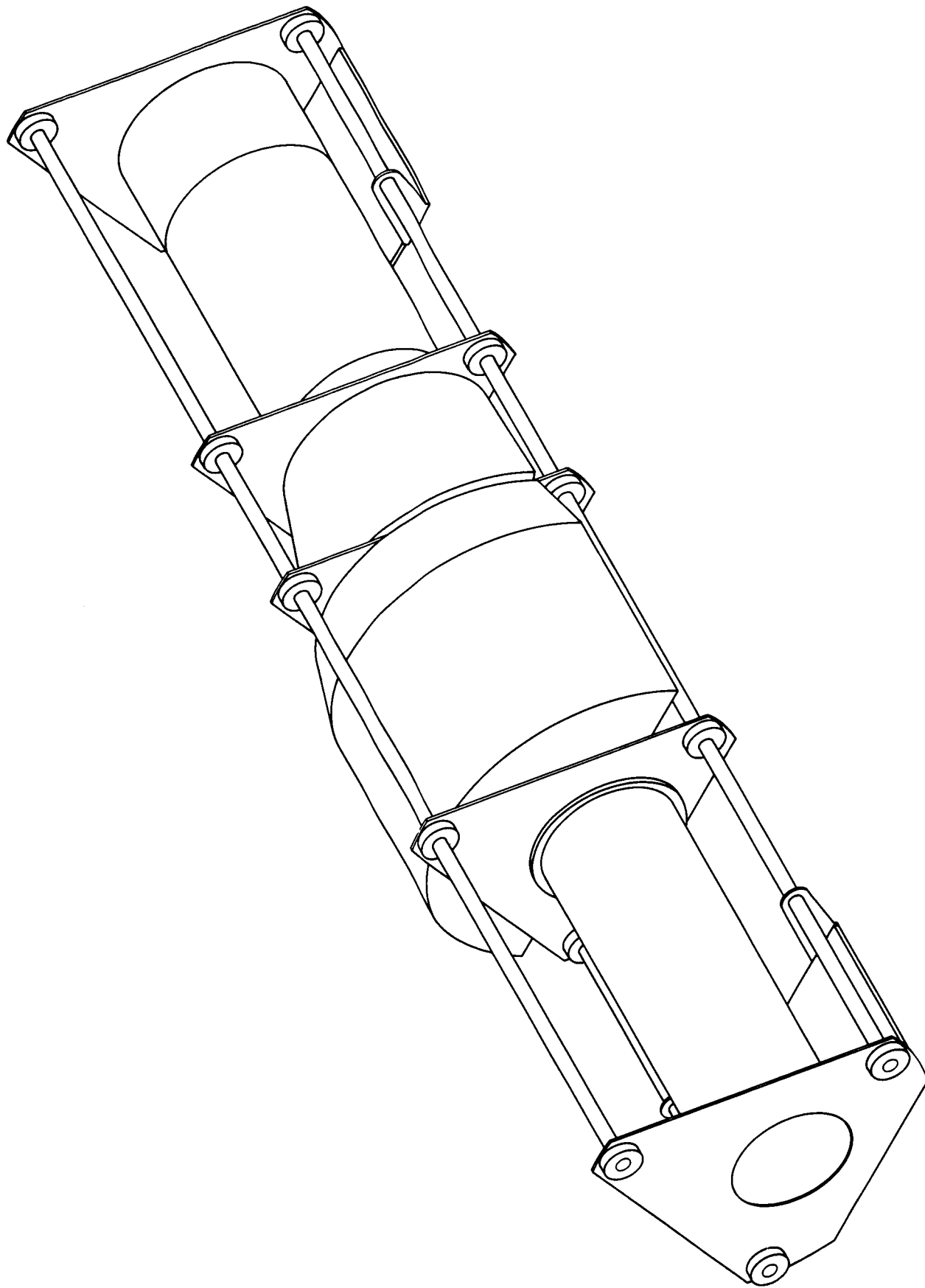
Figure 17 COMBINED NEUTRON EXPERIMENT DETECTOR PROBE (View with 8-cm-thick Reflector)
