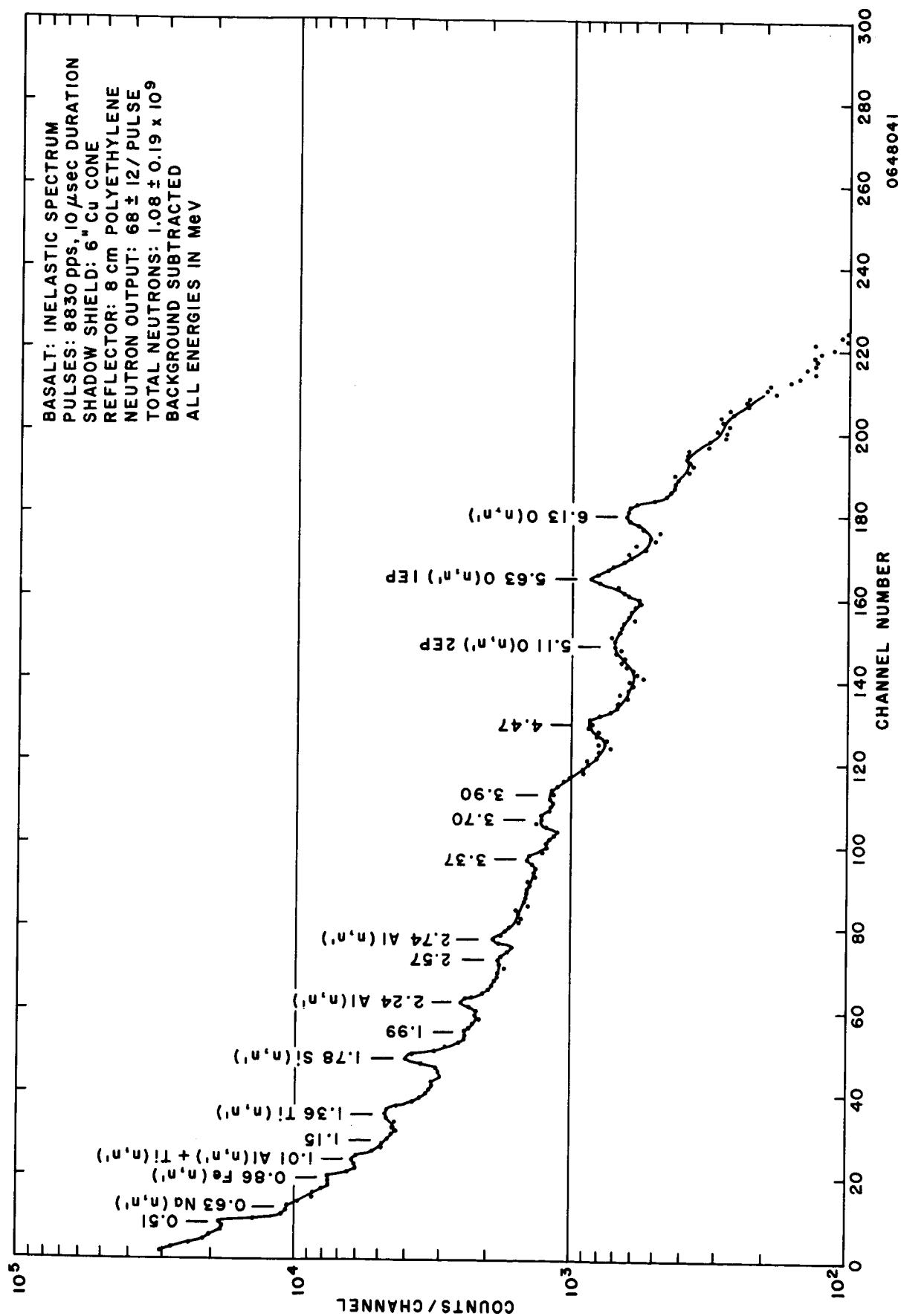
Figure 11 INELASTIC SPECTRUM OF BASALT (8-cm-thick Polyethylene Reflector, 6 in. Cu Shadow Shield)
