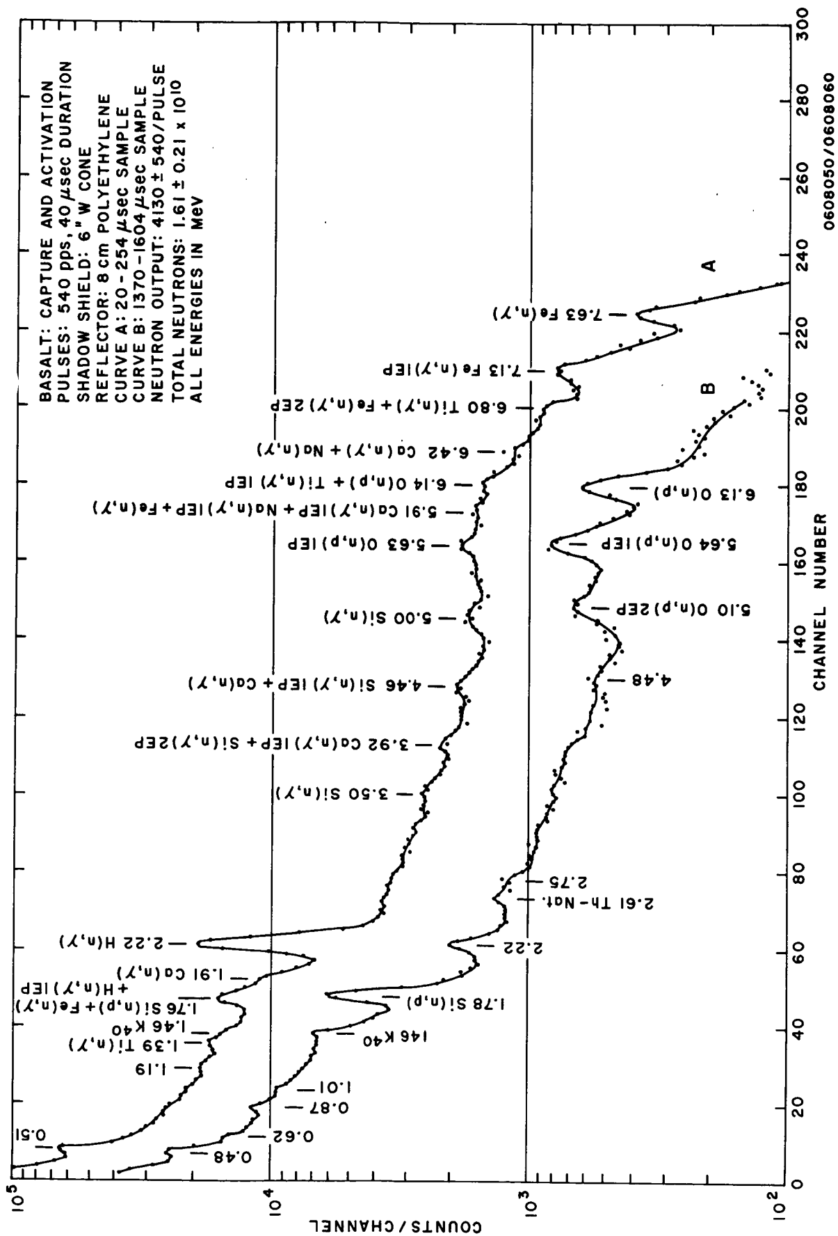
Figure 6 CAPTURE AND CYCLIC ACTIVATION SPECTRA OF BASALT (8-cm-thick Polyethylene Reflector, 6 in. W Shadow Shield)
