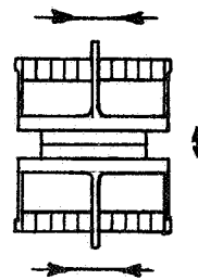
Clutch Assembly
