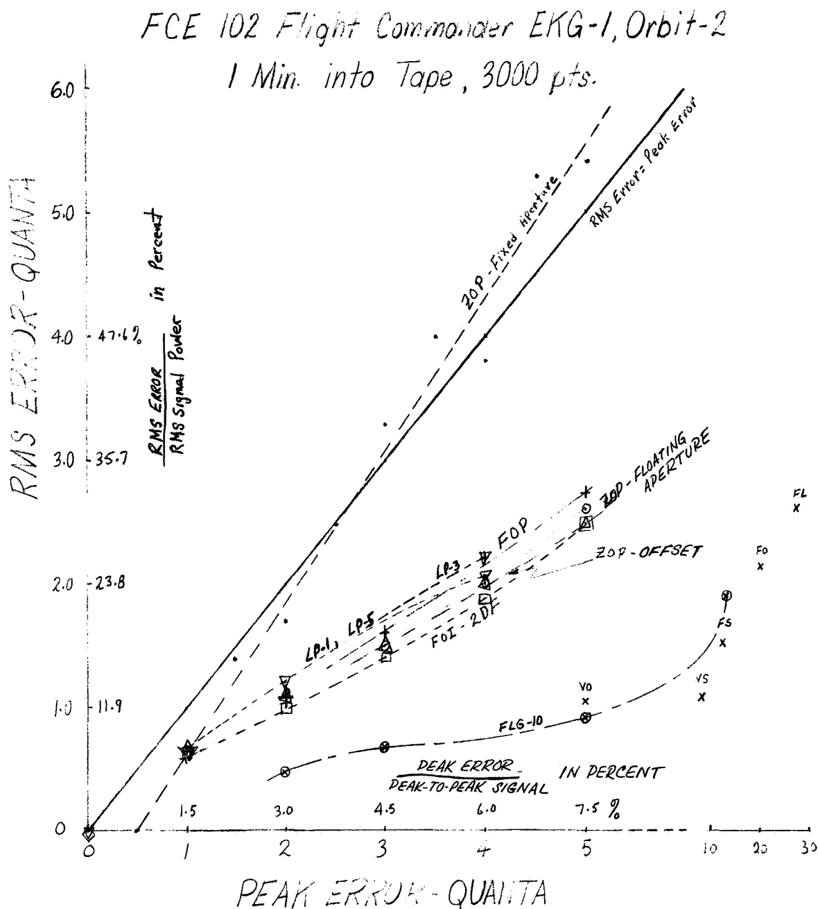
Figure 3-13. RMS Error vs Peak Error for Aperture Techniques, FCE 102, Flight Commander, EKG 1
