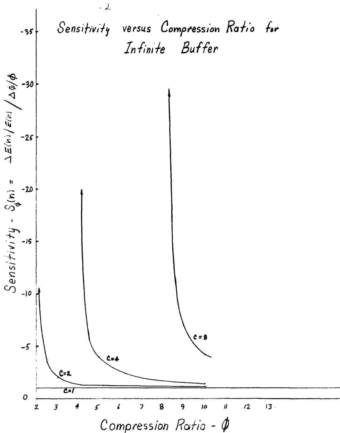
Figure C-2. Sensitivity vs Compression Ratio for Infinite Buffer
