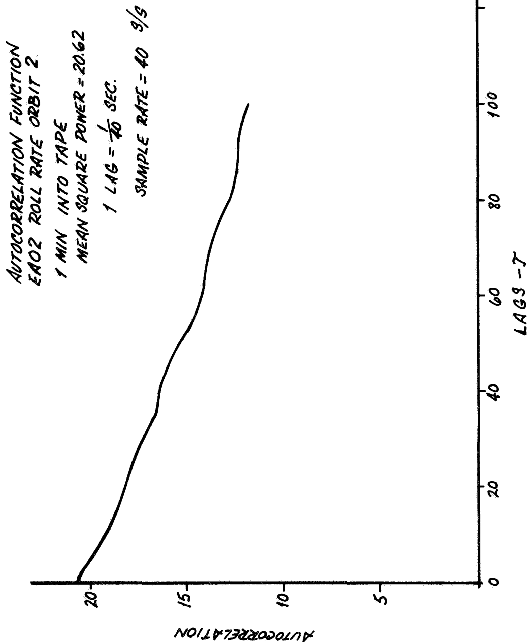
Figure 3-9. Autocorrelation Function, EA 02, Roll Rate
