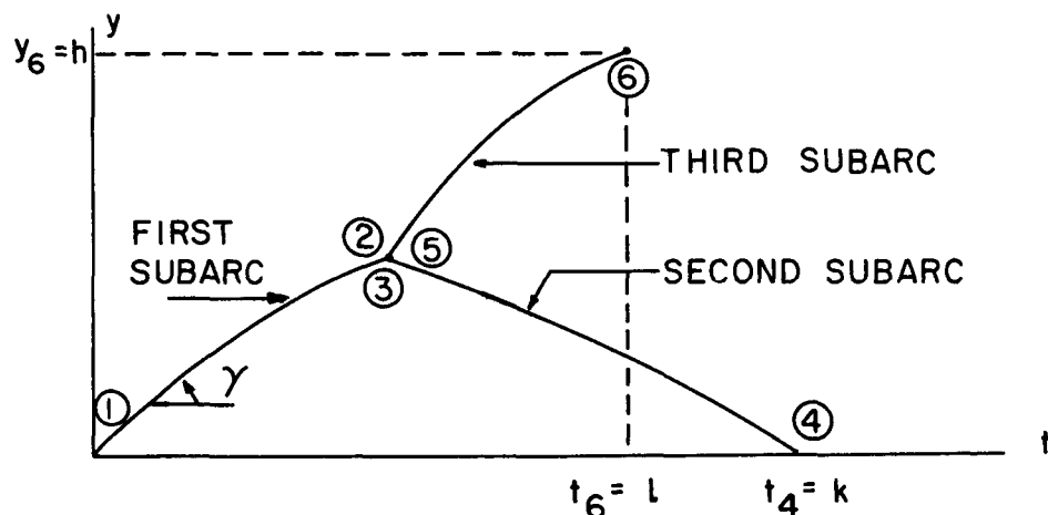
FIGURE 3.1 BRANCHED TRAJECTORY CONNECTING THREE POINTS
