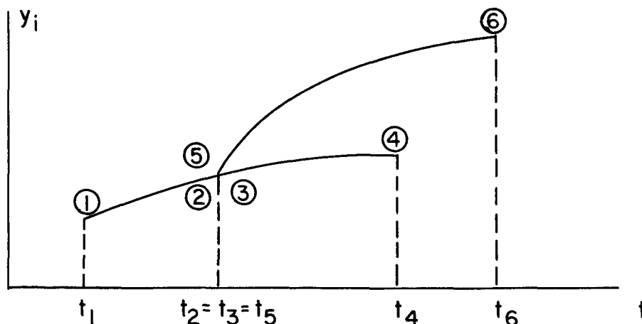
FIGURE 2.4 BRANCHED TRAJECTORIES
