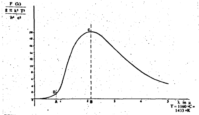
Fig. 1. Emission Spectrum of Infrared Radiation from the Heater (Absorbed in a Blackbody). The Ratio Between the Area ABCD and the Total Area Between the Curve of the Axis of the Abscissa and the Extreme Ordinate Indicates that 26% of the Radiant Energy Emitted by the Source has a Wavelength Between 0.8 and 2.2 \mu .
