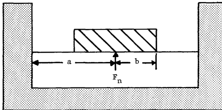
Fig. 3-3. Sketch of Single-Diaphragm Accelerometer.
