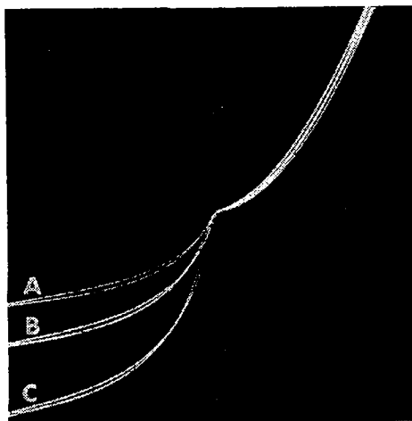
Fig. 3-17. Current-Voltage Characteristics of the +1 g Accelerometer Shown in Fig. 3-16. A = -1 g, B = 0 g and C = +1 g. The Vertical Scale is 0.1 ma/div. for Both Forward and Reverse Modes. The Horizontal Scale is 0.5 V/div. for Forward and -5 V/div. for Reverse Mode.
