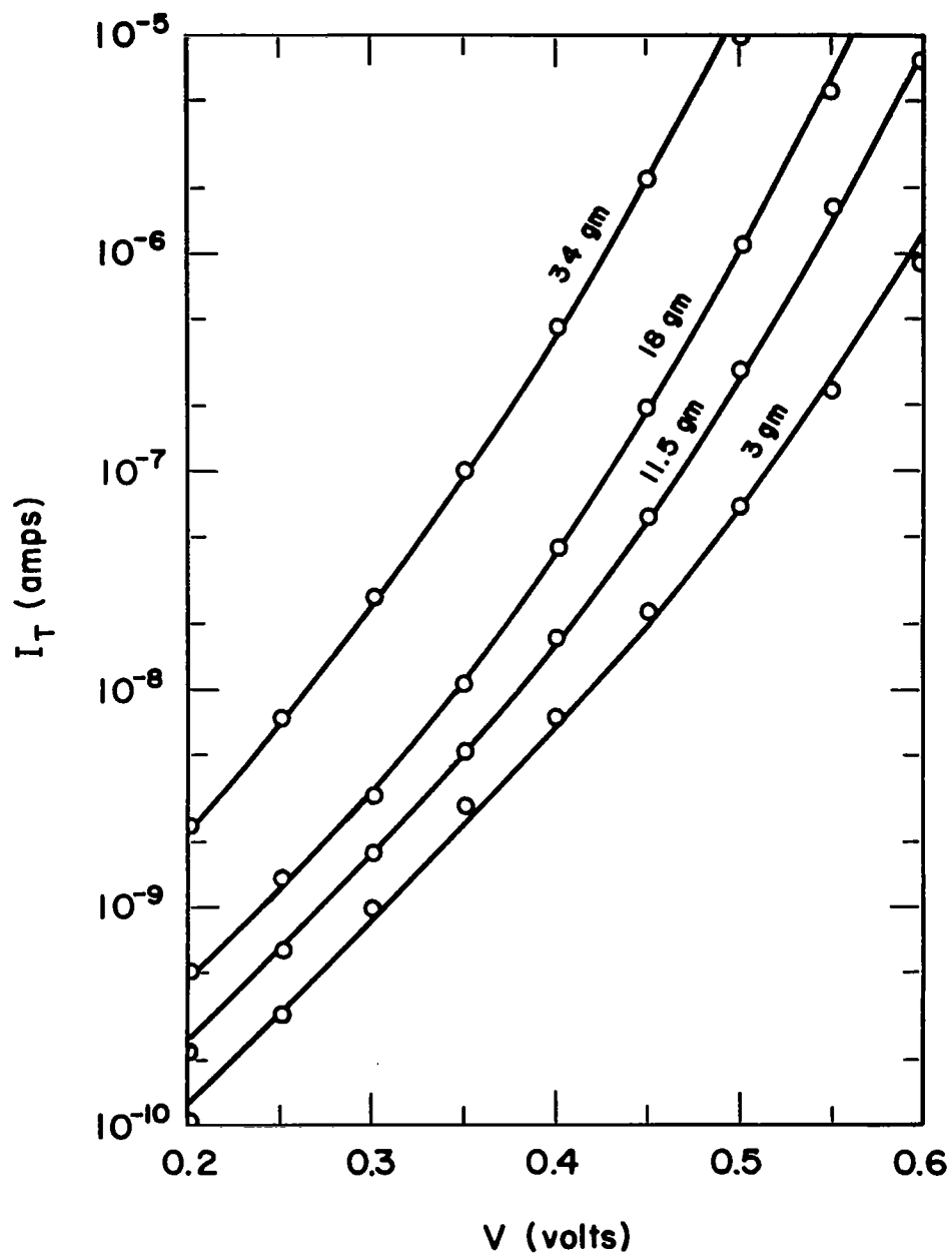
Figure 1.1 Forward Biased I-V characteristics of a mesa diode subjected to stress. (The applied force is shown.)
