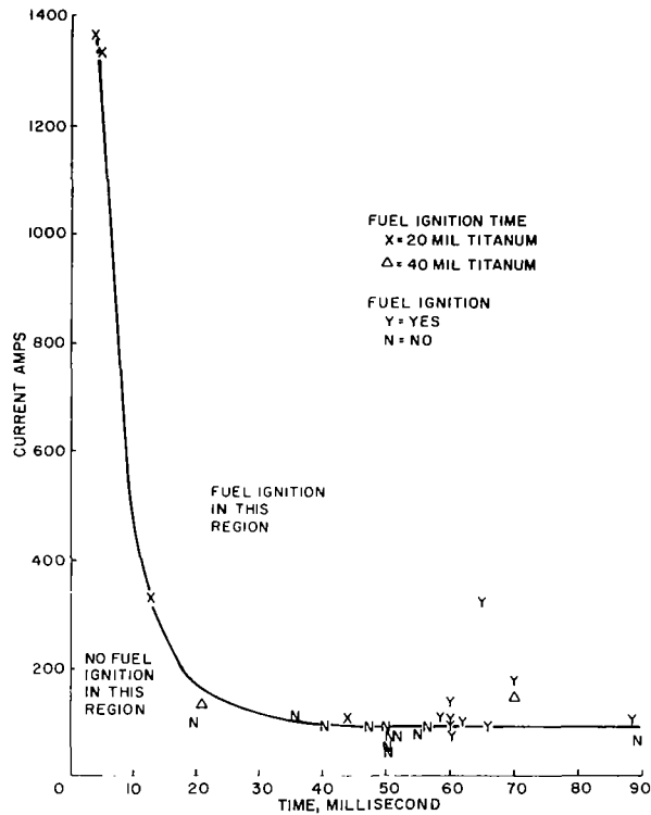
FIGURE 6. Fuel Ignition Time vs Continuing Current Amplitude for 20 & 40 Mil Titanium. 1.5 Stoichiometric Propane/Air Mixture.
