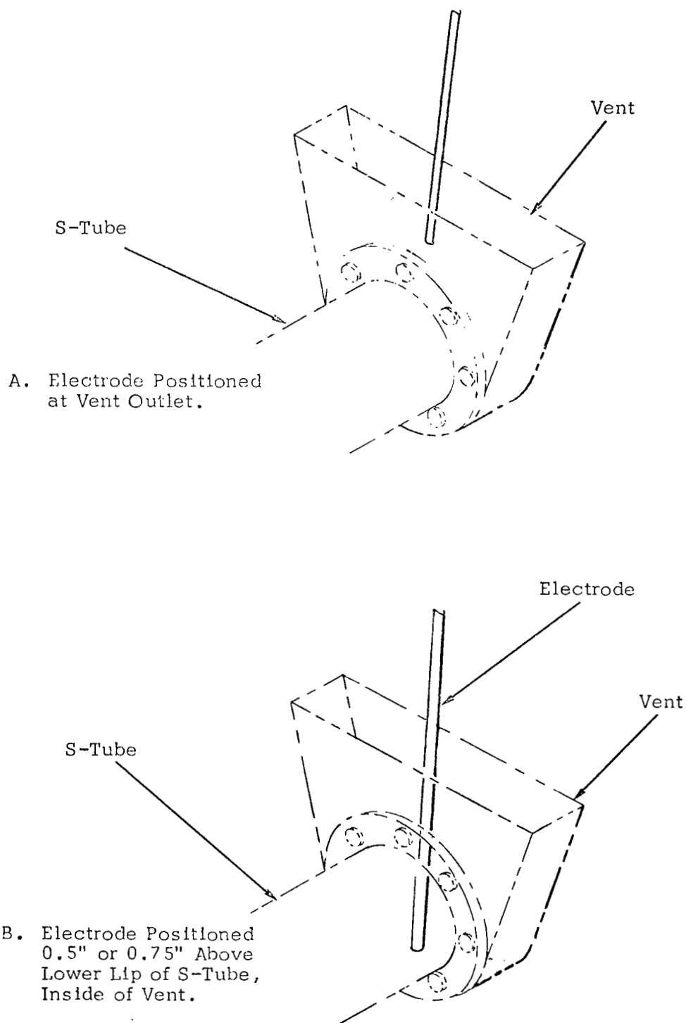
FIGURE 8. Electrode Arrangement at Vent Outlet.
