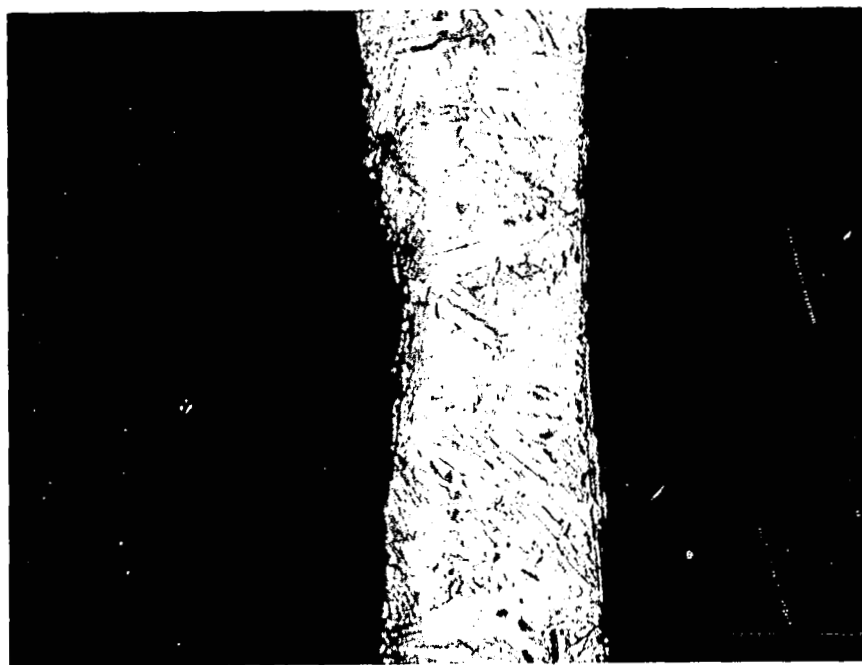
FIGURE 15. Pure Titanium, 0.005" Thick, 500X, Two Electrical Discharges.
