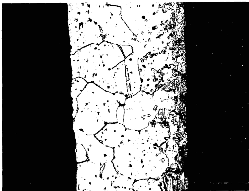
FIGURE 14. Pure Titanium, 0.005" Thick, 500X, One Electrical Discharge.
