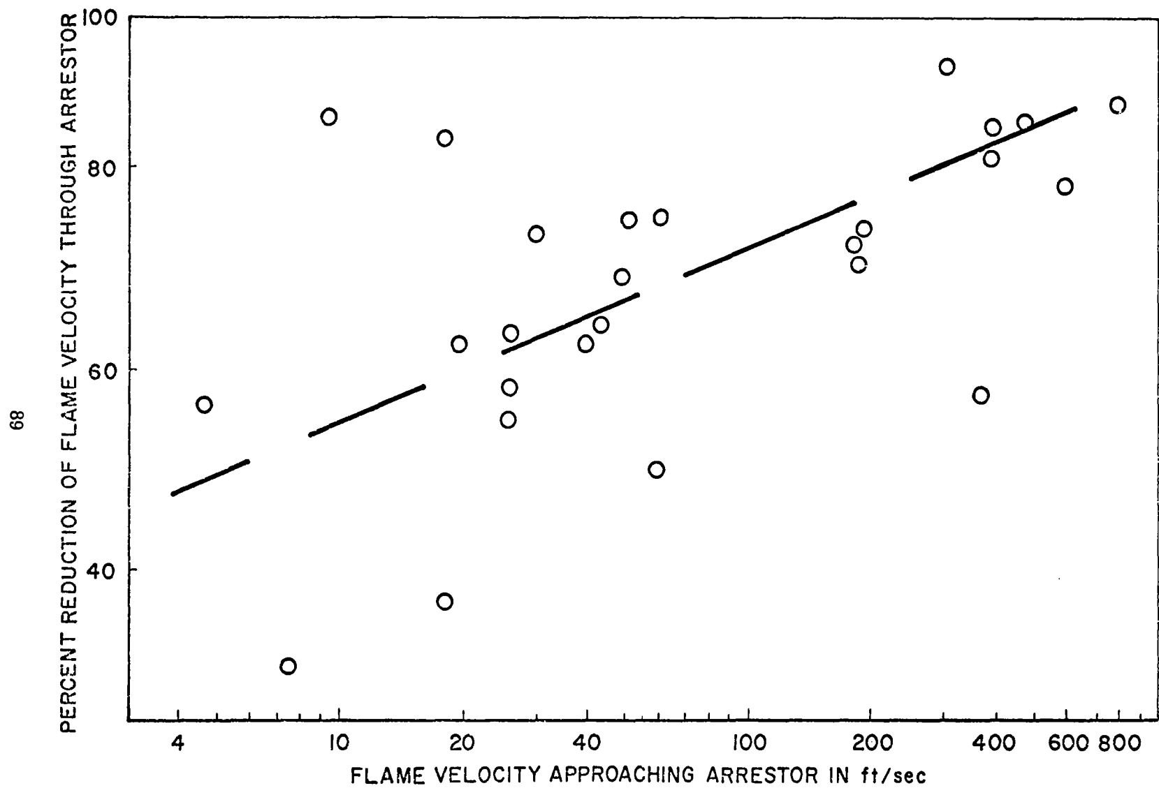
FIGURE 11. Effectiveness of Arrester in Slowing Approaching Flame.
