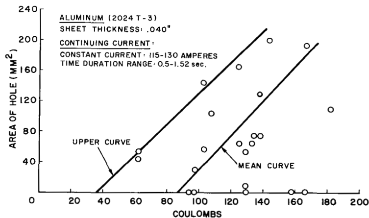
FIGURE 5. Area of Hole Formed Vs. Coulomb Content of Lightning Strike.
