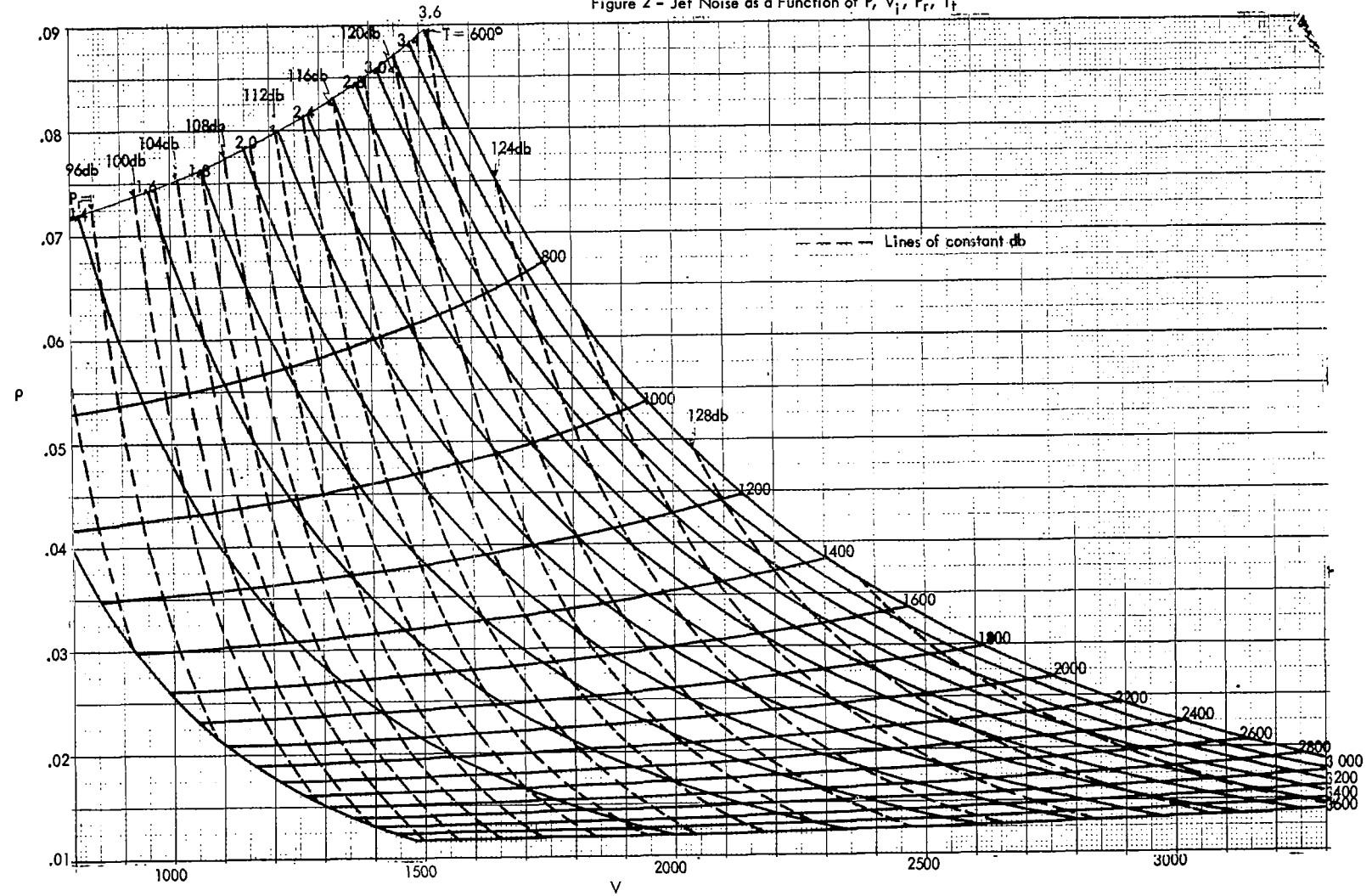
Figure 2 - Jet Noise as a Function of P , V_j , P_r , T_t
