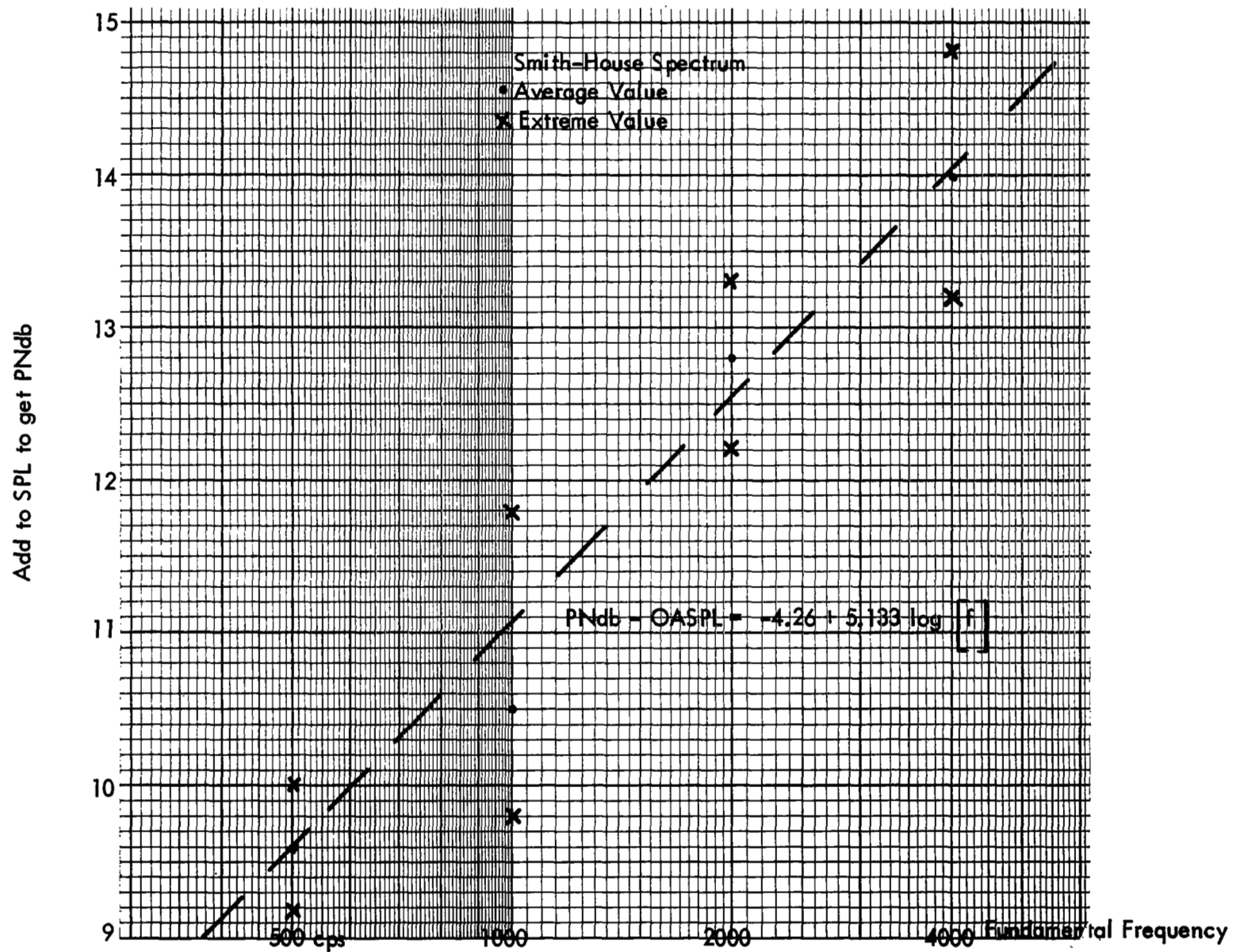
Fig. 20 - Compressor Noise PNdb - OASPL Difference
