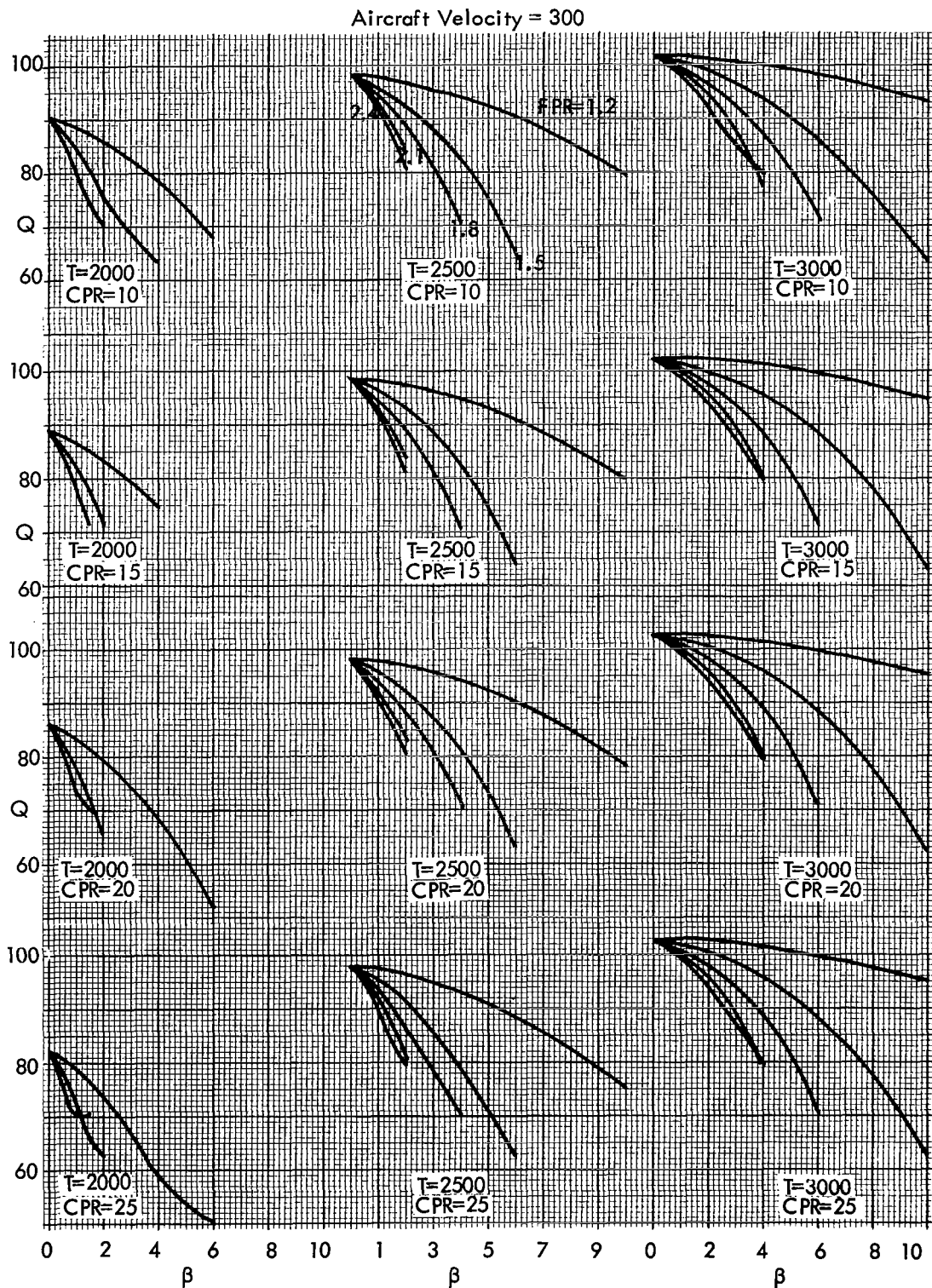
Figure 13c Q as a Function of B, FPR, T 4 , CPR for Various Aircraft Velocities
