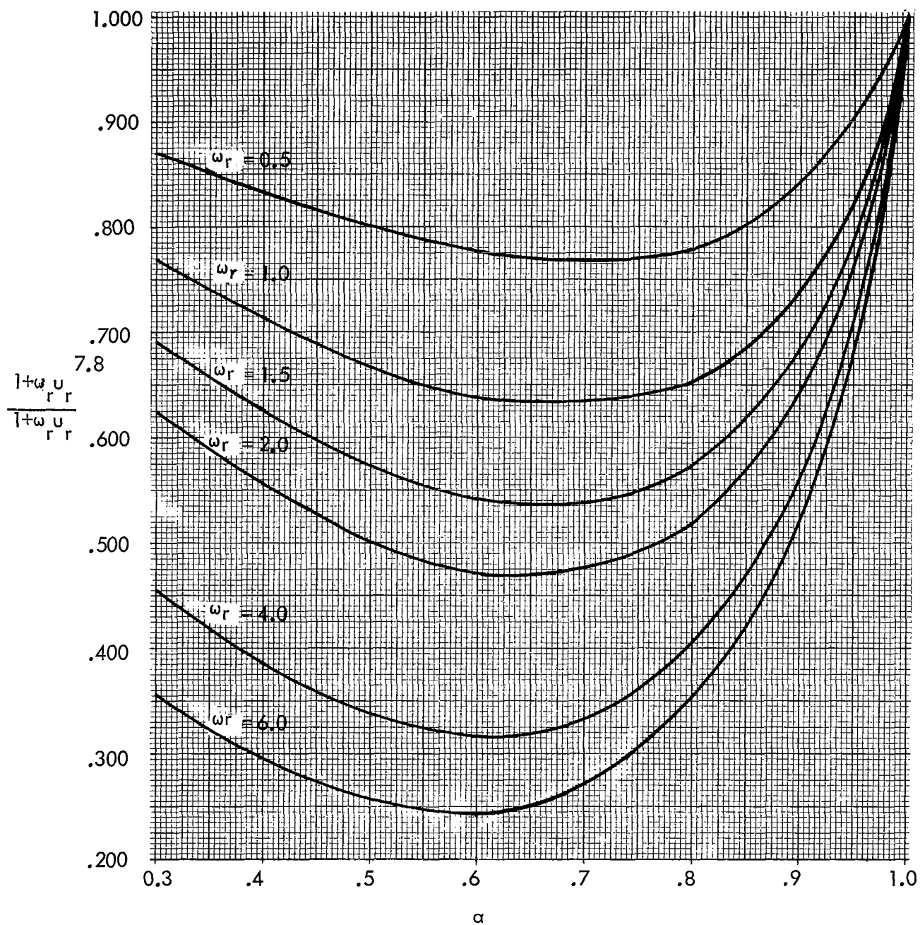
Figure 8 \frac{1 - \omega_r u_r}{1 - \omega_r u_r} Versus u_r and \omega_r
