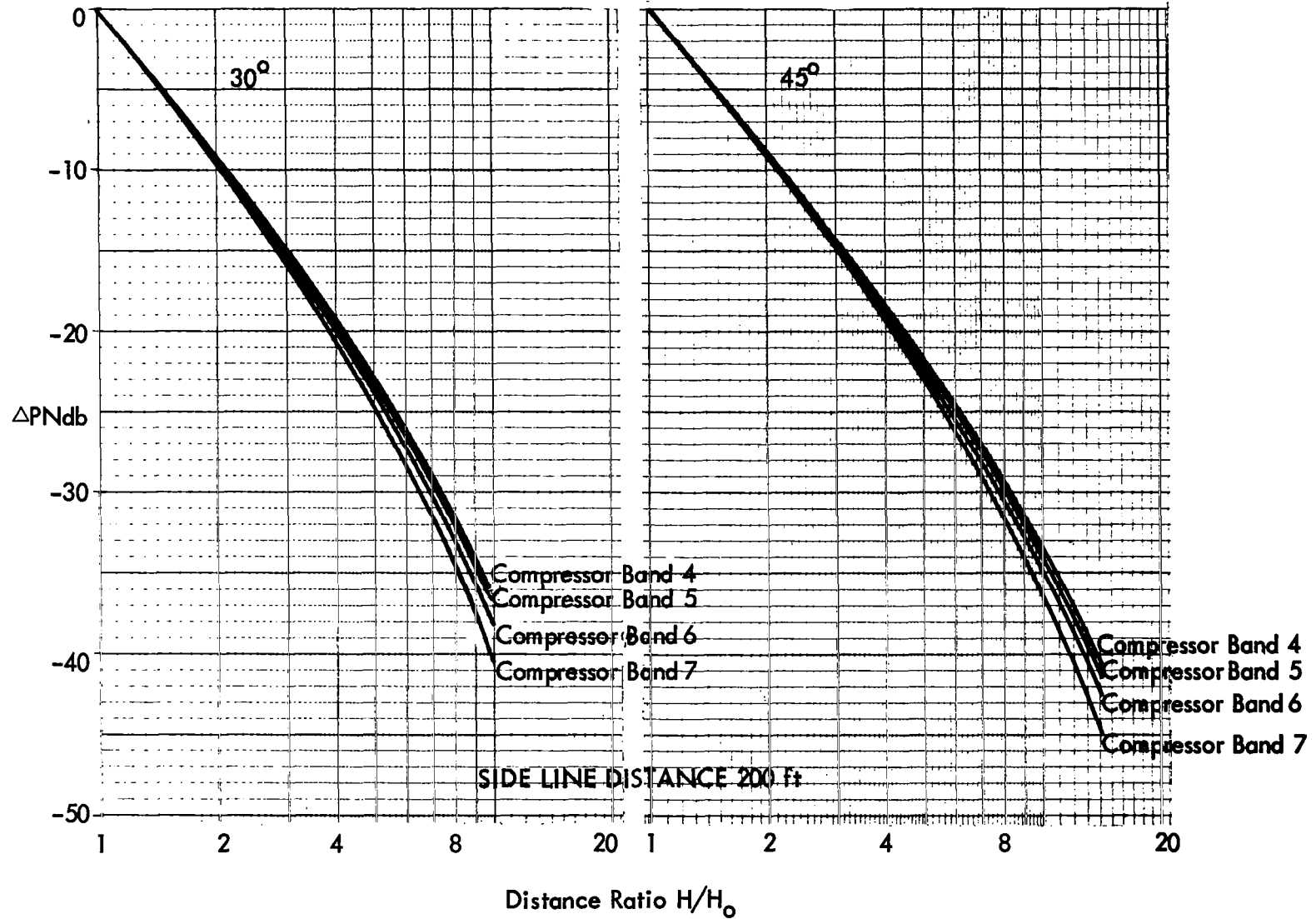
Fig. 33 - ON-Ground Combined Jet and Compressor \Delta P_{Ndb}
