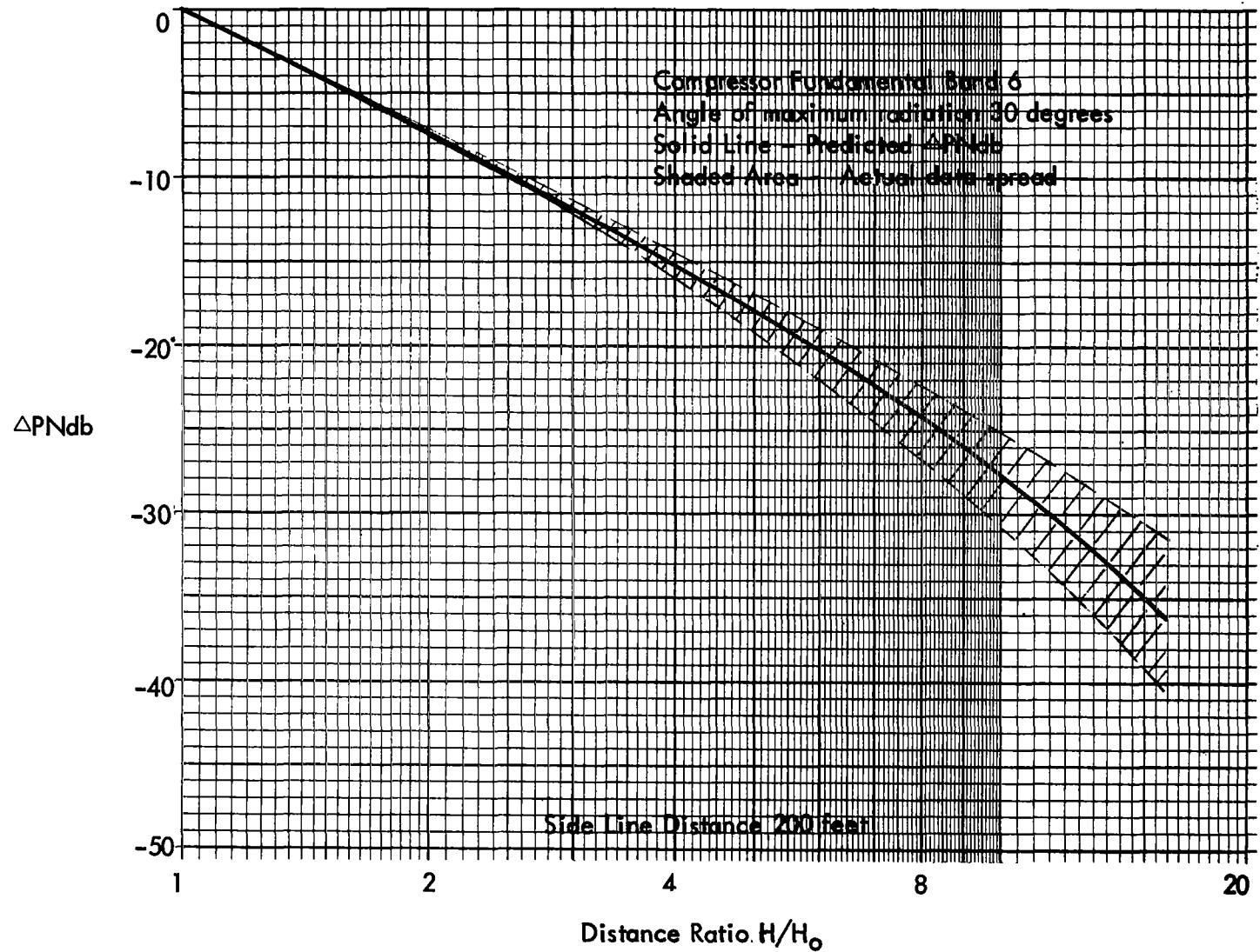
Fig. 37 - In-Flight Combined Jet and Compressor \Delta P_{Ndb} Accuracy
