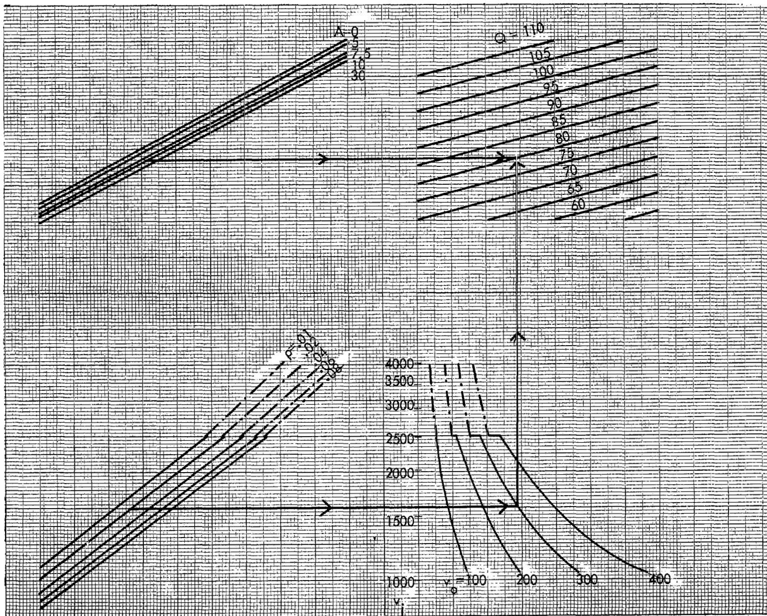
Figure 5 - Nomograph for Q
