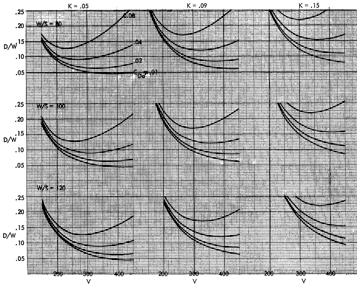
Figure 47 - D/W as a Function of K , C_{D0} , W/S , and V
