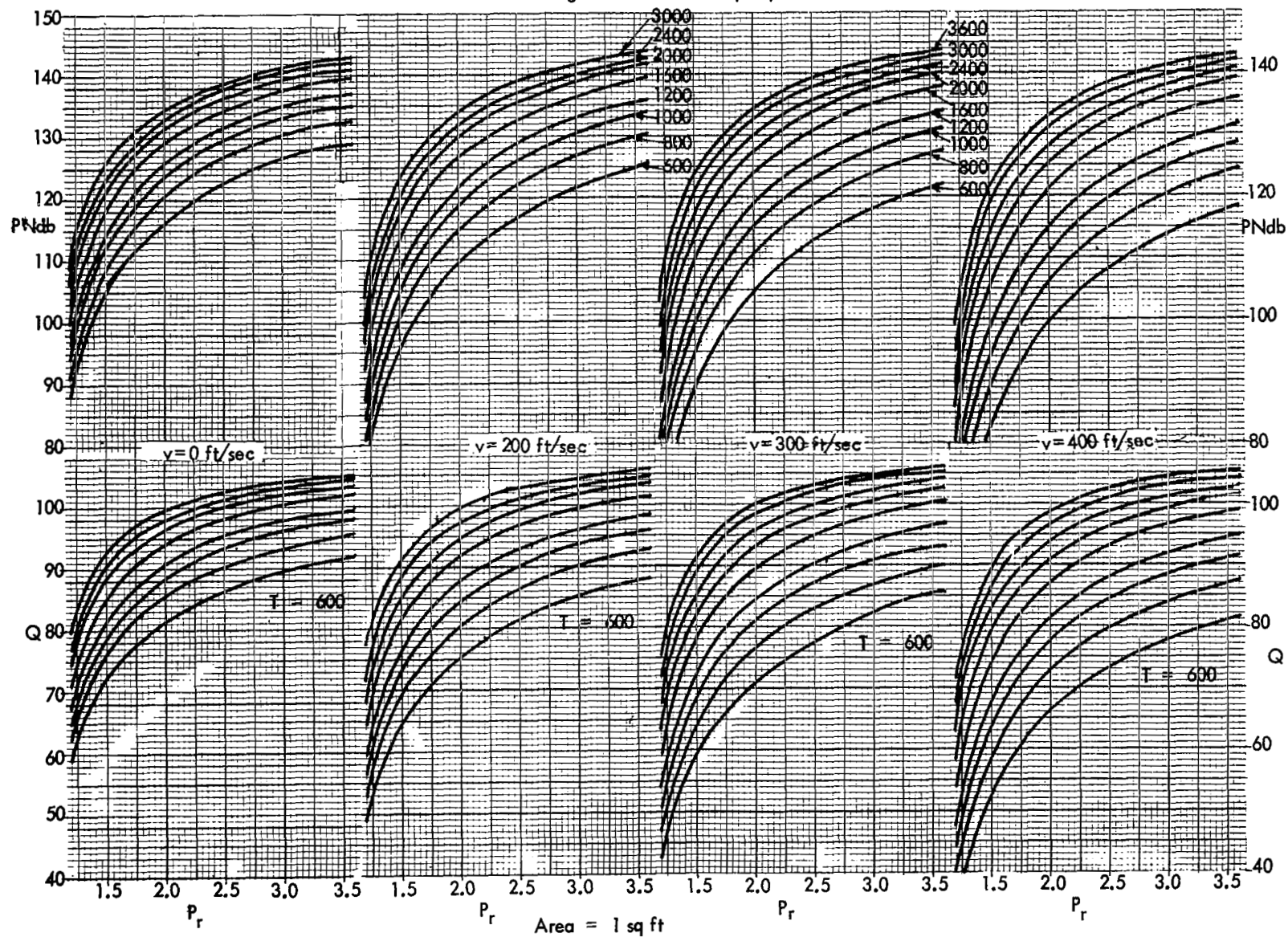
Figure 4a - PNdb_o as a Function of P_r , T_t , A , and V
