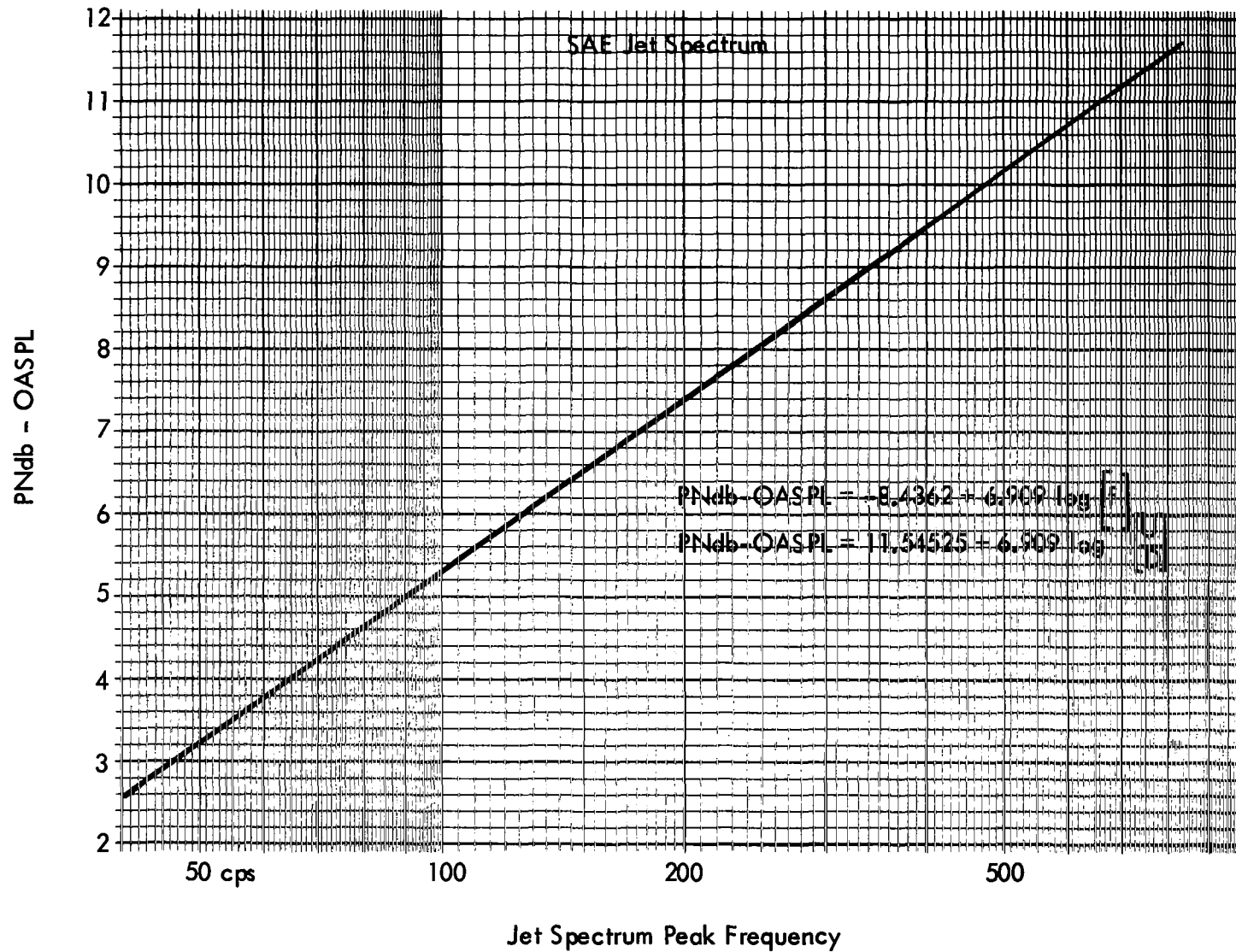
Fig. 19 - Jet Noise PNdb - OASPL Difference
