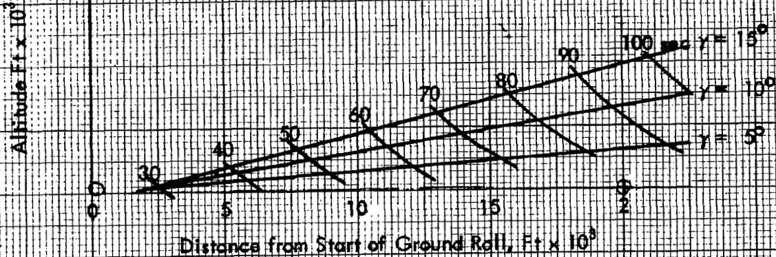
Figure 65a Flight Paths
