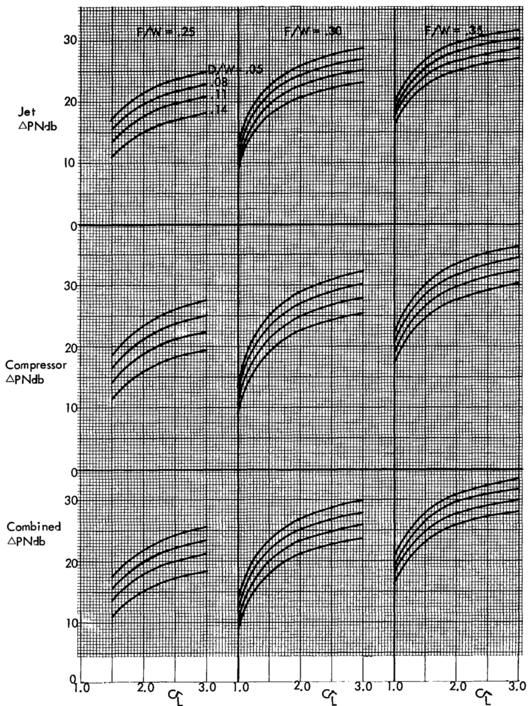
Figure 54 Three-Mile Point \Delta PN_{db} Versus C_L and D/W (For m=1 , n=1 , W_o/S=100 )
