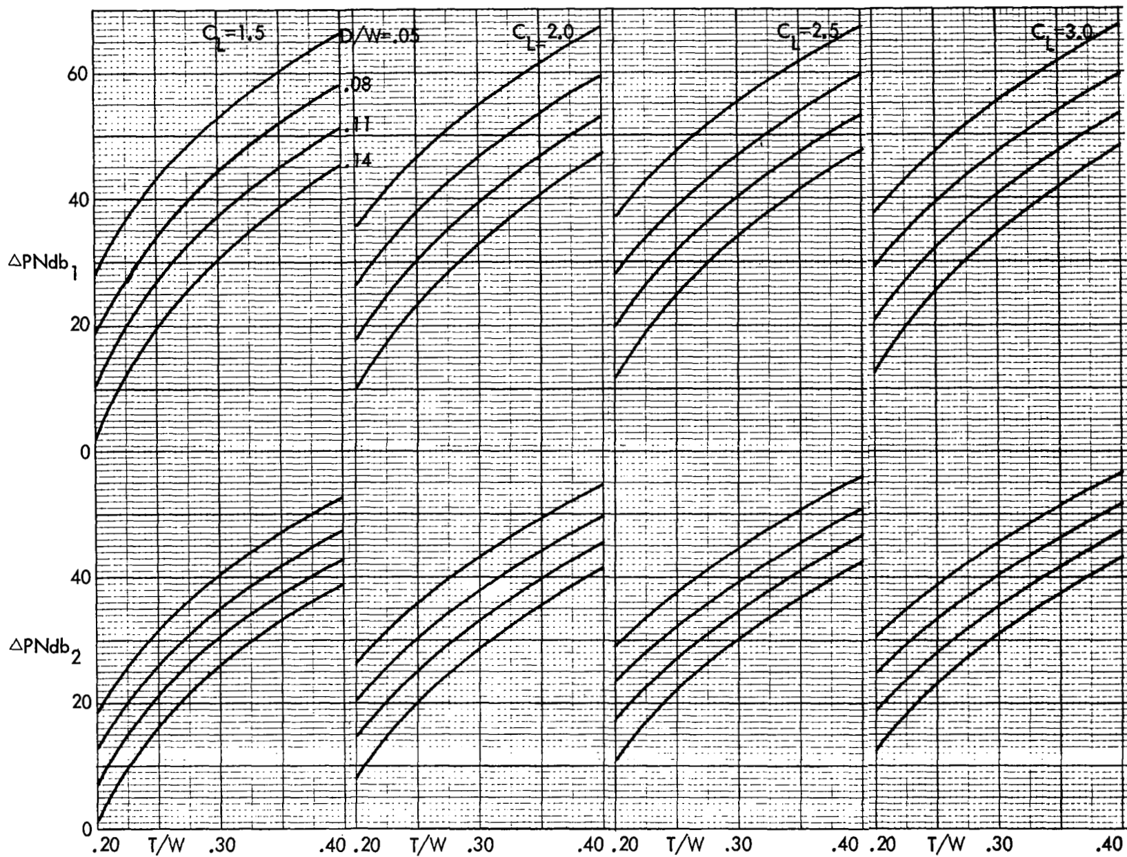
Figure 58 - \Delta PNdb as a Function of T/W , D/W , and C_L ( \overline{RC}=500 , W/S=100 )
