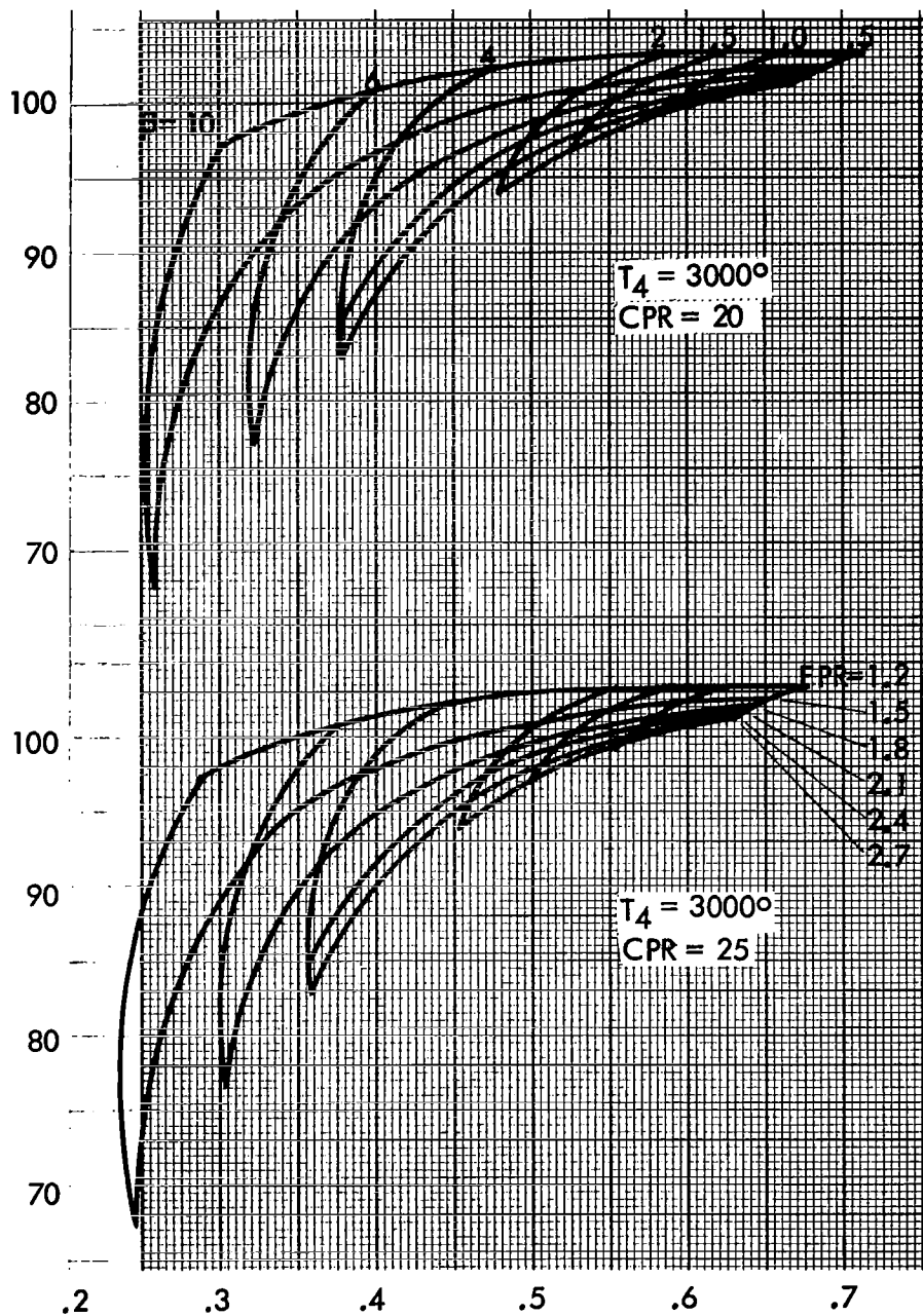
Figure 15b Q Versus SFC for Various CPR, FPR, B, and T 4
