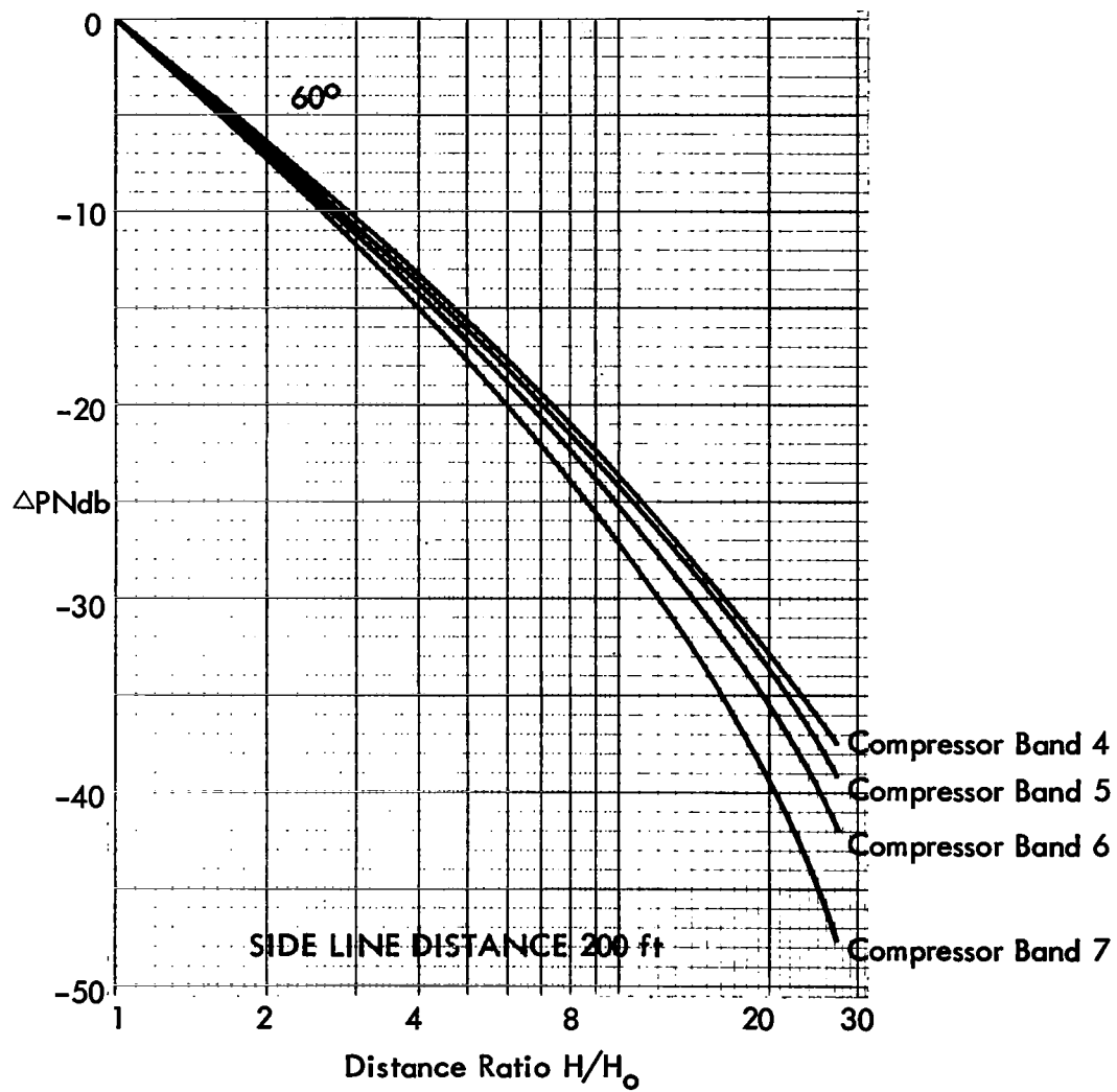
Fig. 30 - In-Flight Combined Jet and Compressor \Delta P_{Ndb}
