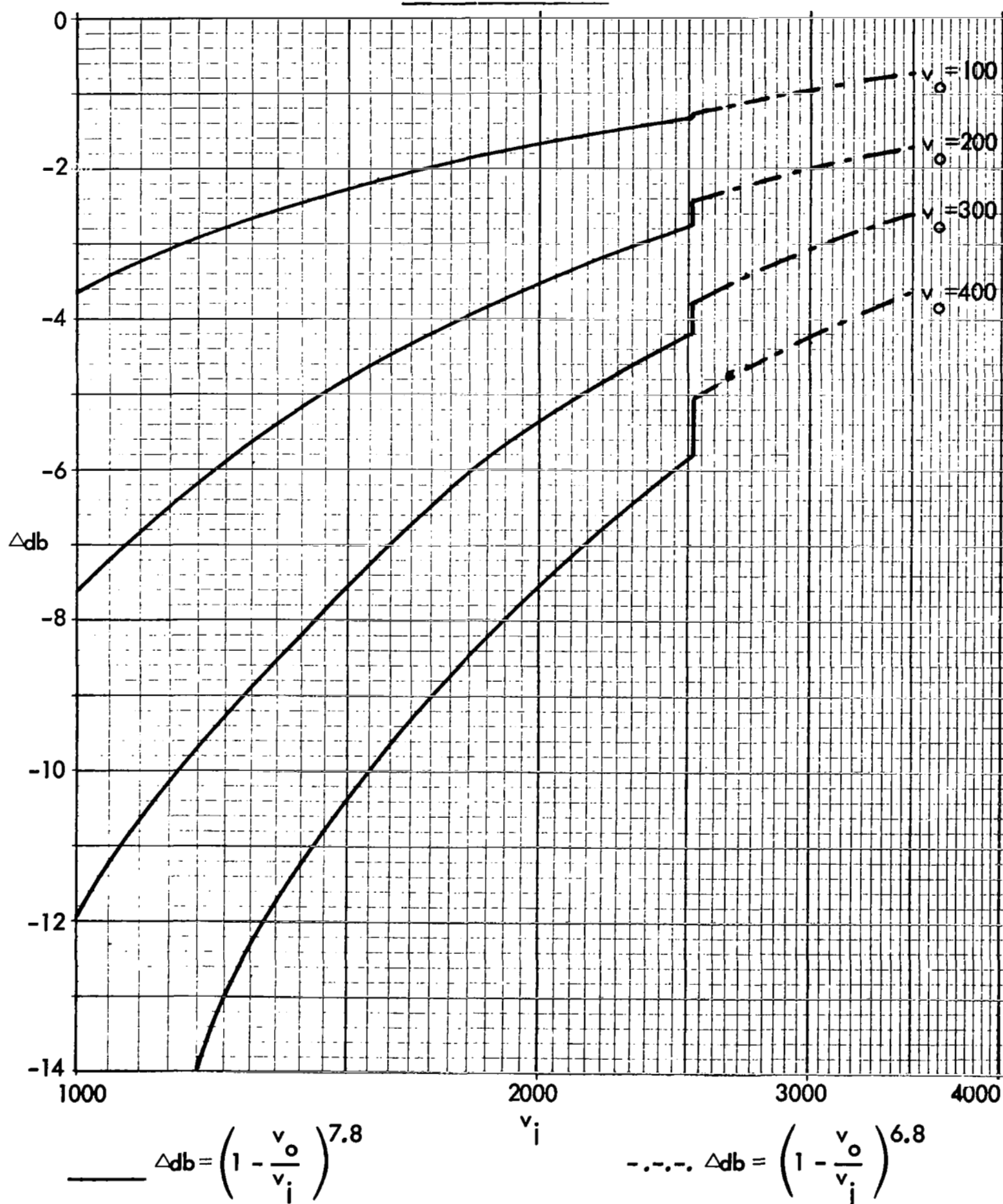
Figure 7 \Delta PNd_{\text{b}} Versus V_i
