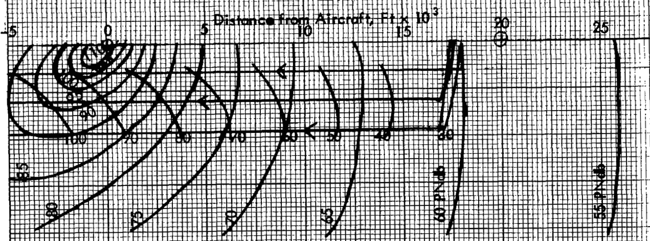
Figure 65b Noise Field Tracks
