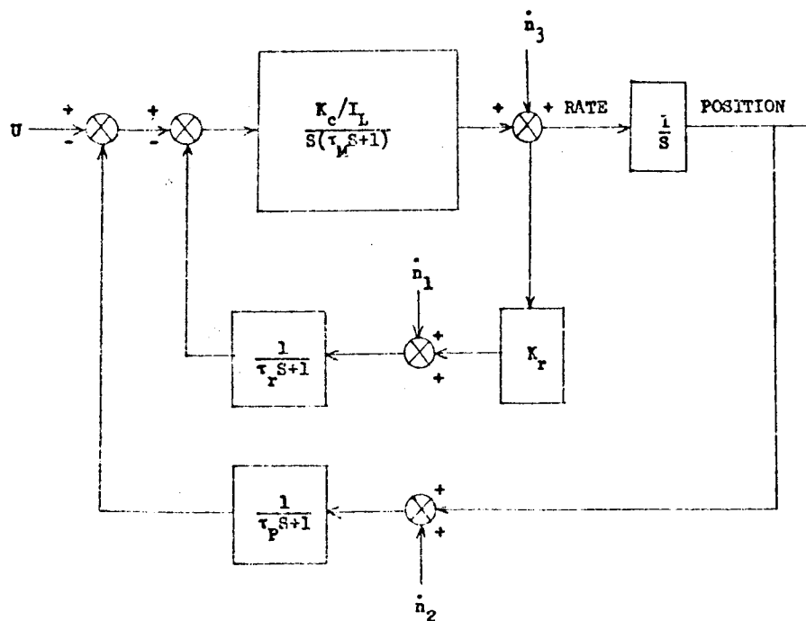
FIGURE 6-3. OPERATIONAL BLOCK DIAGRAM FOR SAMPLE SYSTEM
