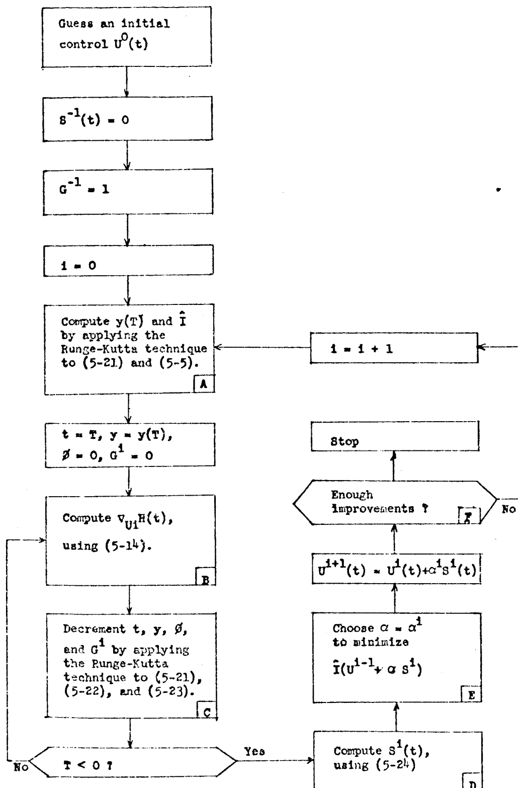
FIGURE 5-1. THE CONJUGATE GRADIENT ALGORITHM
