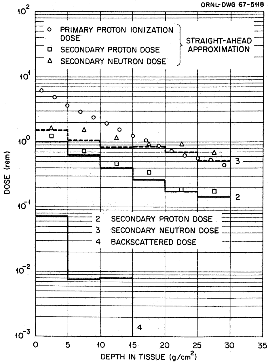
Fig. 10. Tissue Dose (rem) vs Depth; Flare Spectrum ( P_0 = 100 MV) Normally incident on 20 \text{ g}/\text{cm}^2 of Al Followed by Tissue.
