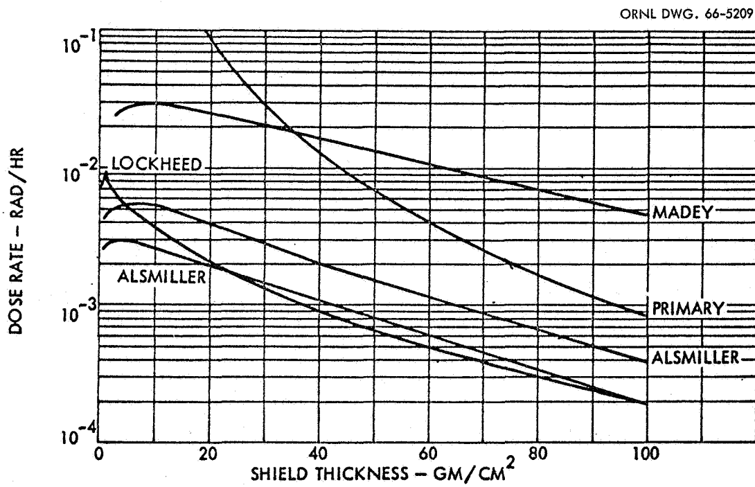
Fig. 14. Primary Proton and Gamma Dose Rate Aluminum Shield.
