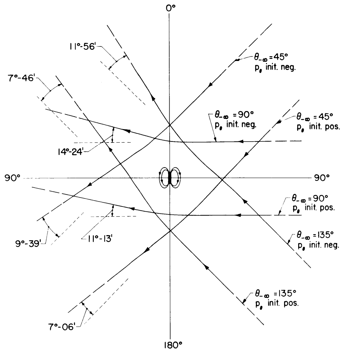
Figure 8. Comparative Meridian Plane Orbits With p_e Initially Positive And Negative.
