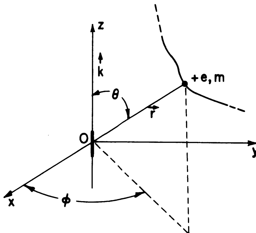
FIGURE 1. POSITION OF THE ION IN SPHERICAL COORDINATES.
