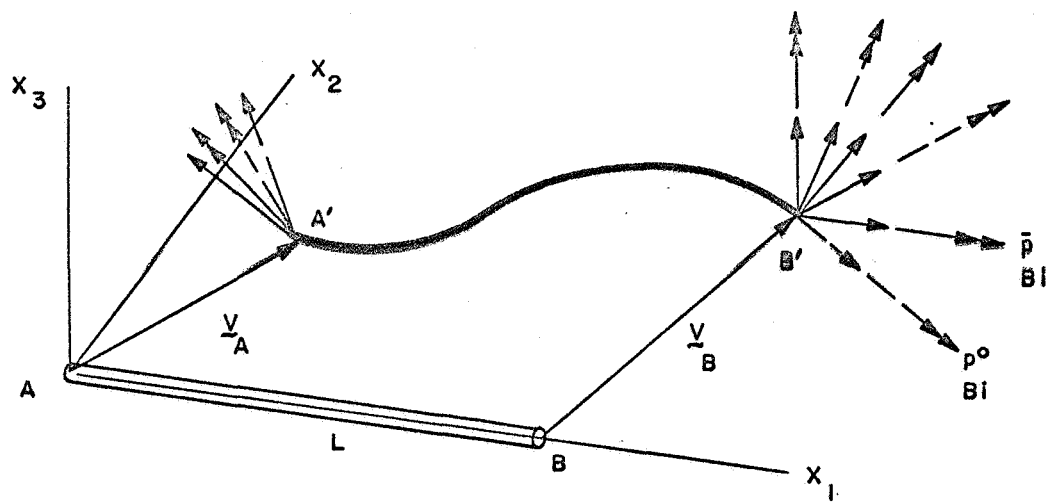
FIG. 6 NODE FORCES ON DEFORMED BAR
