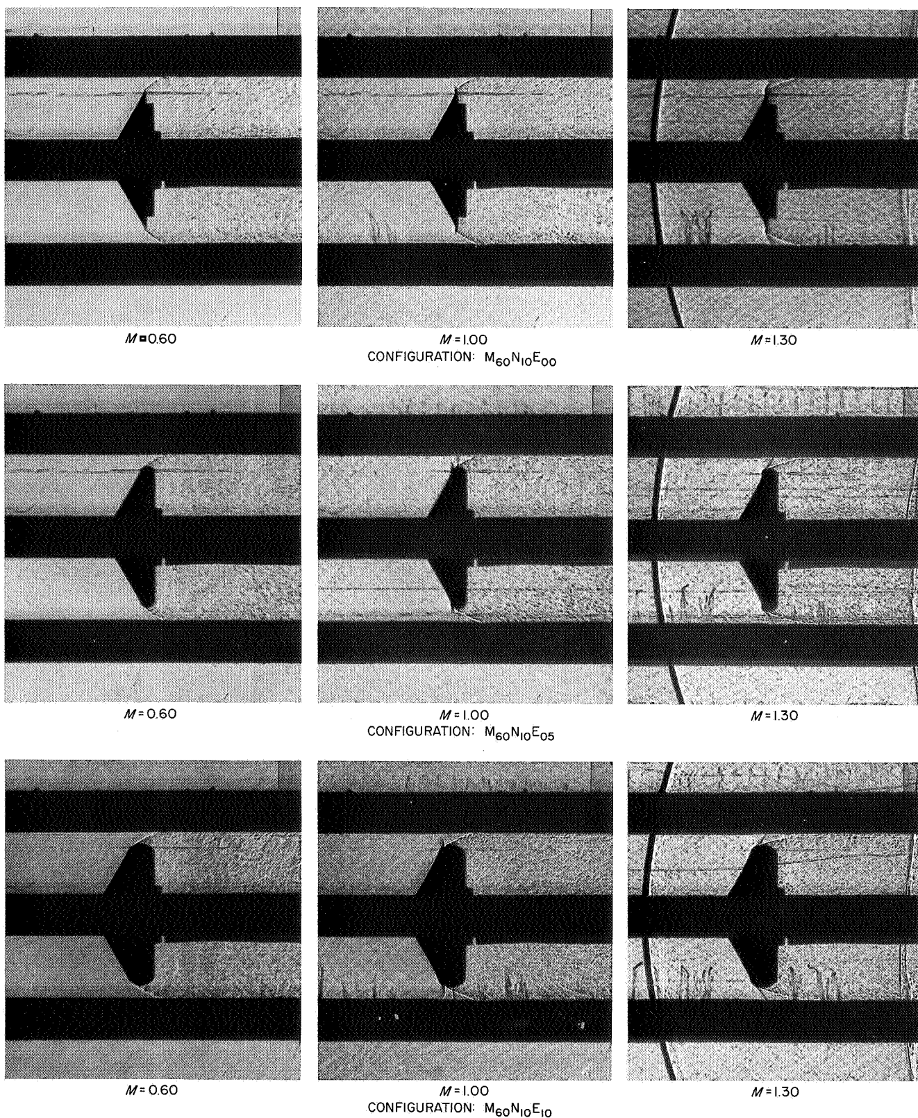
Fig. 4. Shadowgraph photographs at M = 0.60, 1.00 , and 1.30 , \alpha = 0 deg
