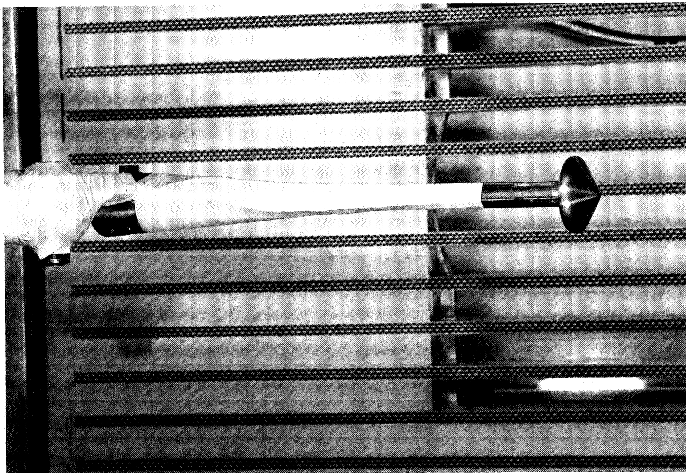
Fig. 2. Typical model installation in ARC 2 × 2-ft transonic wind tunnel
