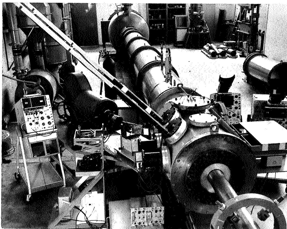
Figure 2 Target Chamber Set-up, with Continuous-Writing Streak Camera in Position
