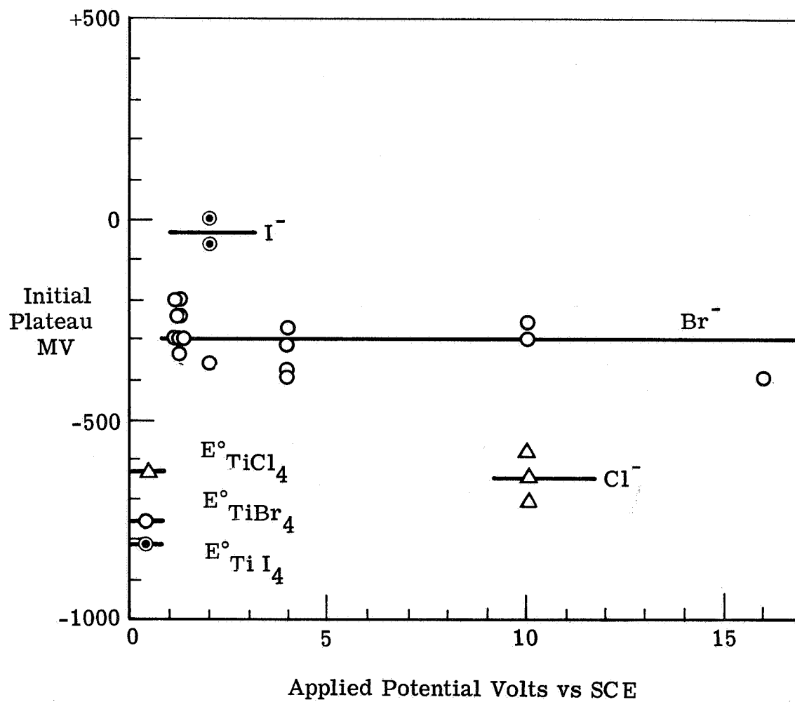
Fig. 2. Initial Open-Circuit Potential During Pitting of Titanium in 0.6 M Halide Solutions.
