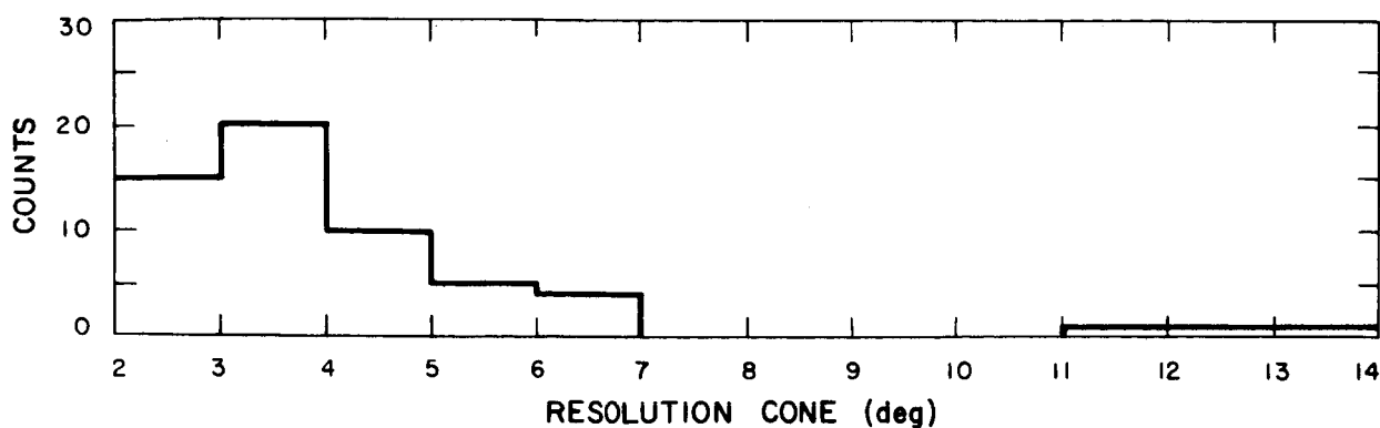
Figure 13a. Events within 20^\circ RA and 20^\circ declination of Crab Nebula vs. resolution cone angle.
