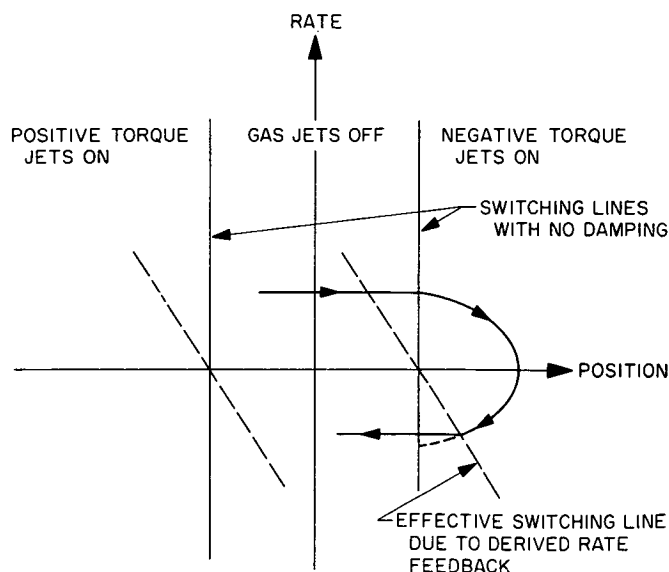
Fig. 8. Derived-rate damping in the phase plane
