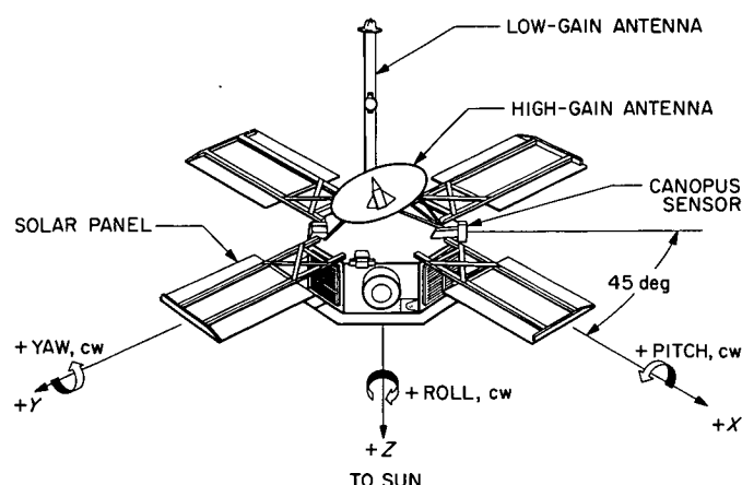
Fig. 2. Spacecraft coordinate system
