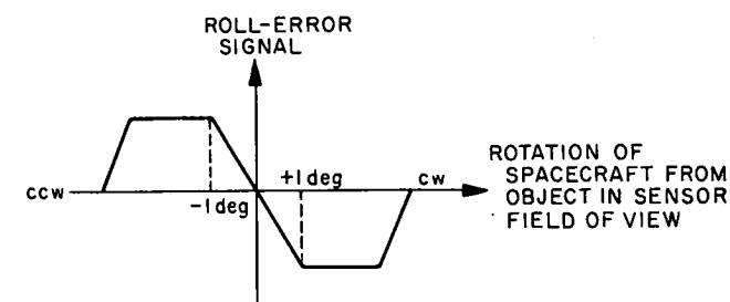
Fig. 6. Roll-error signal
