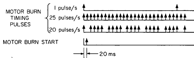
Fig. 12. Phasing of motor burn timing signal
