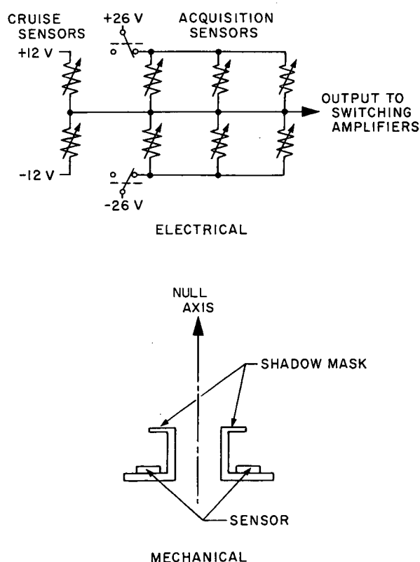
Fig. 4. Sun sensors
