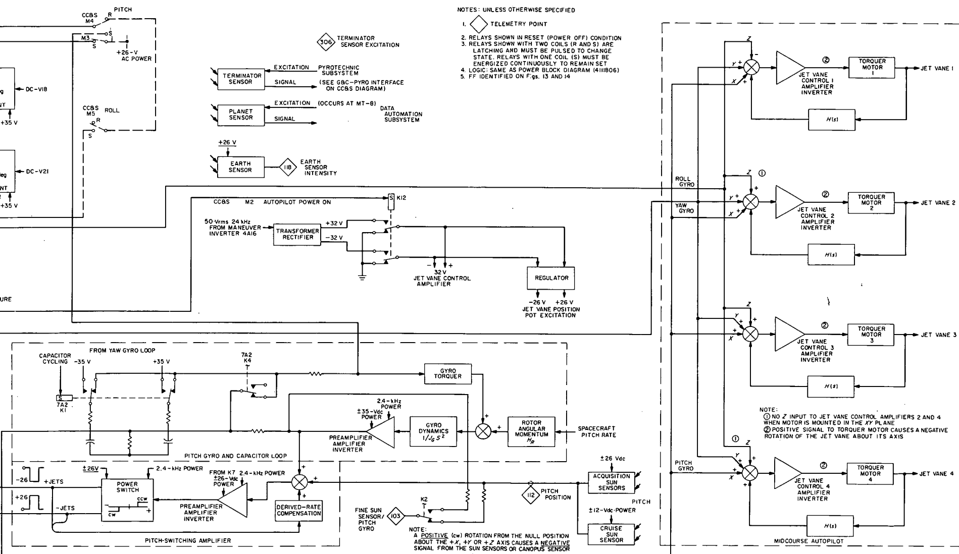
Fig. 15. G&C block diagram: attitude control subsystem
