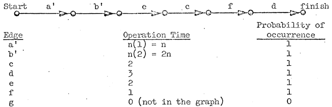
Figure 5 Single Path Program Graph of the Function Y = A \sum_{i=1}^n X_i + B
