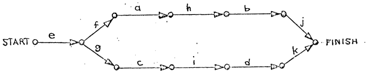
Figure 7 Program Graph for a Probabilistic Function of Computation
