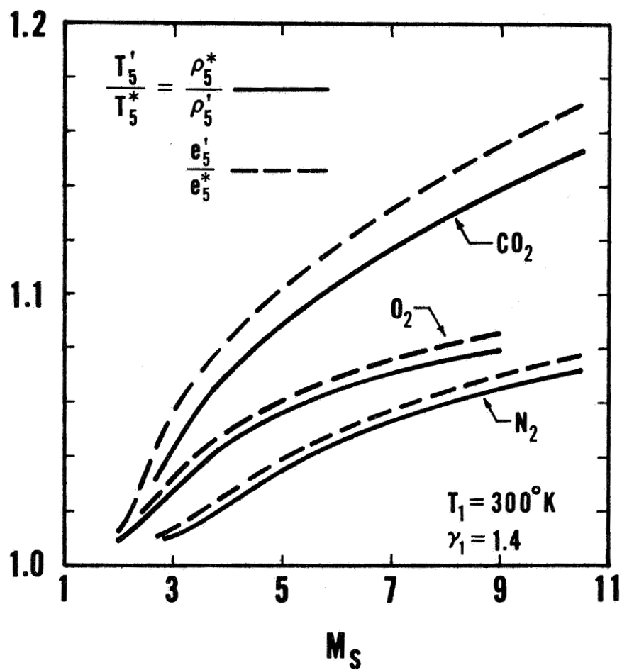
Fig. 48. Simple model predictions for final end-wall states in vibrationally relaxing \text{CO}_2 , \text{O}_2 and \text{N}_2 .
