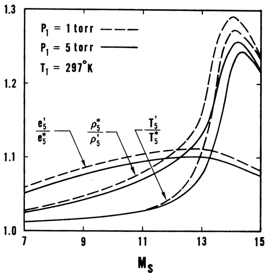
Fig. 49. Simple model predictions for final end-wall states in chemically relaxing \text{O}_2 .
