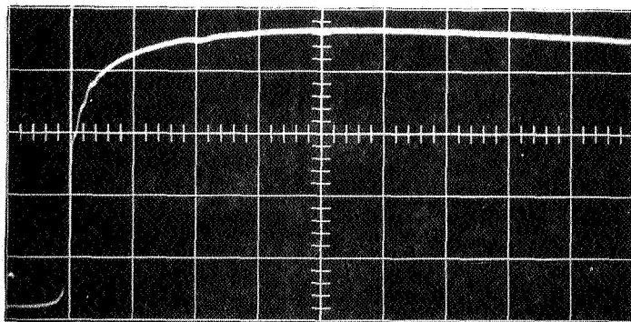
b) V_s = 7.1 \text{ km/sec} ; P_1 = .53 \text{ torr} ; Sweep Speed = 1 \text{ } \mu\text{sec/div.}
