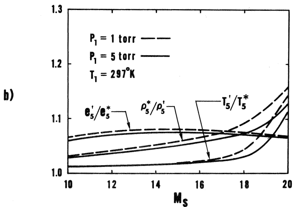
Fig. 44. Final end-wall states in chemically relaxing \text{O}_2 and \text{N}_2 : a) \text{O}_2 ; b) \text{N}_2 .
