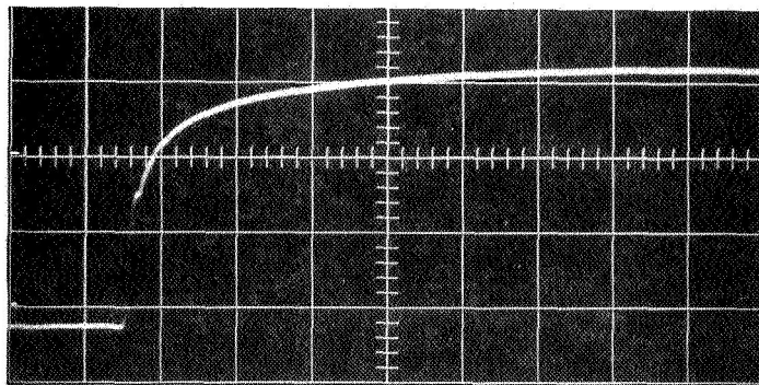
a) V_s = 6.0 \text{ km/sec} ; P_1 = .86 \text{ torr} ; Sweep Speed = 1 \text{ } \mu\text{sec/div.}
