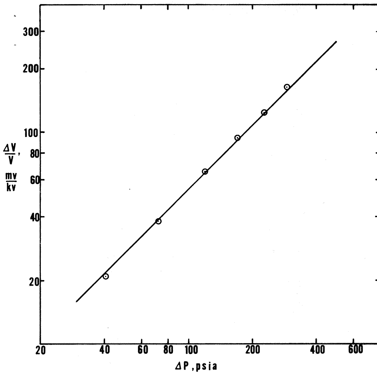
Fig. 17. Pressure-gauge calibration curve. Gauge sensitivity = 0.53 mv/psi-kv.
