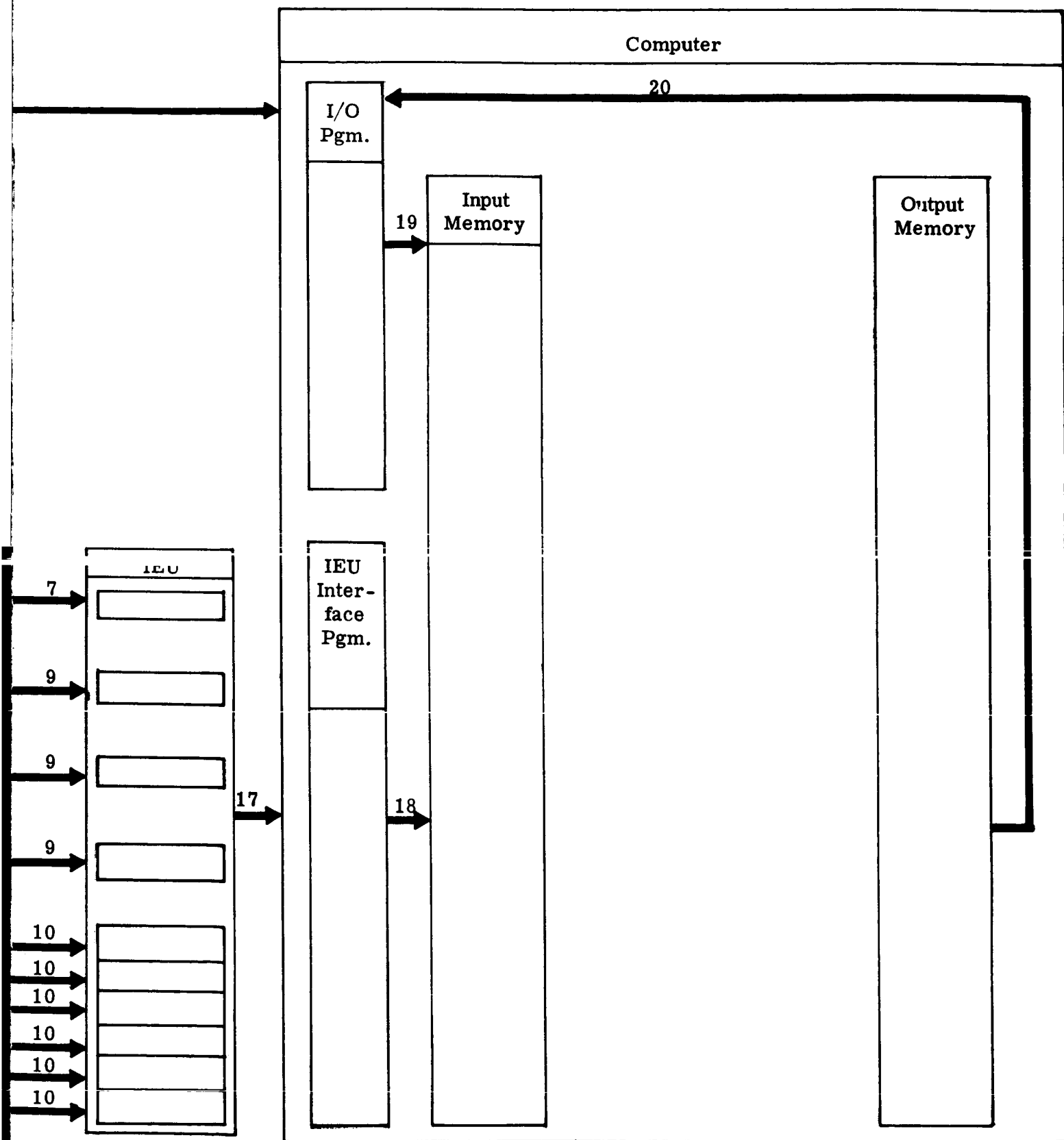
Figure 3-6. Laboratory Flow Diagram System Data Interfaces
