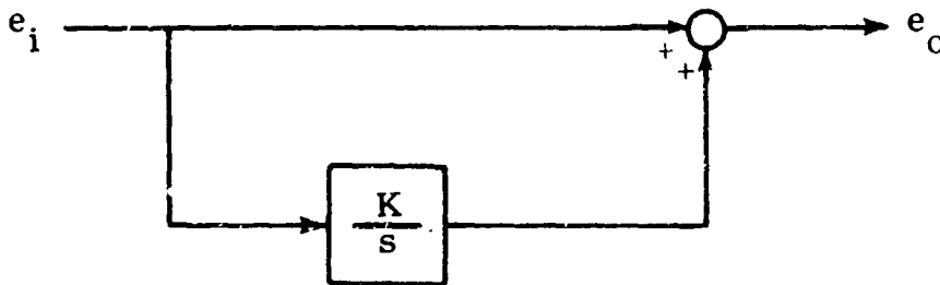
Figure 3.1-7 Block Diagram for Integral Bypass Compensation
