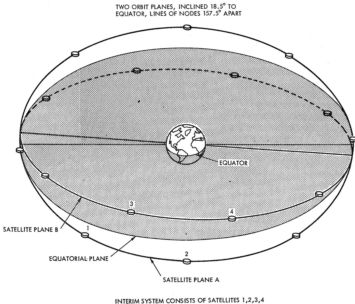
Figure 1. Satellite Geometry
