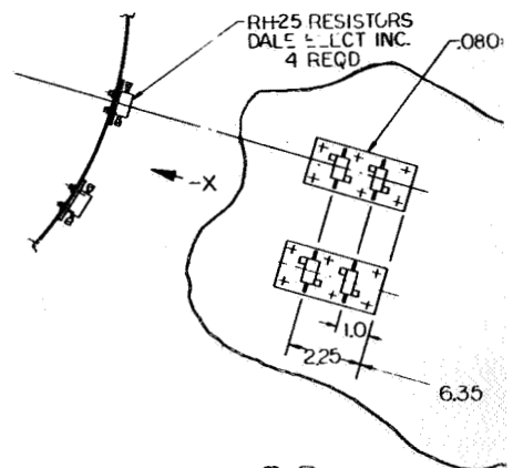
VIEW D-D
