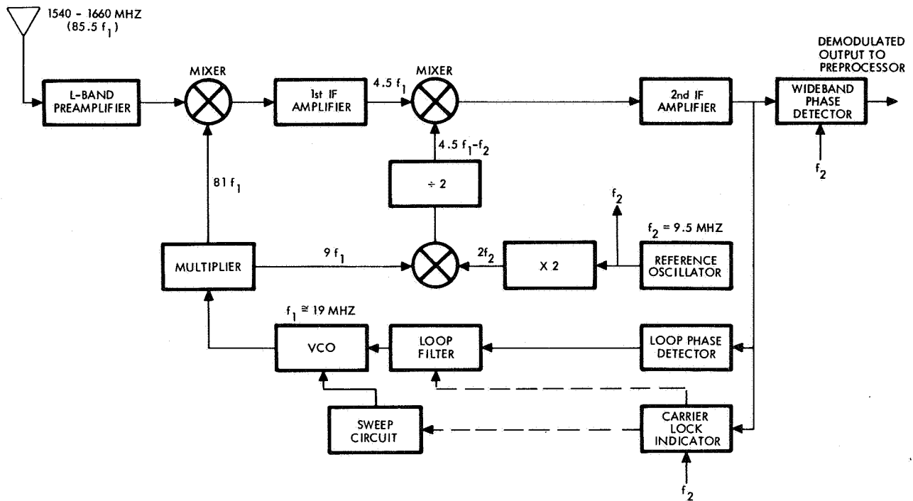
Figure 22. Simplified Block Diagram of NAVSTAR CW Receiver
