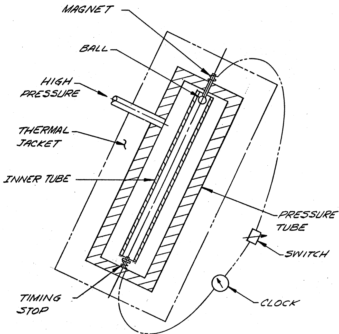
DIAGRAM OF PRINCIPLE OF RUSKA HIGH PRESSURE VISCOMETER
