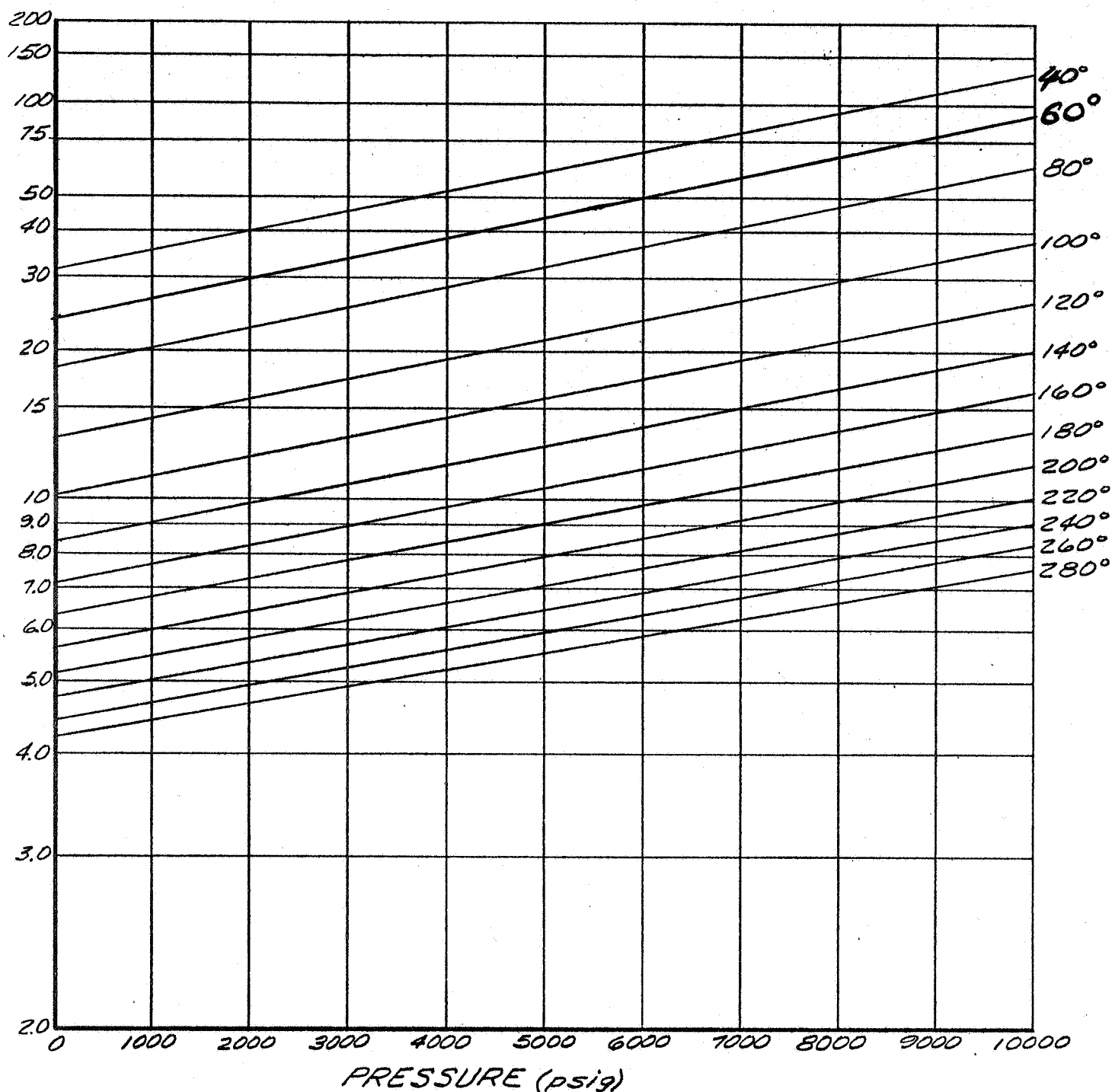
VISCOSECITY-PRESSURE-TEMPERATURE, MIL 5606 CALCULATED DATA
